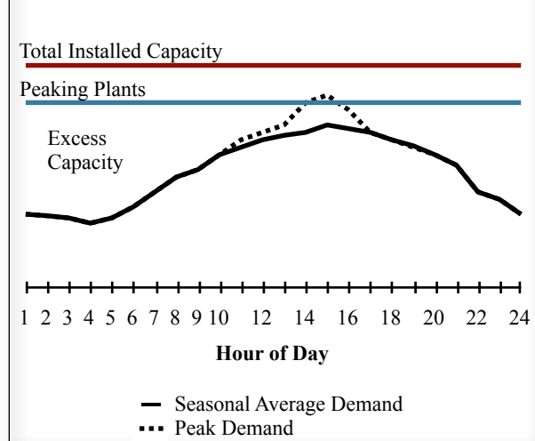
Figure 13: Load Shape for 1 Day During Peak Season
