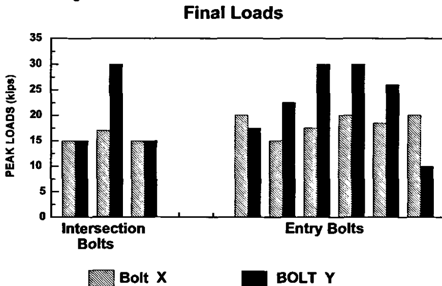
Final loads measured on the instrumented bolts at Mine A. Bolts are paired by location (i.e., the first pair shows the right-hand intersection "X" bolt compared to the right-hand intersection "Y" bolt.
