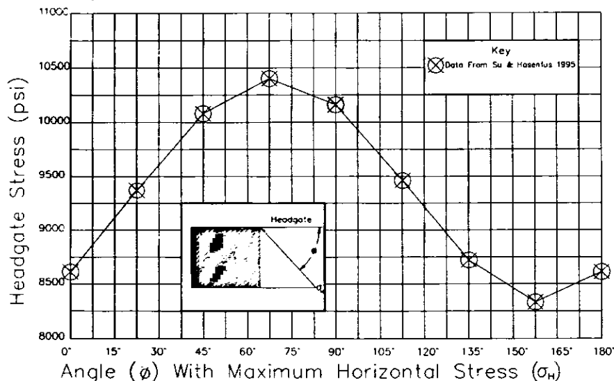
Affect of panel orientation on horizontal stresses (Mises shear stresses) calculated by finite element modeling (after Su and Hasenfus, 1995).
