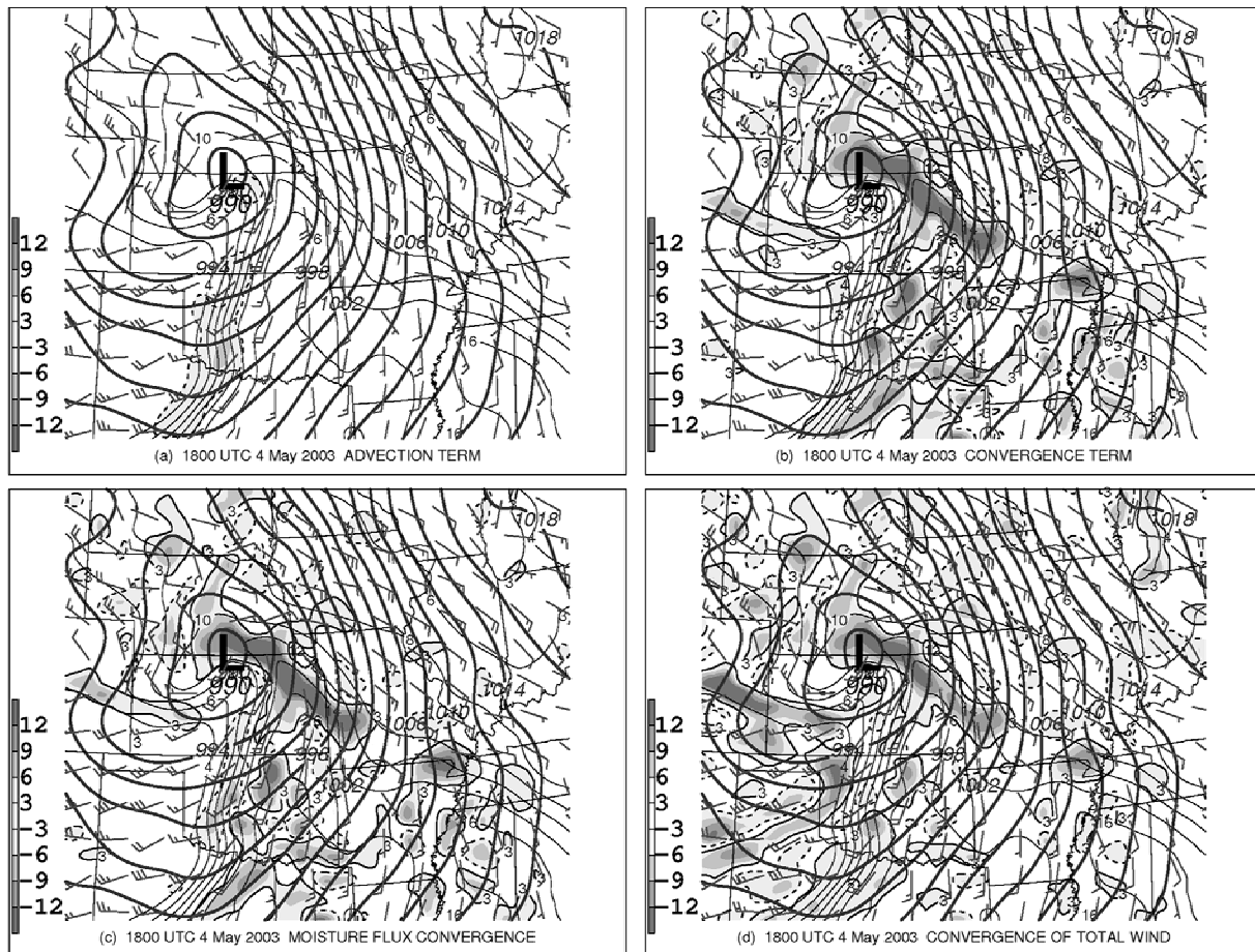
Fig. 1 Surface objective analysis valid at 1800 UTC on 4 May 2003. Sea-level pressure (thick solid lines every 2 mb), specific humidity (thin solid lines every 2 \text{g kg}^{-1} ). Shaded regions represent (a) the advection term in MFC expression ( 10^{-4} \text{ g kg}^{-1} \text{ s}^{-1} ), where positive values represent moist advection, (b) the convergence term in MFC expression ( 10^{-4} \text{ g kg}^{-1} \text{ s}^{-1} ), where positive values represent convergence, (c) the total moisture flux convergence ( 10^{-4} \text{ g kg}^{-1} \text{ s}^{-1} ), where positive values represent positive MFC, and (d) the horizontal mass convergence of the total wind ( 10^{-5} \text{ s}^{-1} ), where negative values represent horizontal mass divergence. Thin dashed lines (thin solid lines) delineate negative (positive) values associated with shaded regions for
