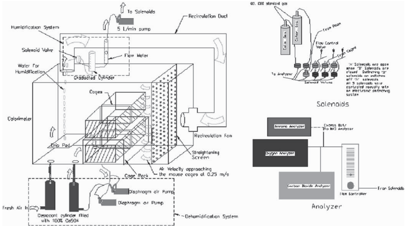
Figure 3 Experimental apparatus for mass generation rates of ammonia in mouse cages at low and high relative humidities.
