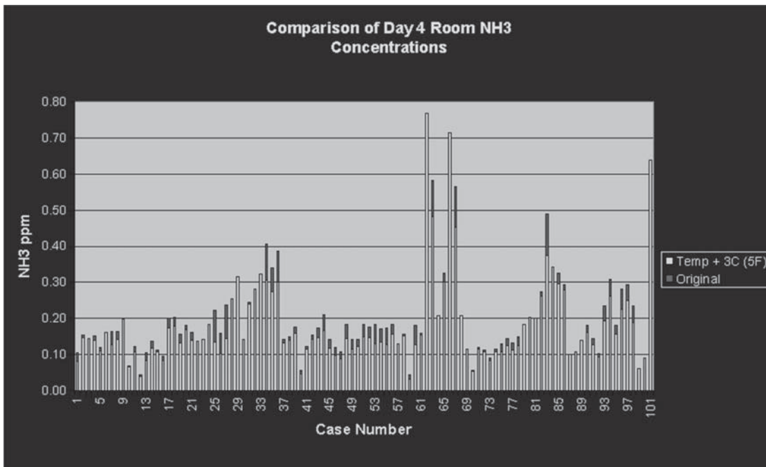
Figure 11 Comparison of room day 4 \text{NH}_3 concentrations on increased supply air discharge temperature (cases taken from Memarzadeh [1986]).
