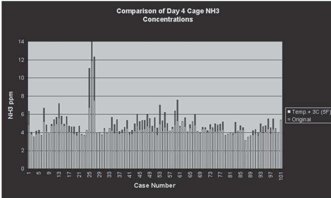
Figure 10 Comparison of cage day 4 \text{NH}_3 concentrations on increased supply air discharge temperature (cases taken from Memarzadeh [1986]).
