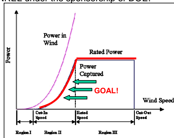
Figure 18. Wind Turbine Power Curve
