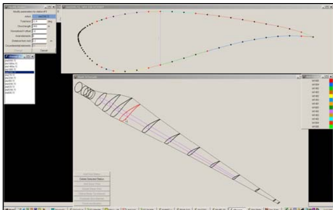
Figure 21. NuMAD - Structural Flexibility/Expandability Analysis
