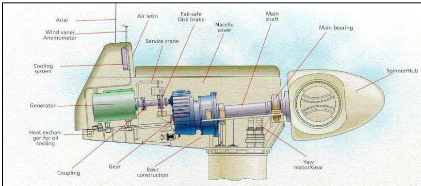
Figure 4. Typical Wind Turbine Architecture
