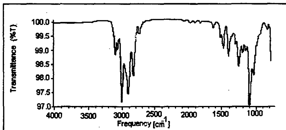
FIG. 2A —The infrared spectrum obtained in the process of the urine extract GC/FTIR analysis.
