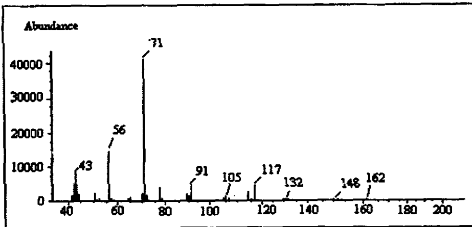
FIG. 3A —The mass spectrum obtained after the GC/MS analysis of the urine extract.
