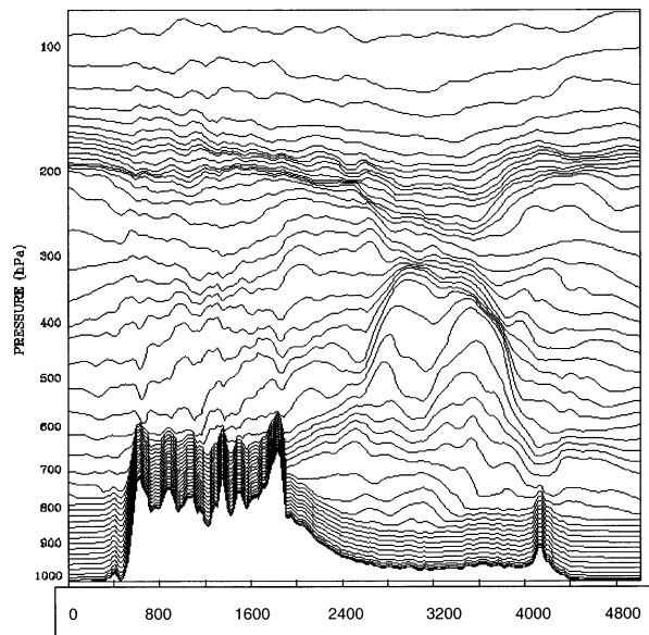
FIG. 6. Vertical cross section of RUC hybrid isentropic–sigma coordinate levels for 1800 UTC 14 Jan 2002. The cross section is oriented approximately west–east through California on the left-hand side, Colorado, and the Appalachian Mountains.
