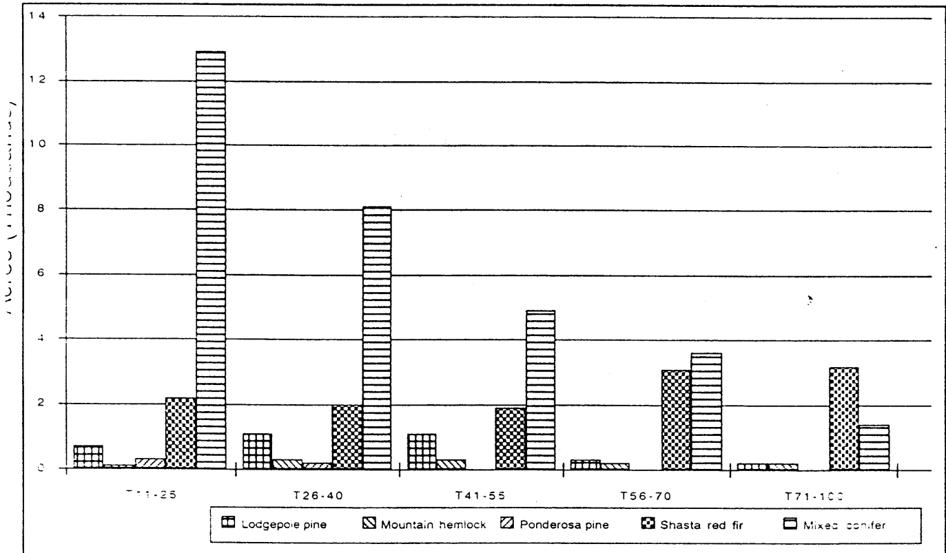
Figure 15. Spencer Creek Watershed - 1994 Canopy Closure, Trees Only
