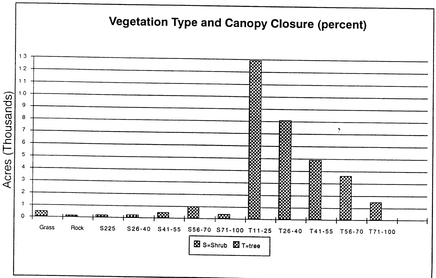
Figure 4. Spencer Creek Watershed - 1994 Mixed Conifer Zone Canopy Closure
