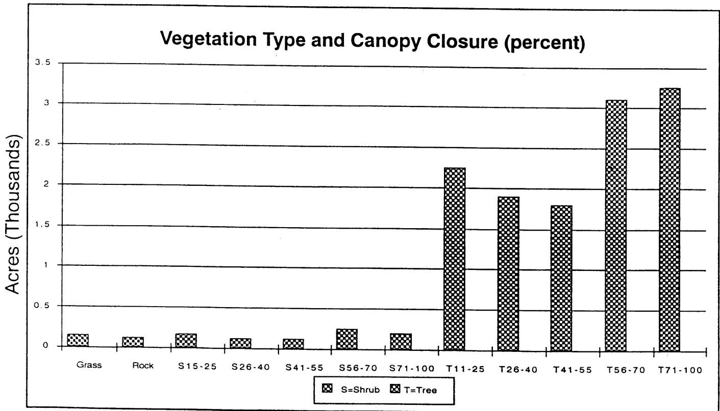
Figure 6. Spencer Creek Watershed - 1994 Shasta Red Fir Zone Canopy Closure
