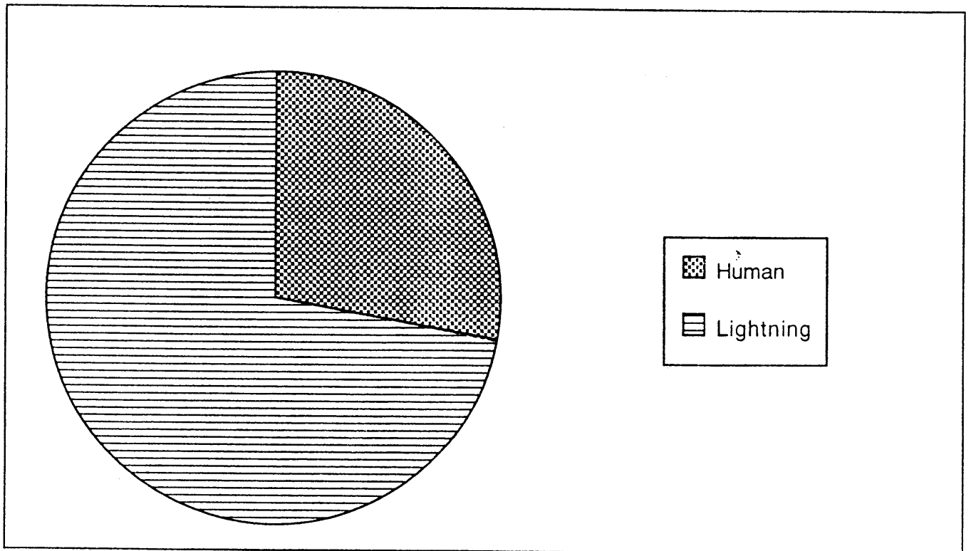
Figure 9. Spencer Creek - 1961-1994 Fires - Human Caused Versus Lightning Caused (percent of total fires)
