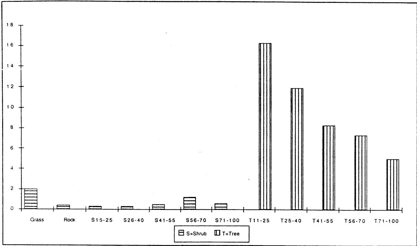
Figure 14. Spencer Creek Watershed - 1994 Canopy Closure for the Entire Watershed, All Vegetation Types
