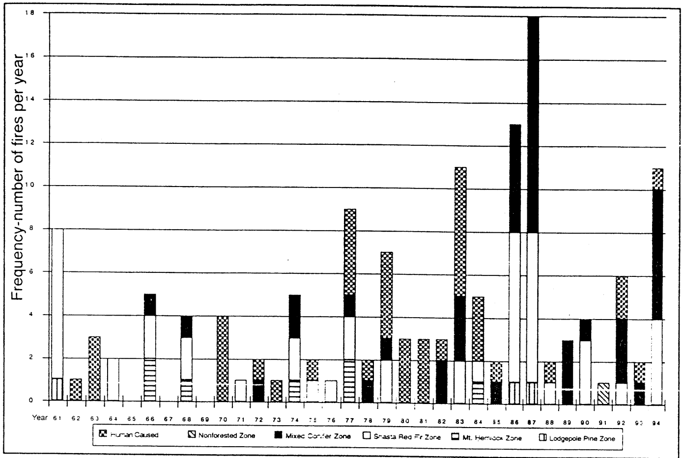
Figure 8. Spencer Creek - Lightning Fires By Zone and Human Caused Fires (for all lands)
