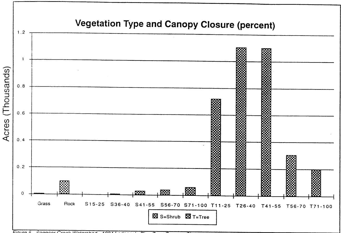
Figure 5. Spencer Creek Watershed - 1994 Lodgepole Pine Zone Canopy Closure
