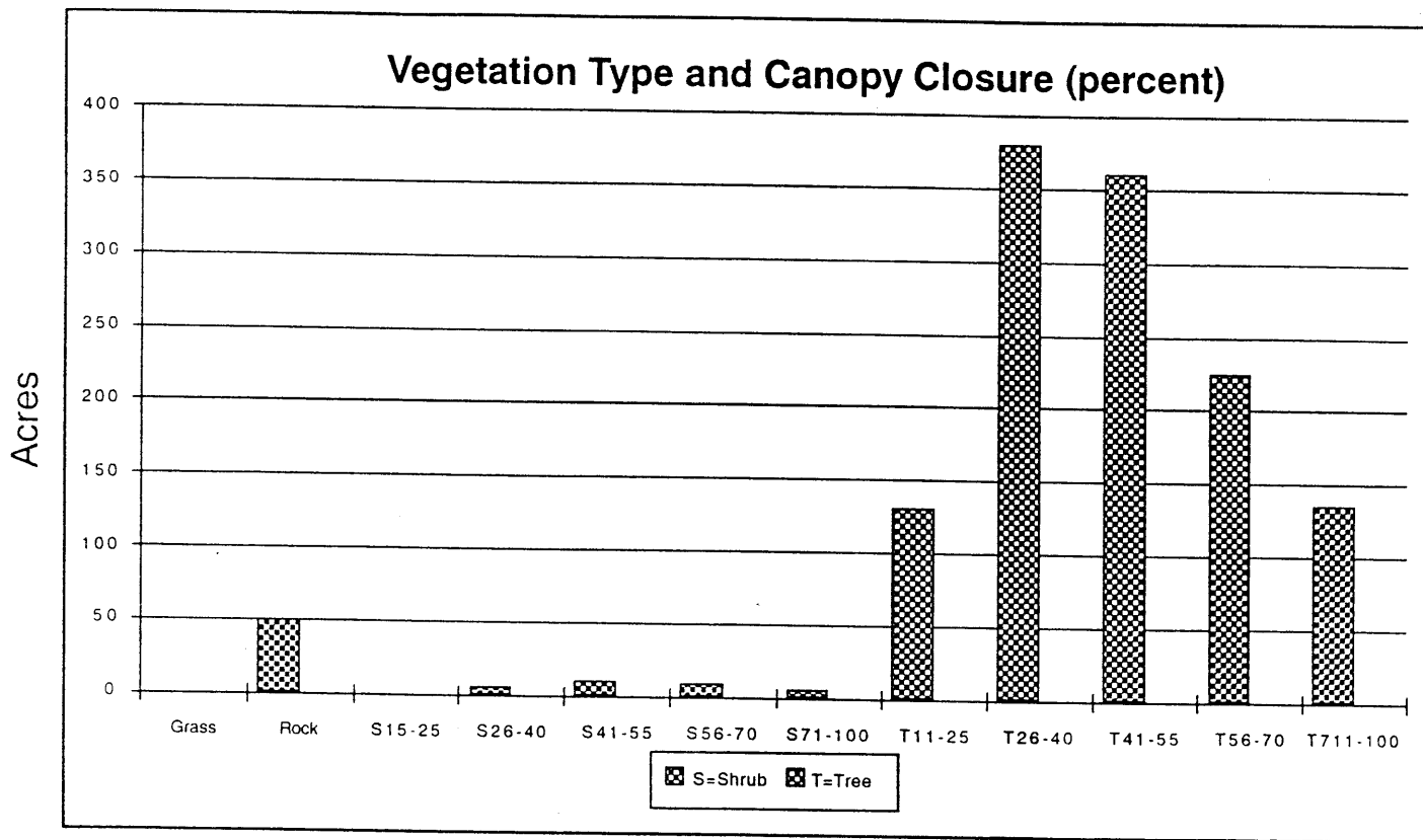
Figure 7. Spencer Creek Watershed - 1994 Mountain Hemlock Zone Canopy Closure
