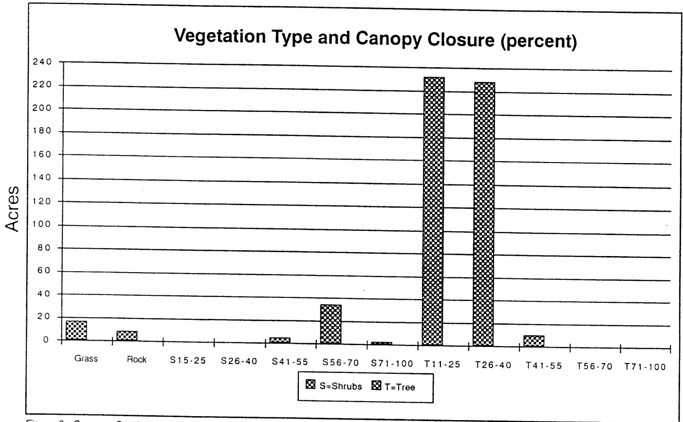
Figure 3. Spencer Creek Watershed - 1994 Ponderosa Pine Zone Canopy Closure
