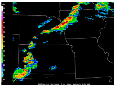
(a) Observed hourly maximum base-reflectivity
