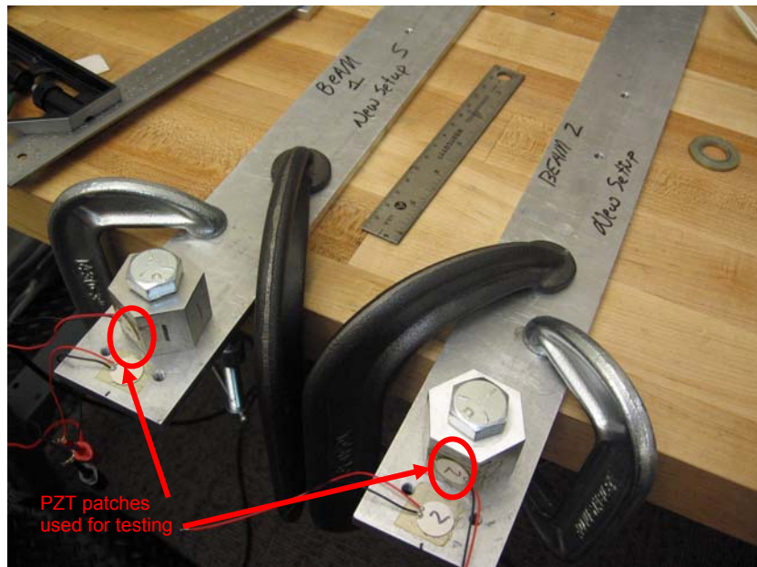
Figure 6: Experimental setup with PZT enhanced washers.
