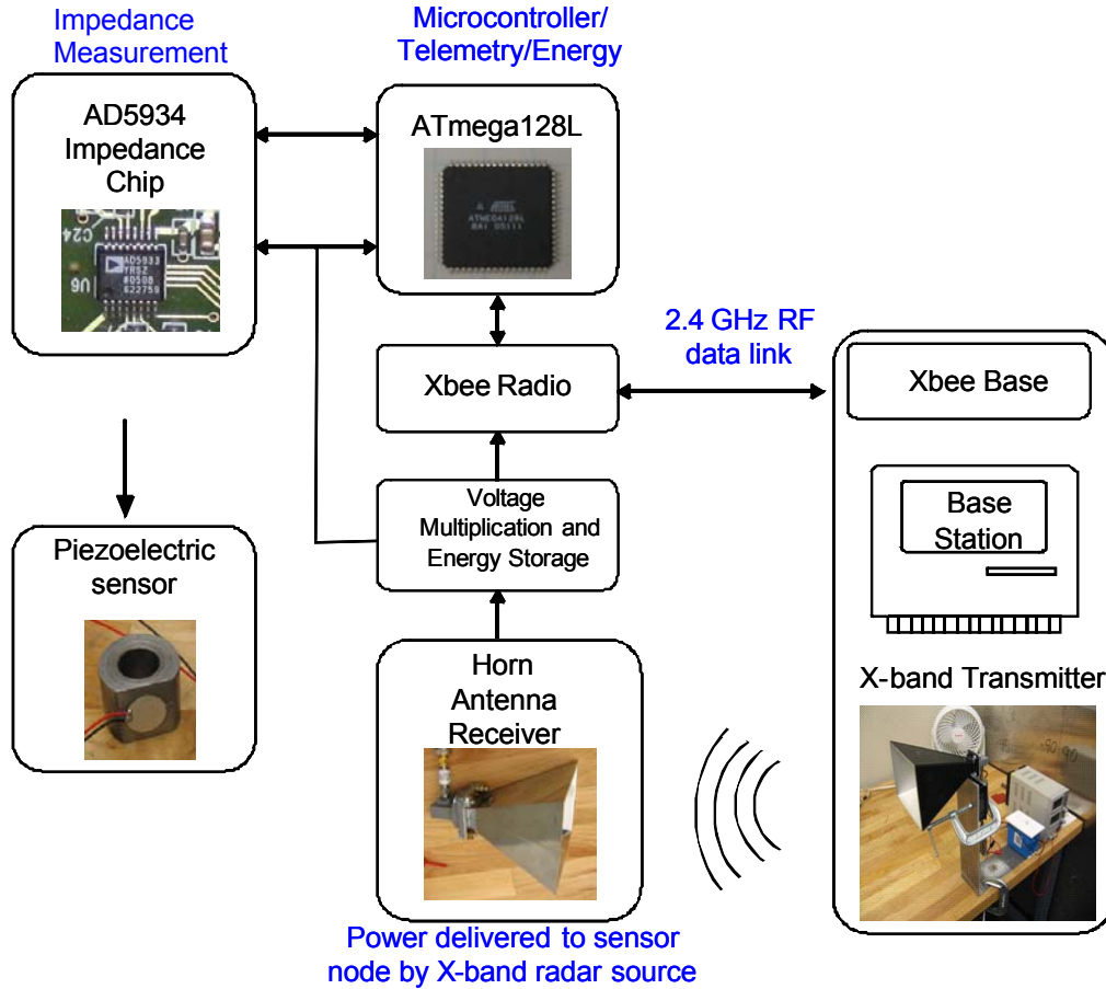
Figure 2. Block Diagram of proposed sensor node
