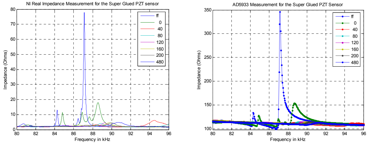
Figure 7: Experimental results with NI system (left) and the sensor node (right).
