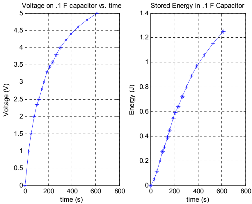
Figure 9. Voltage and Energy storage across 0.1 F supercapacitor as X band Source transmits power.
