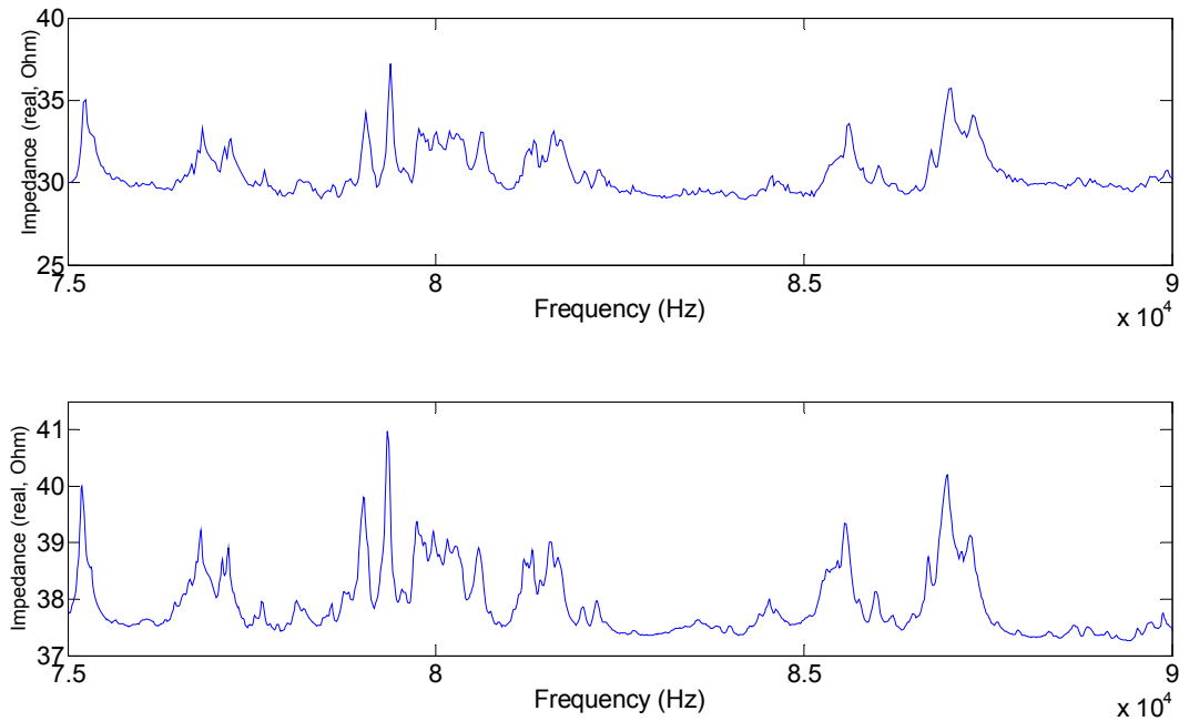
Figure 5: Impedance Measurement from AD5933 (Top) and National Instruments System (Bottom).
