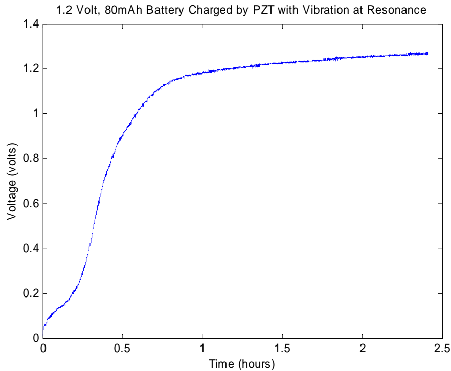
Figure 1: Typical charge cycle of a nickel metal hydride battery, in this case an 80mAh battery was charged (Sodano, 2003a).
