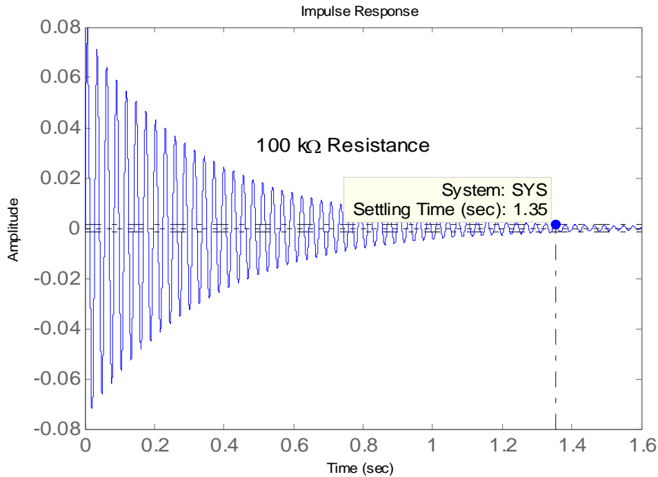
Figure 3: Impulse response with a 100k \Omega resistive load (Sodano, 2003b).
