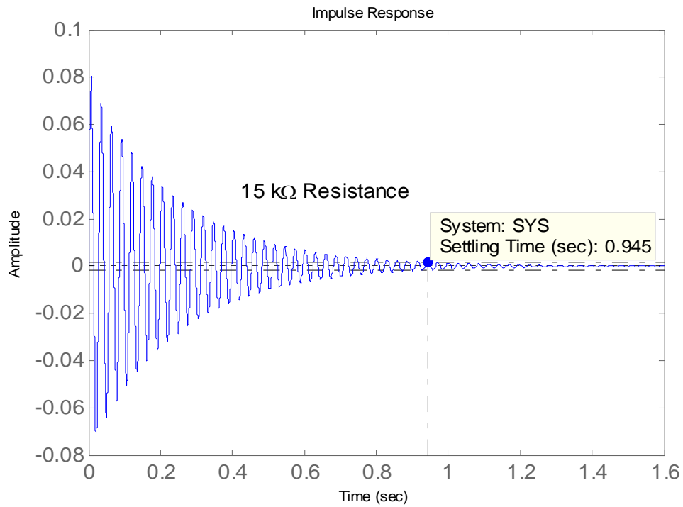
Figure 2: Impulse response with a 15kΩ resistive load (Sodano, 2003b).
