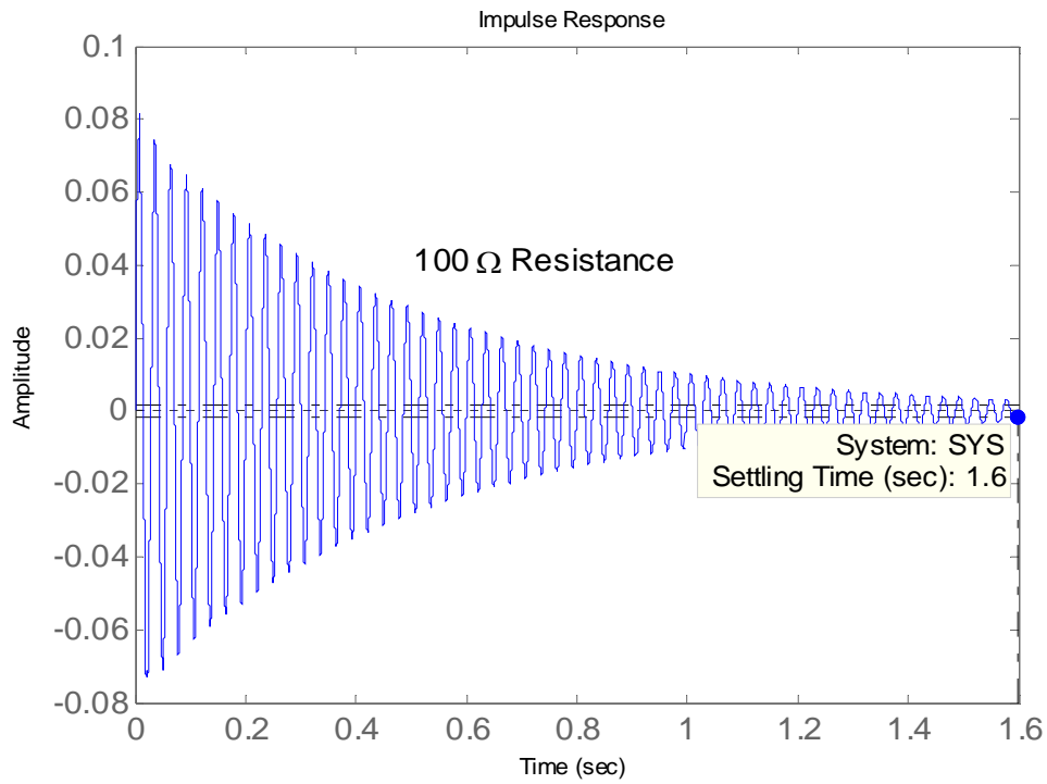
Figure 1: Impulse response with a 100Ω resistive load (Sodano, 2003b).
