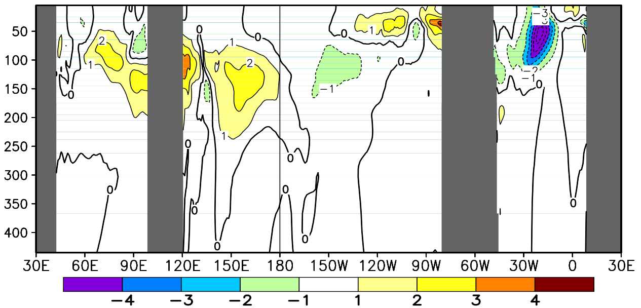
FIGURE T17. Equatorial depth–longitude section of ocean temperature (top) and ocean temperature anomalies (bottom) for AUG 2008. Contour interval is 1°C. Dashed contours in bottom panel indicate negative anomalies. Data are derived from the NCEP’s global ocean data assimilation system version 2 which assimilates oceanic observations into an oceanic GCM (Xue, Y. and Behringer, D.W., 2006: Operational global ocean data assimilation system at NCEP, to be submitted to BAMS). Anomalies are departures from the 1982–2004 base period means.
