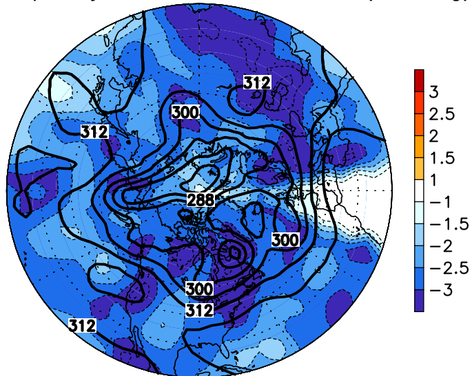
FIGURE E13. Northern Hemisphere: 700-hPa heights for AUG 2008 overlaid with standard deviation of high-pass filtered height (left) and normalized anomalous variance of high-pass filtered height (right). Heights are indicated by thick solid contours in both panels (interval is 60 m). High-pass filtered fields reflect fluctuations having periods less than 10 days, and are indicated by thin contours and shading. Contour interval for standard deviation is 15 m with values > 45 m shaded. Contour interval for normalized variance is 1 standard deviation, with positive values shown by solid contours and dark shading and negative values shown by dashed contours and light shading. Anomalies are departures from the 1964-93 base period monthly means.
