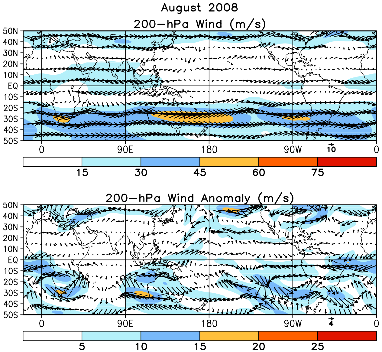
FIGURE T21. Mean (top) and anomalous (bottom) 200-hPa vector wind (CDAS/Reanalysis) for AUG 2008. Contour interval for isotachs is 15 \text{ ms}^{-1} (top) and 5 \text{ ms}^{-1} (bottom). Anomalies are departures from 1979–95 base period monthly means.
