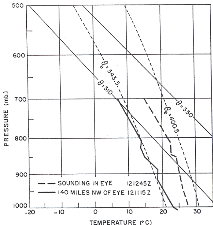
FIGURE 5.—Dropsonde in hurricane Diane, August 12, 1955.
