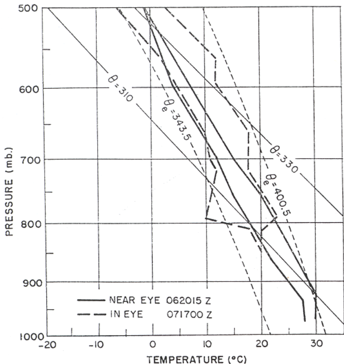
FIGURE 1.—Dropsondes in hurricane Connie, August 6 and 7, 1955.
