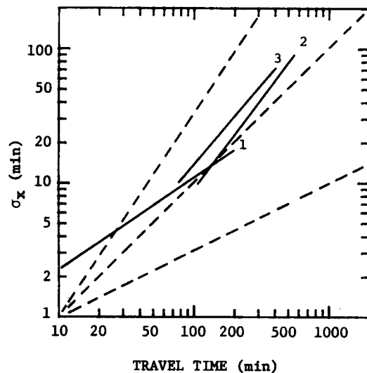
Figure 3. Summary of dispersion data at: 1 - Ft. Wayne, 2 - Victoria, and 3 - Oceanside. The dashed lines show lines with slopes of 0.5, 1.0 and 1.5.
