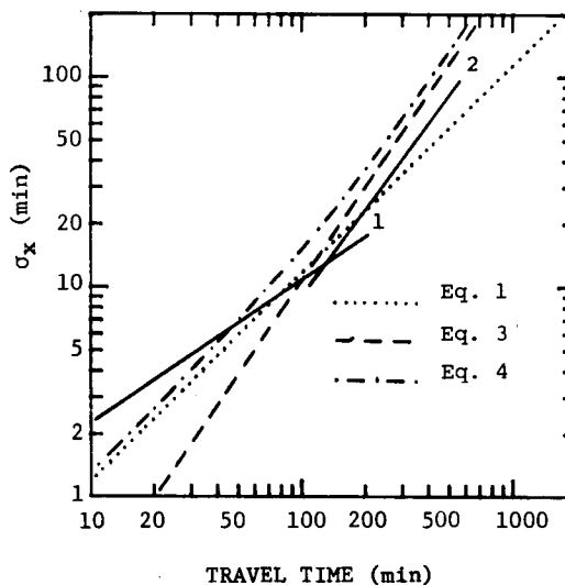
Figure 4. The dispersion data at Ft. Wayne (1) and Victoria (2) compared to predictions of along-wind dispersion by turbulence (Eq. 1), wind shear (Eq. 3), and the combined effects of both (Eq. 4).
