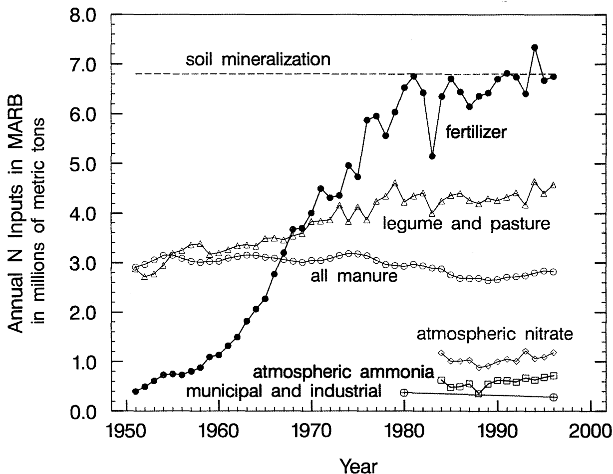
FIGURE 5.7. Annual nitrogen inputs to the Mississippi–Atchafalaya River Basin, 1951–96 NOTE: See text for sources of data and methods used to estimate inputs.
