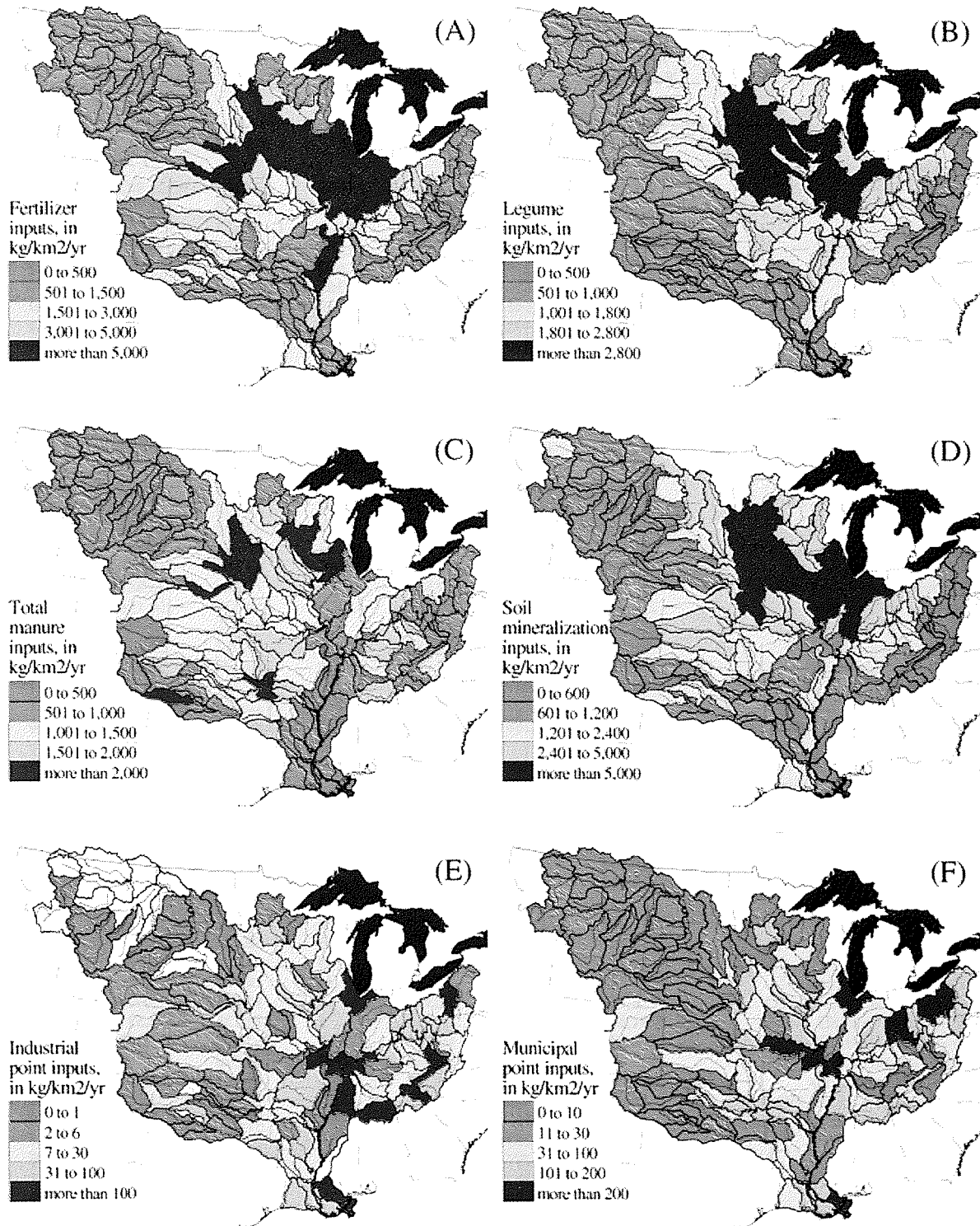
FIGURE 5.8. Nitrogen inputs in hydrologic accounting units in 1992 from (A) fertilizer, (B) legumes, (C) livestock manure, (D) soil mineralization, (E) industrial point sources, and (F) municipal point sources.
