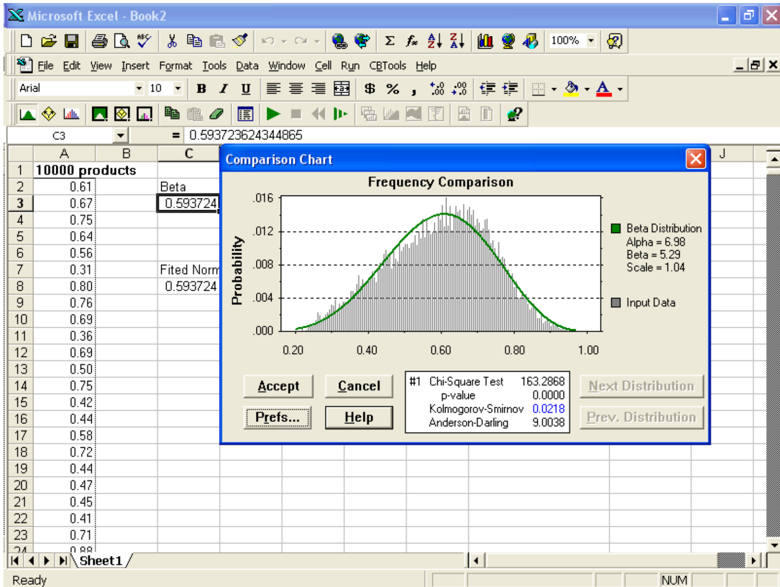
Figure 3.7-2. The Best-Fitting Beta Distribution, Fitted to the Sample of 10,000 Products
