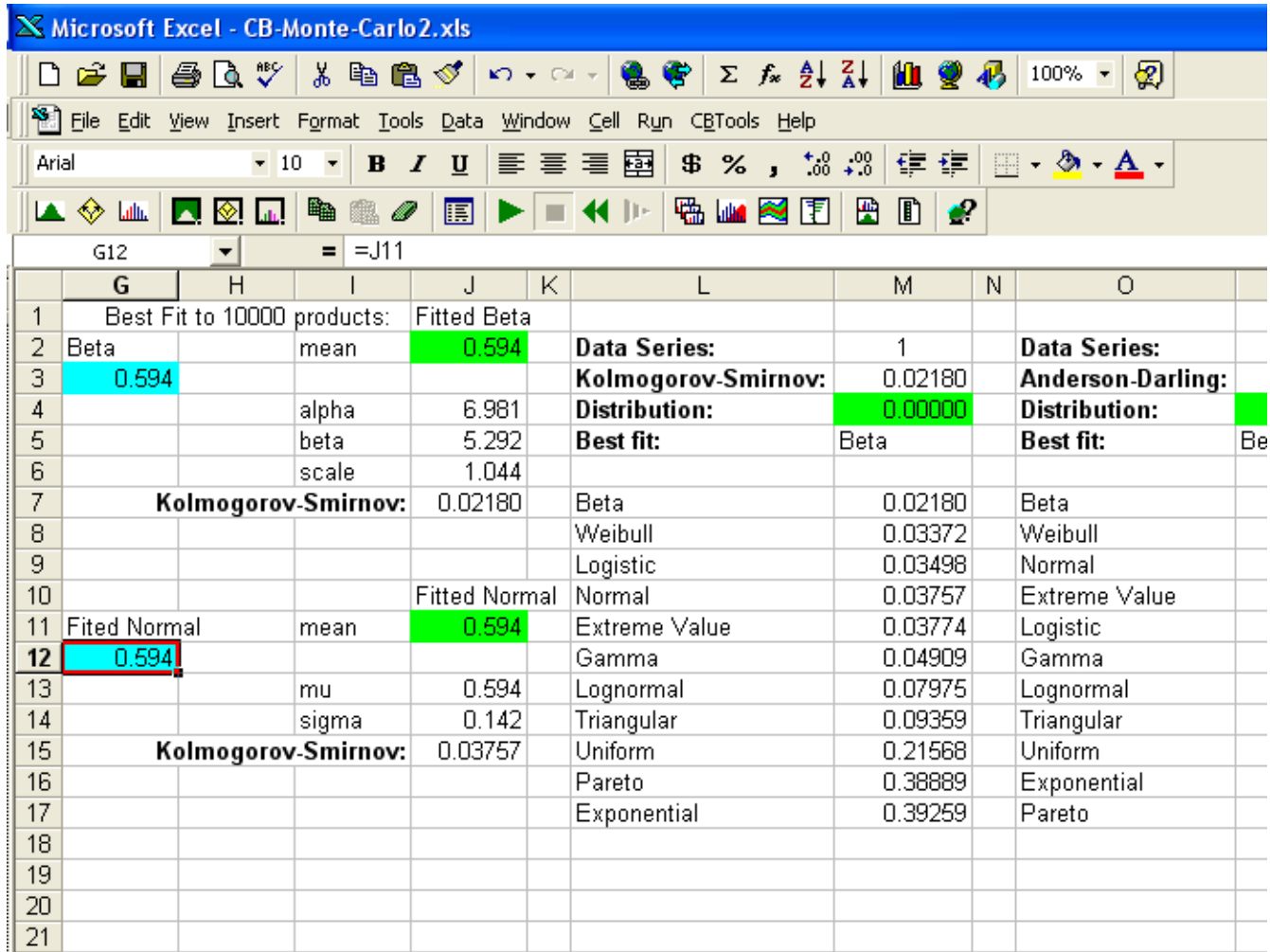
Figure 3.7-1. K-S and A-D Statistics for All Distributions Fitted to a Sample of 10,000 Products using Crystal Ball 2000 Batch Fit Procedure
