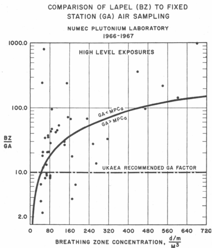
Figure 3.10-1. Comparison of Lapel to Fixed Station Air Sampling (Source: Caldwell et al. 1967)
