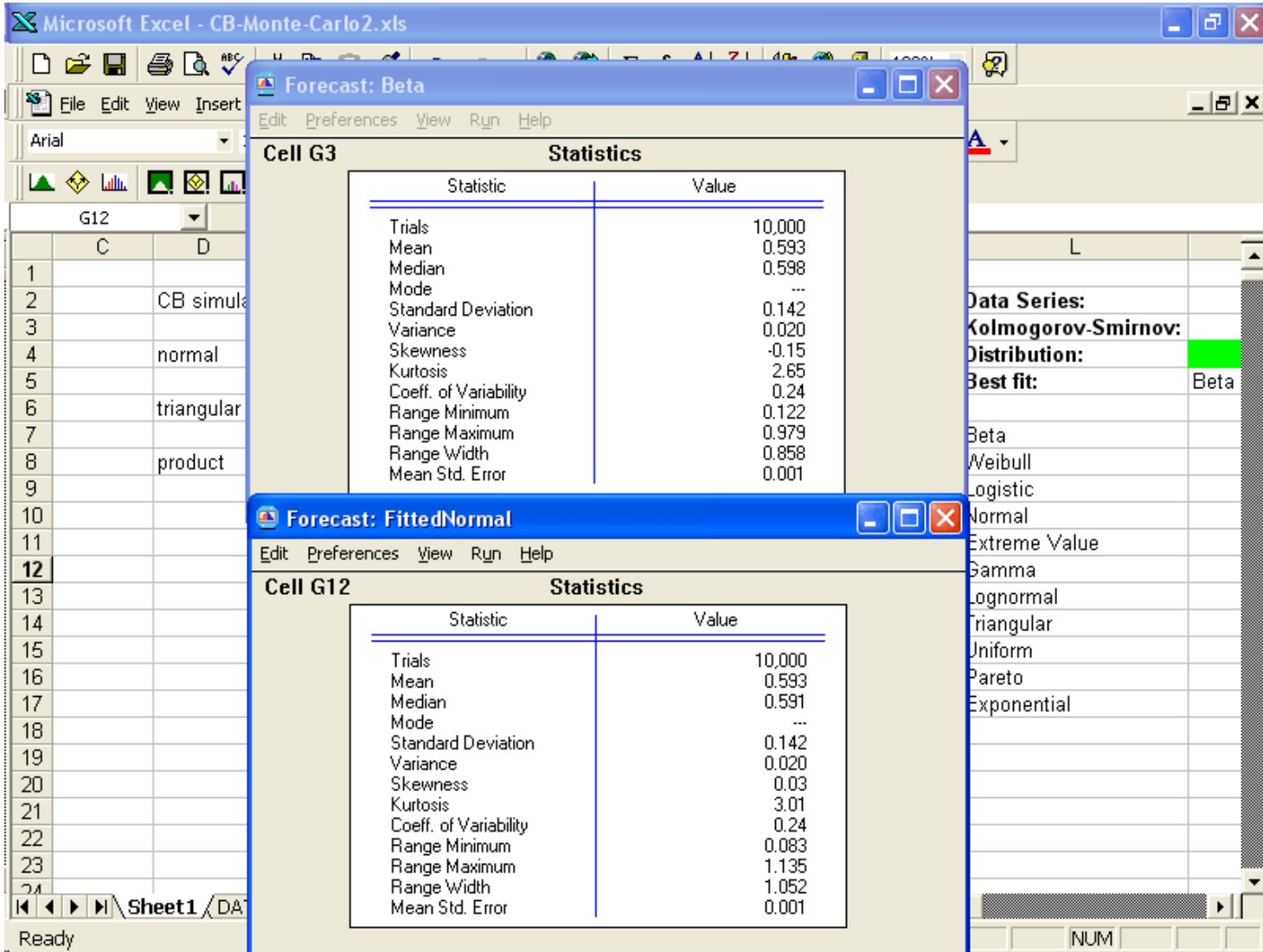
Figure 3.7-4. Comparison of Statistics Obtained from Samples of Size 10,000 from the Best-Fitting Beta Distribution and the Best-Fitting Normal Distribution
