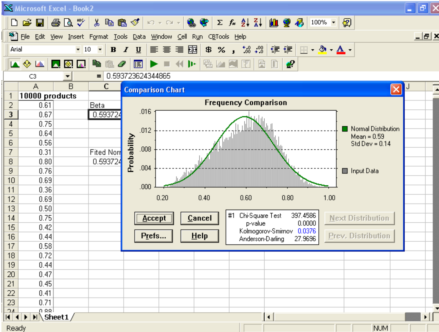
Figure 3.7-3. The Best-Fitting Normal Distribution, Fitted to the Sample of 10,000 Products
