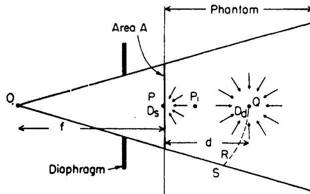
Figure 5.1 Diagram to Illustrate the Meaning of Surface Backscatter and Percentage Depth Dose
