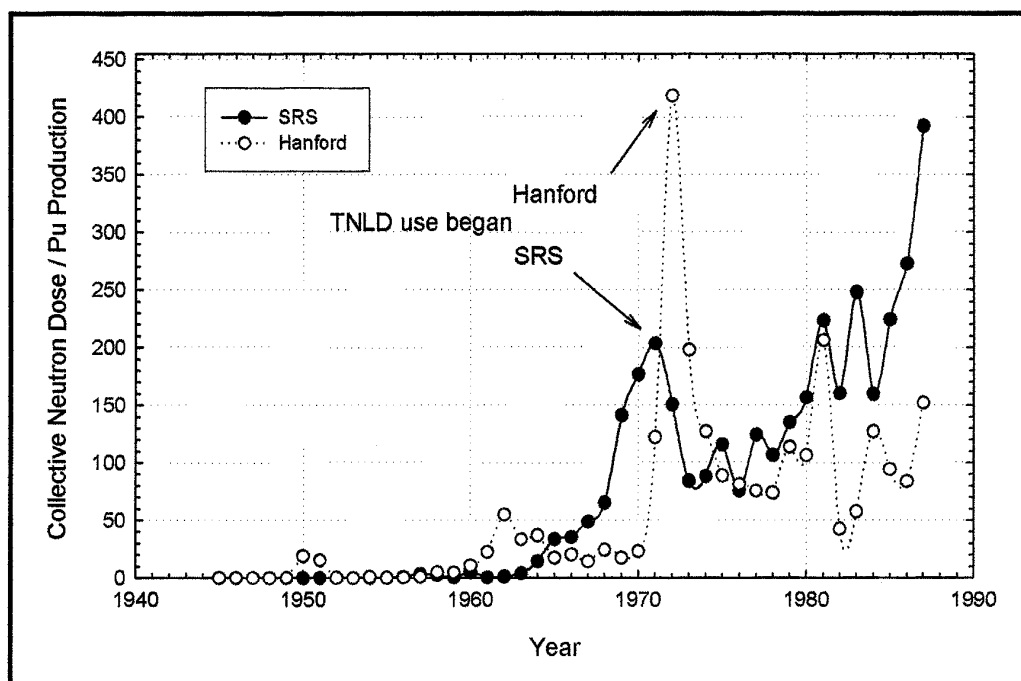
Figure 5.3 Trends in SRS and Hanford Collective Neutron Dose Normalized to Plutonium Production
