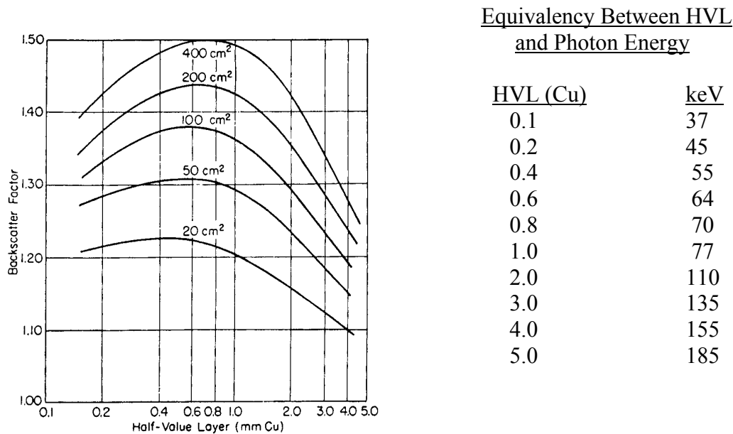
Figure 5.2 Variation of the Backscatter Factor with the Quality of the Radiation for a Number of Field Sizes (Source: Hine and Brownell 1956)
