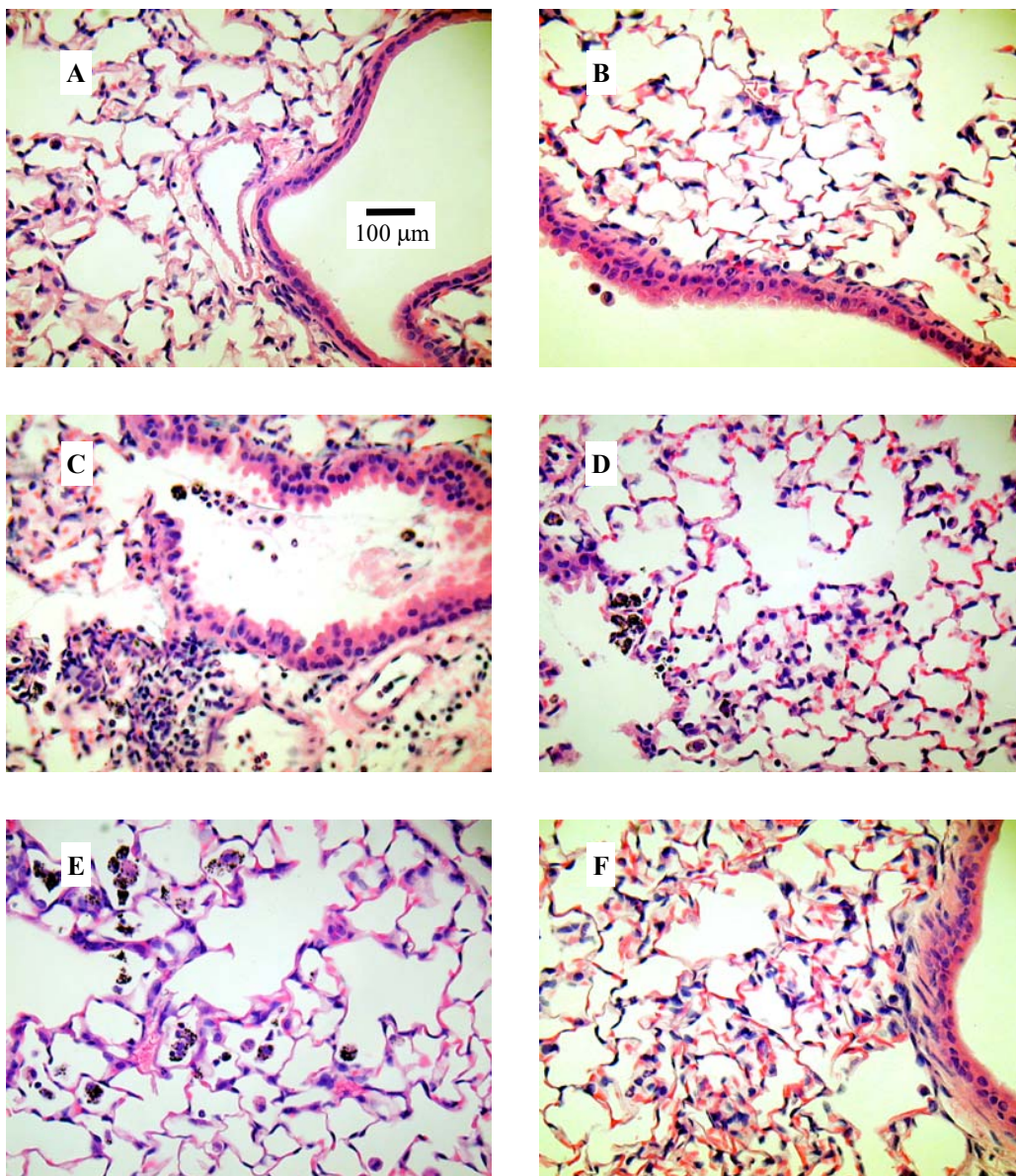
Figure 18. Experiment C. Representative micrographs of lesions occurring in lungs of mice 1 or 3 days after intratracheal instillation of 100 µg PM sample or saline vehicle (all panels same magnification: bar length = 100 µm). A. Saline-instilled control mouse (#301), Day 1, with no remarkable findings. B. Mouse #349 instilled with WTCC, Day1, showing minimal degree of focal subacute bronchiolar inflammation (FSBI). C. Mouse #291 instilled with NIST, Day 1, with moderate degree of FSBI. D. Mouse #270 instilled with WTC13, Day 1, with moderate degree of FSBI. E. Mouse #300 instilled with NIST, Day 3, with slight/mild degree of FSBI. F. Mouse #280 instilled with WTC13, Day 3, with minimal degree of FSBI.
