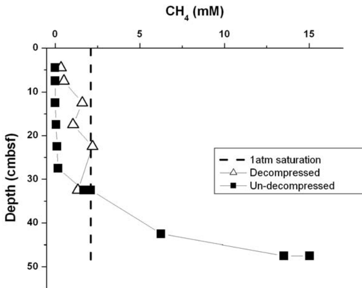
Figure 3: Methane concentrations at 1-atm saturation (dotted line), are compared to data from the original pre-adaptation instrument (where samples were allowed to decompress) and from the adapted instrument outfitted with high-pressure sample chambers and valves (un-decompressed samples). Figure adapted from Lapham, 2007 dissertation.
