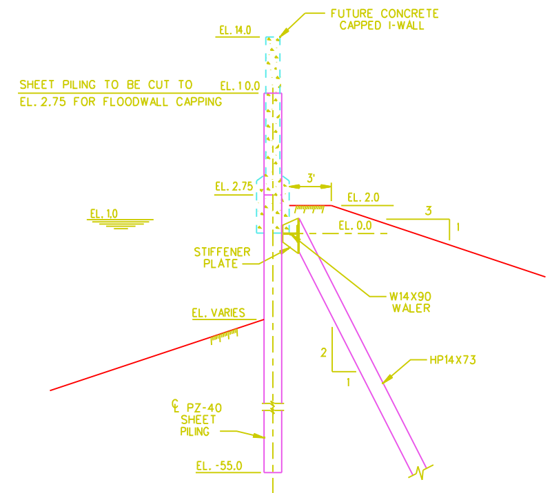
SECTION F 30 31 SECTION G SIMILAR SCALE: 1/4" = 1'-0"
