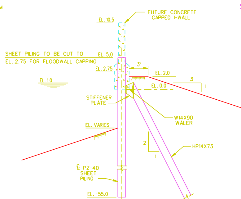
SECTION D 30 31 SECTION E SIMILAR SCALE: 1/4" = 1'-0"
