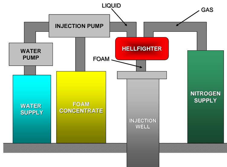
Figure 1. Schematic of surface foam injection system.
