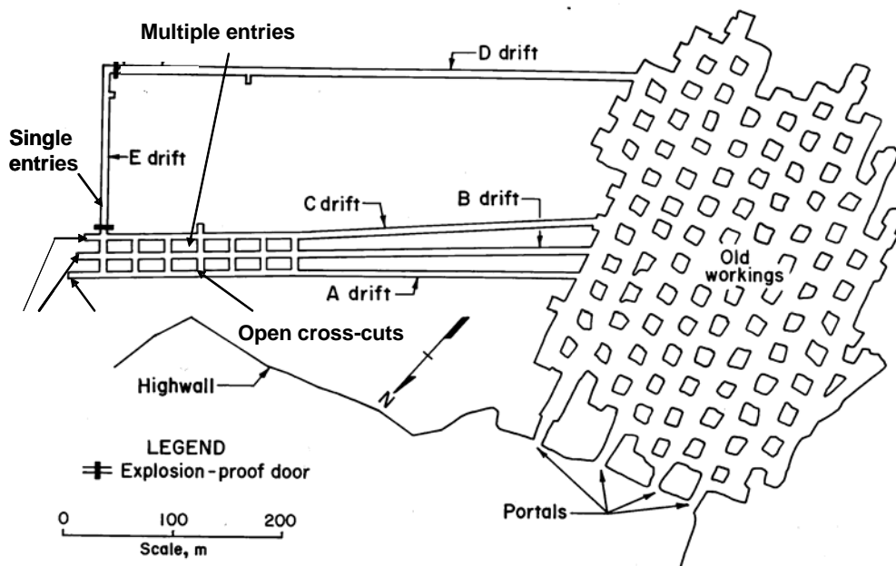
Figure 5. Schematic of Lake Lynn Experimental Mine.
