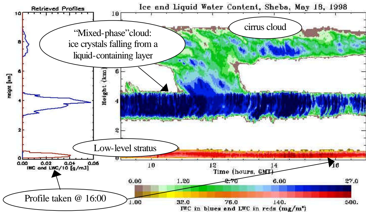
Figure 1. Time-height image of retrieved ice water content (blues) and liquid water content (reds) on May 18, 1998 at SHEBA next to a profile of the same parameters taken at 16:00. The image shows an ice cloud, a mixed-phase cloud (the ice component only), and a low-level stratus layer.
