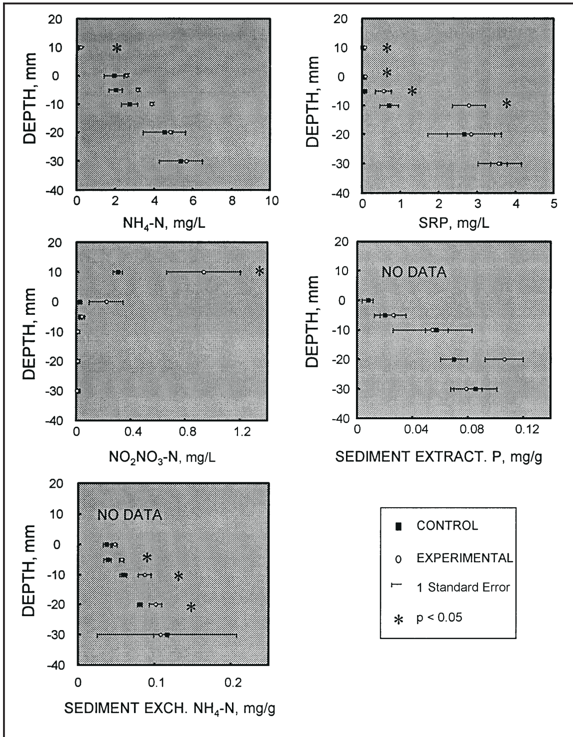
Figure 1. Variations in mean concentrations of ammonium nitrogen (NH 4 -N), nitrate-nitrite nitrogen (NO 2 NO 3 -N), and soluble reactive phosphorus (SRP) in the overlying water and sediment pore water, and variations in sediment exchangeable ammonium nitrogen (EXCH. NH 4 -N) and extractable phosphorus (EXTRACT. P) in experimental and control microcosms. Negative depths indicate depths in the sediment below the sediment-water interface
