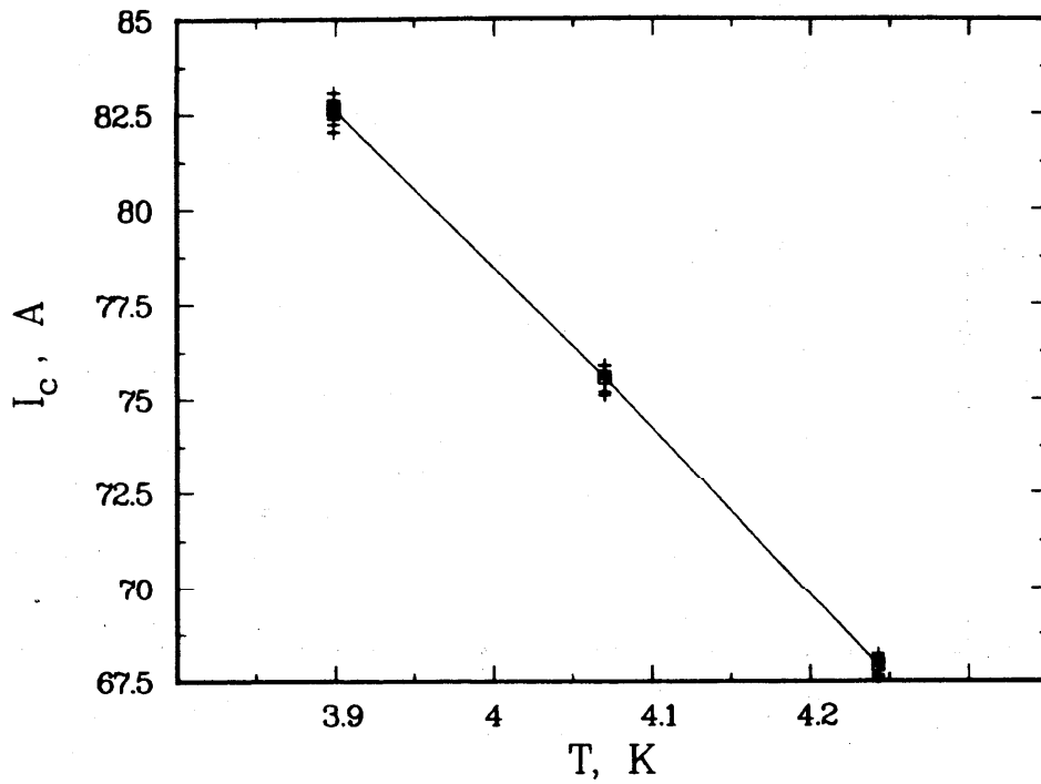
Figure 10d. Critical current measurements at 8 T and 0.2 \mu\text{V}/\text{cm} : I_c (+) and average I_c ( \square ) versus temperature.
