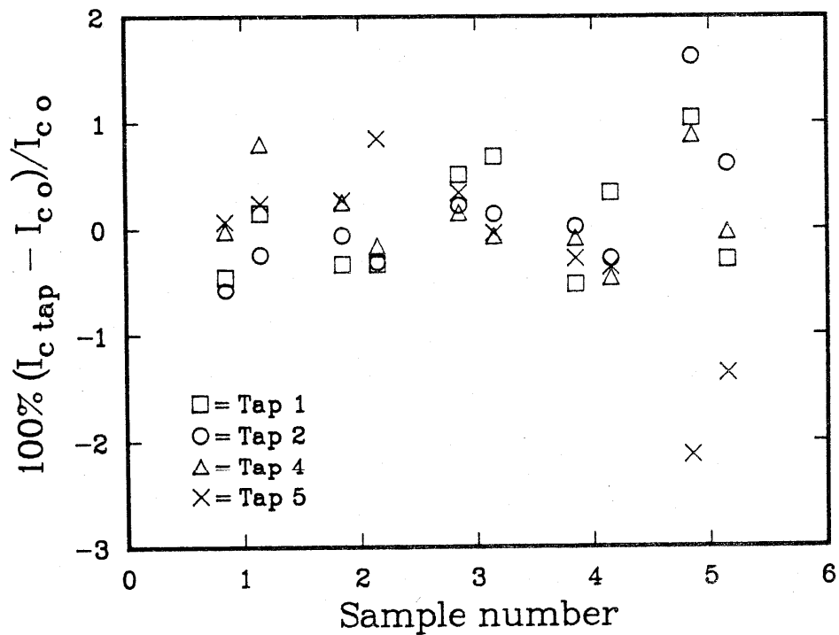
Figure 7. Short-range homogeneity of the 5 and 50 m specimens of each sample. The 50 m data are shifted slightly to the right and the 5 m data to the left over the sample number. Plotted are the percentage differences between the measured I_c on the center voltage tap and that of the other four taps (at 4 T).
