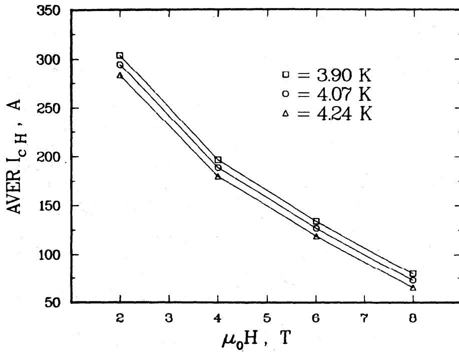
Figure 13a. Dependence of I_c on temperature and magnetic field at 0.05 \mu\text{V}/\text{cm} ; points plotted are sample means.
