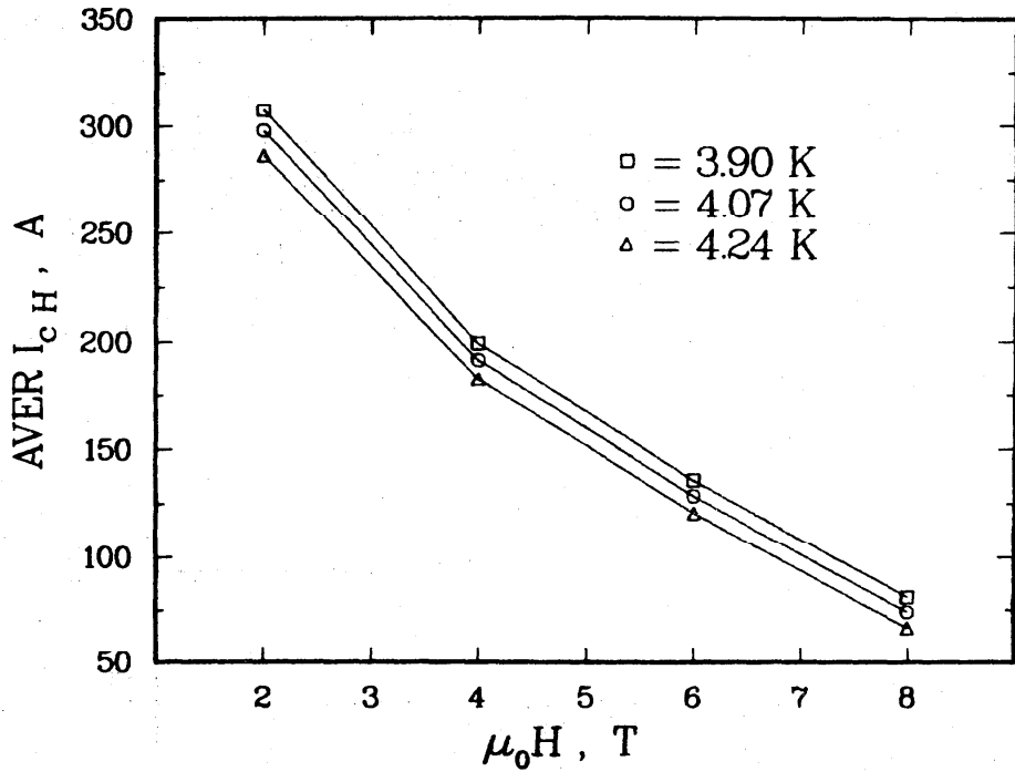
Figure 13b. Dependence of I_c on temperature and magnetic field at 0.10 \mu\text{V}/\text{cm} ; points plotted are sample means.
