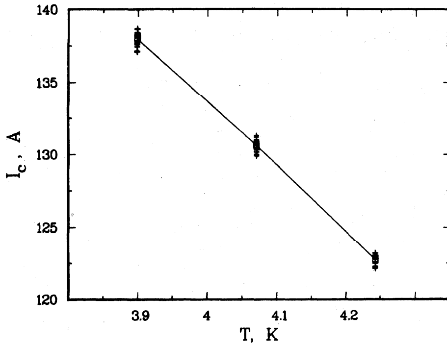
Figure 10c. Critical current measurements at 6 T and 0.2 \mu\text{V}/\text{cm} : I_c (+) and average I_c ( \square ) versus temperature.
