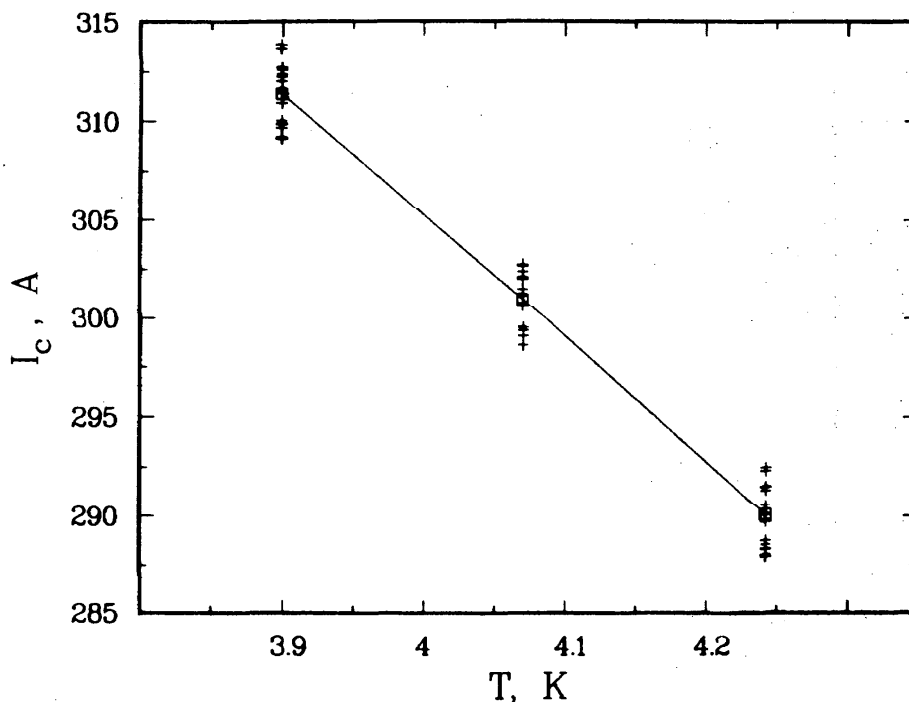
Figure 10a. Critical current measurements at 2 T and 0.2 \mu\text{V}/\text{cm} : I_c (+) and average I_c ( \square ) versus temperature.
