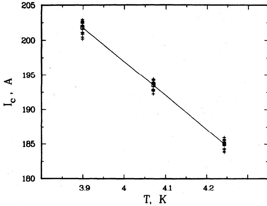
Figure 10b. Critical current measurements at 4 T and 0.2 \mu\text{V}/\text{cm} : I_c (+) and average I_c ( \square ) versus temperature.
