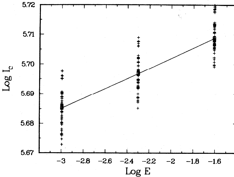
Figure 11a. Critical current measurements at 2 T and 4.07 K; natural log I_c (+) and average natural log I_c ( \square ) versus natural log of electric field criterion.
