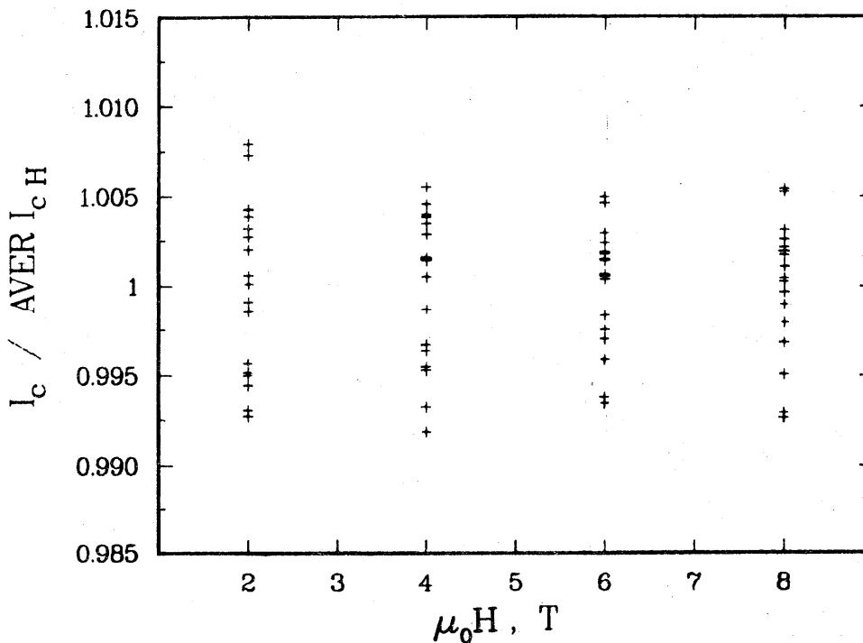
Figure 9a. Critical current measurements at 3.90 K and 0.2 \mu\text{V}/\text{cm} : ( I_c /average I_c ) versus magnetic field.
