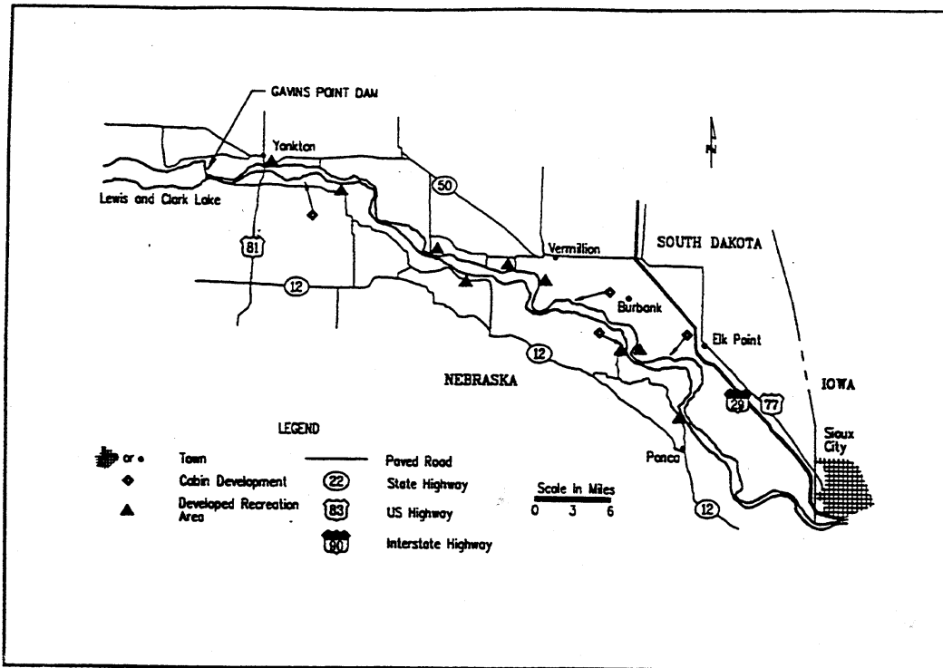
Figure 3.12-10. River reach from Gavins Point Dam, Nebraska, to Sioux City, Iowa.
