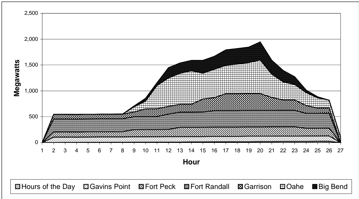
Figure 3.11-2. Typical summer load pattern (reservoirs full, normal releases).
