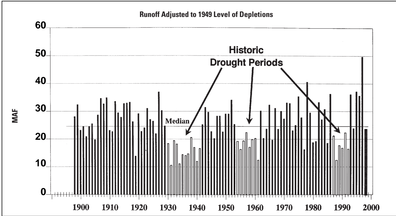
Figure 3.3-1. Annual runoff at Sioux City, Iowa.
