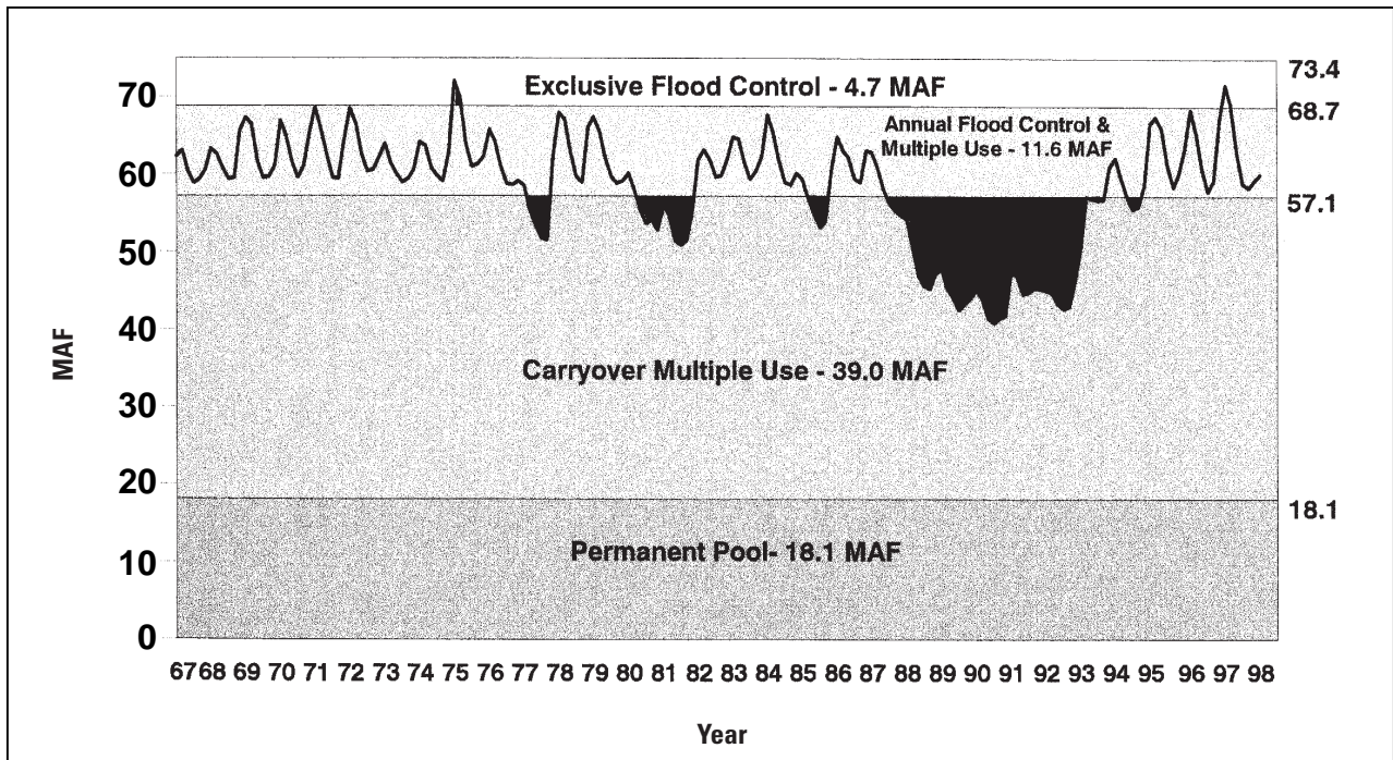
Figure 3.3-2. Total Mainstem Reservoir System end-of-month water in storage (MAF) from 1967 through 1998.
