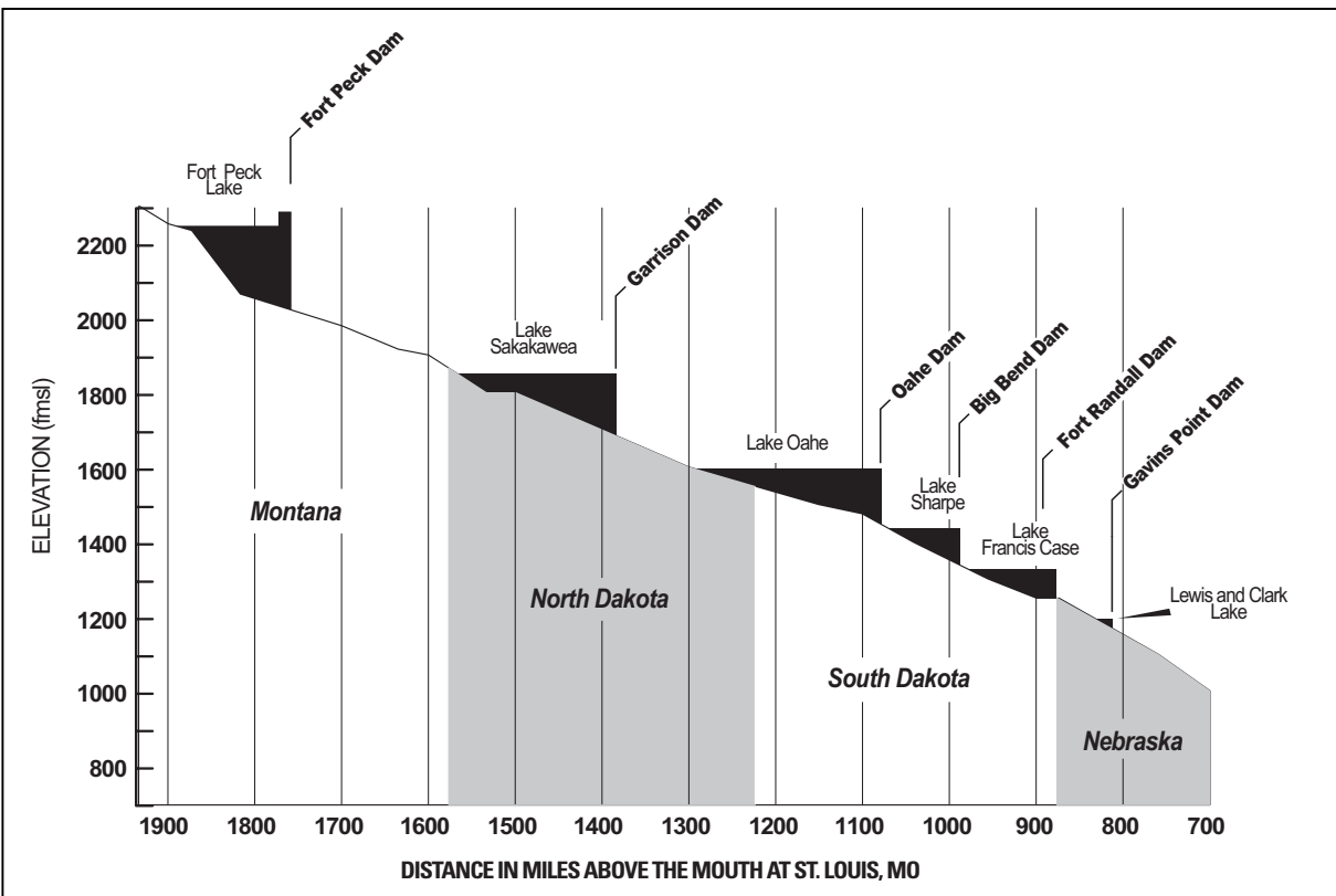
Figure 3.1-2. Profile of Missouri River Mainstem Reservoir System reservoirs.
