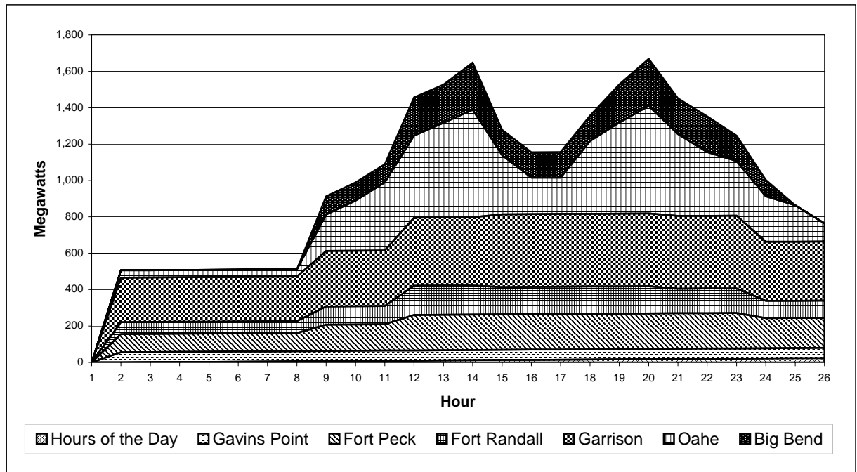
Figure 3.11-3. Typical winter load pattern (reservoirs full, normal releases).
