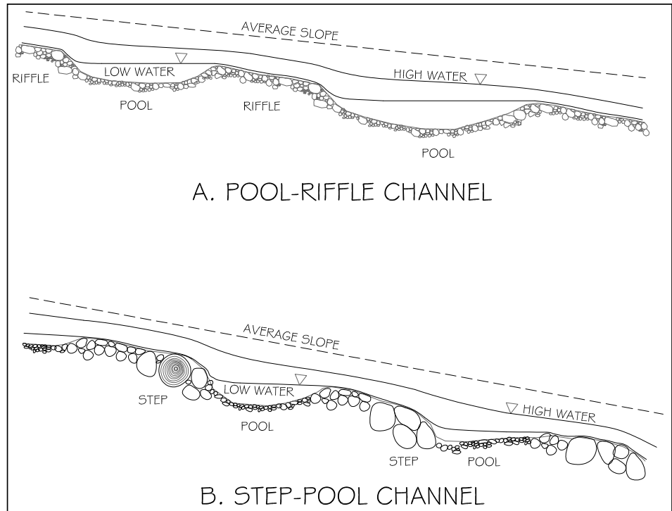
Figure A.8—Pool-riffle and step-pool channel profiles showing variable local slopes. From Knighton (1998). permission to use requested.
