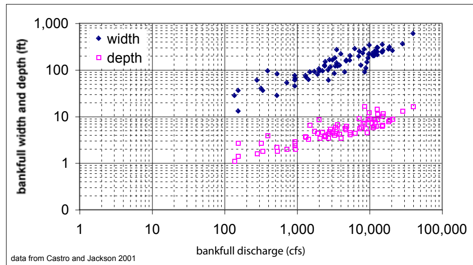
Figure A.18—Relationship of bankfull channel dimensions (determined in the field using geomorphic indicators) to bankfull discharge (determined from gauge records at observed bankfull elevation). Data from Castro and Jackson (2001).
