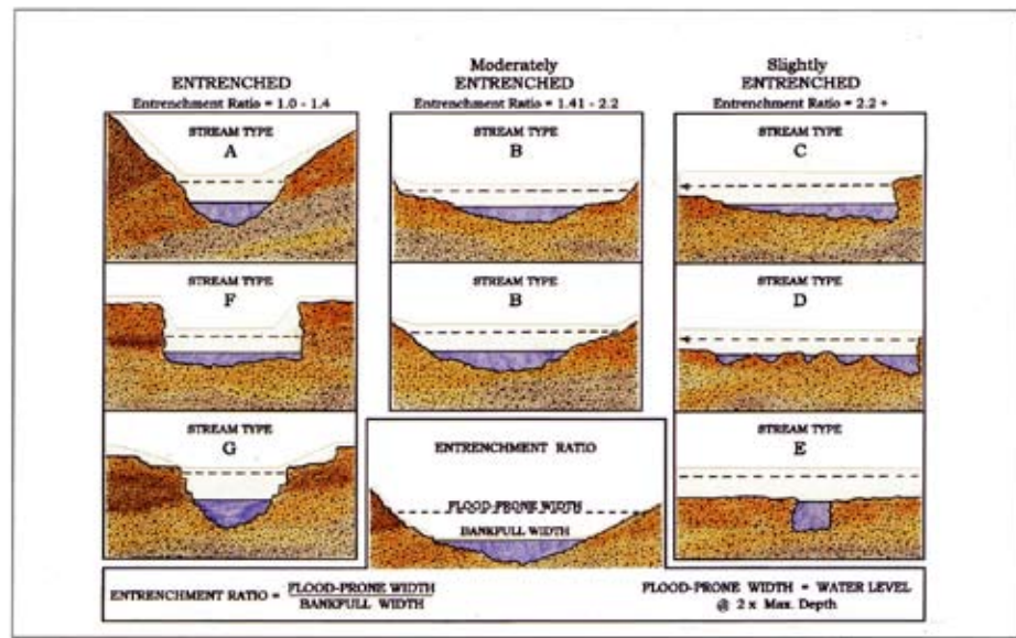
Figure A.13—Channel entrenchment (from Rosgen 1994).
