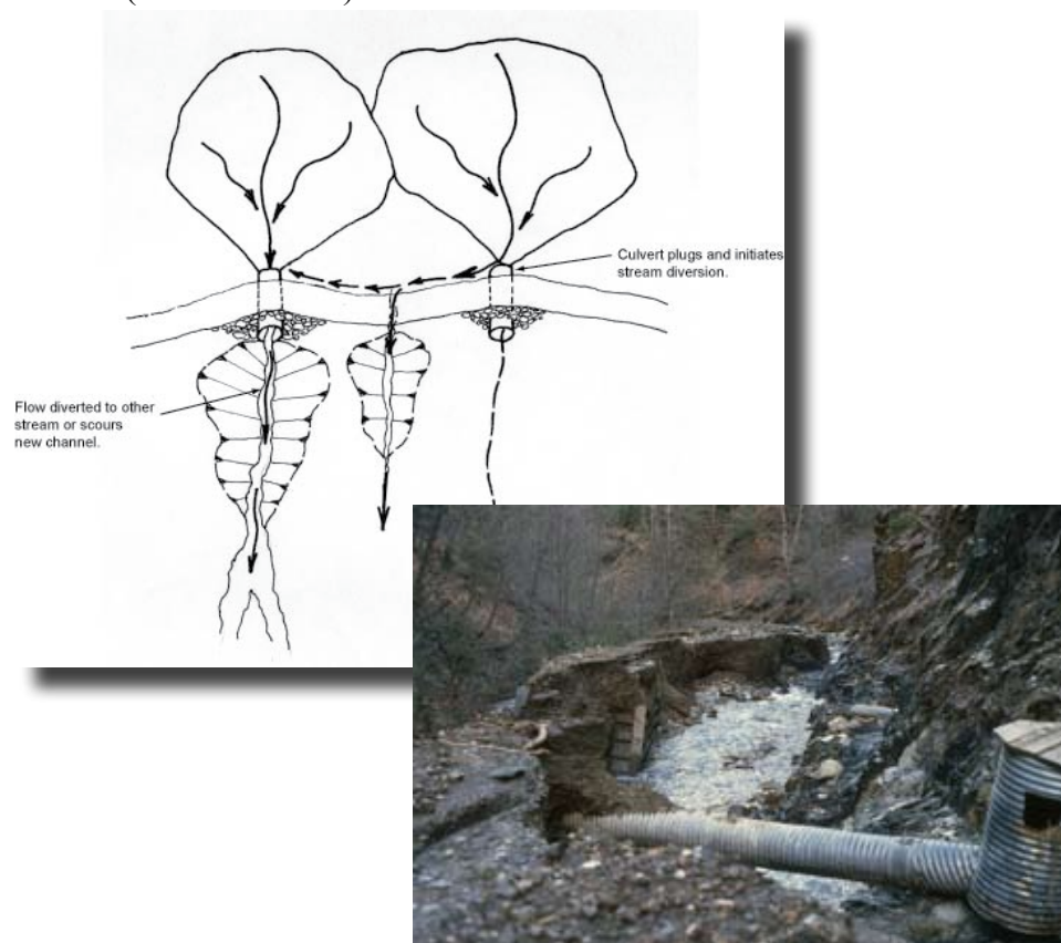
Figure 6.31—Stream diversion at plugged pipe. (inset: Stream diverted down road, Plumas National Forest 1997)
