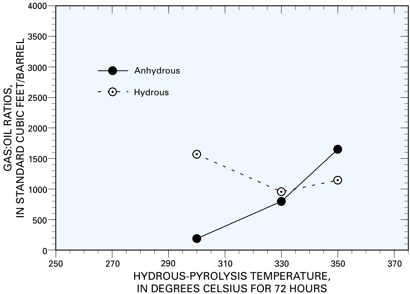
Figure 4. Comparison of gas:oil ratios (GOR) for aliquots of a sample of Woodford Shale (Type-II) subjected to hydrous and anhydrous pyrolysis at 300°, 330°, and 350°C for 72 hours. Original data reported by Lewan (1997, tables 2 and 6).
