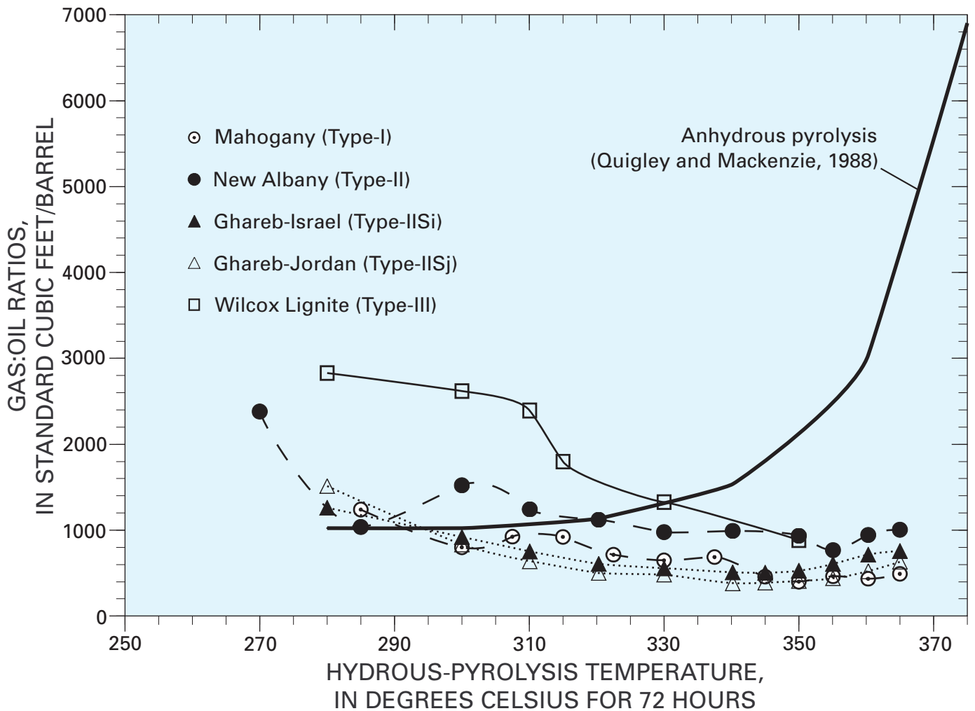
Figure 3. Comparison of gas:oil ratios (GOR) for source rocks with different kerogen types subjected to hydrous- and anhydrous-pyrolysis temperatures between 270° and 365°C for 72 hours.
