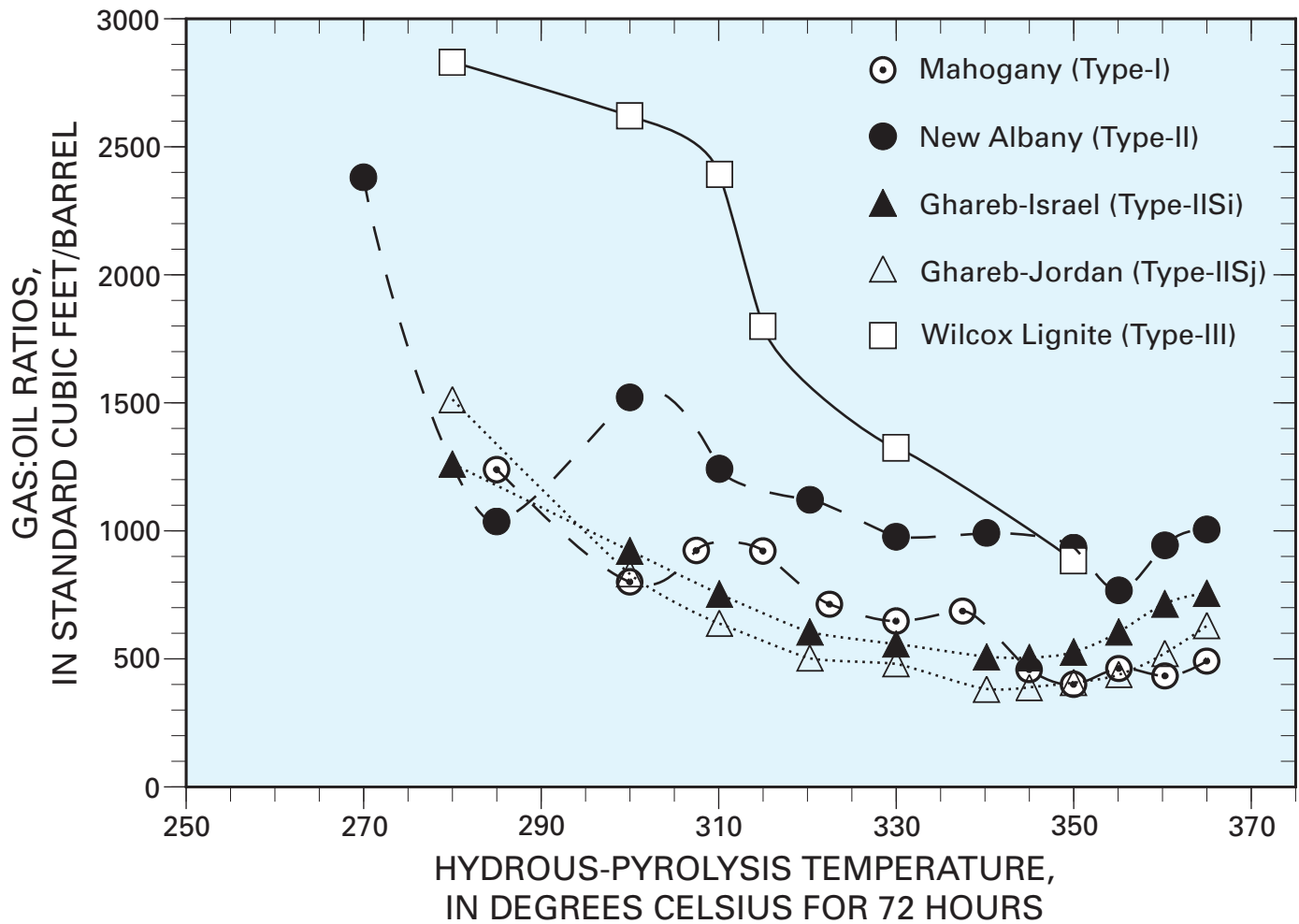
Figure 2. Gas:oil ratios (GOR) for source rocks with different kerogen types subjected to hydrous-pyrolysis temperatures between 270° and 365°C for 72 hours.
