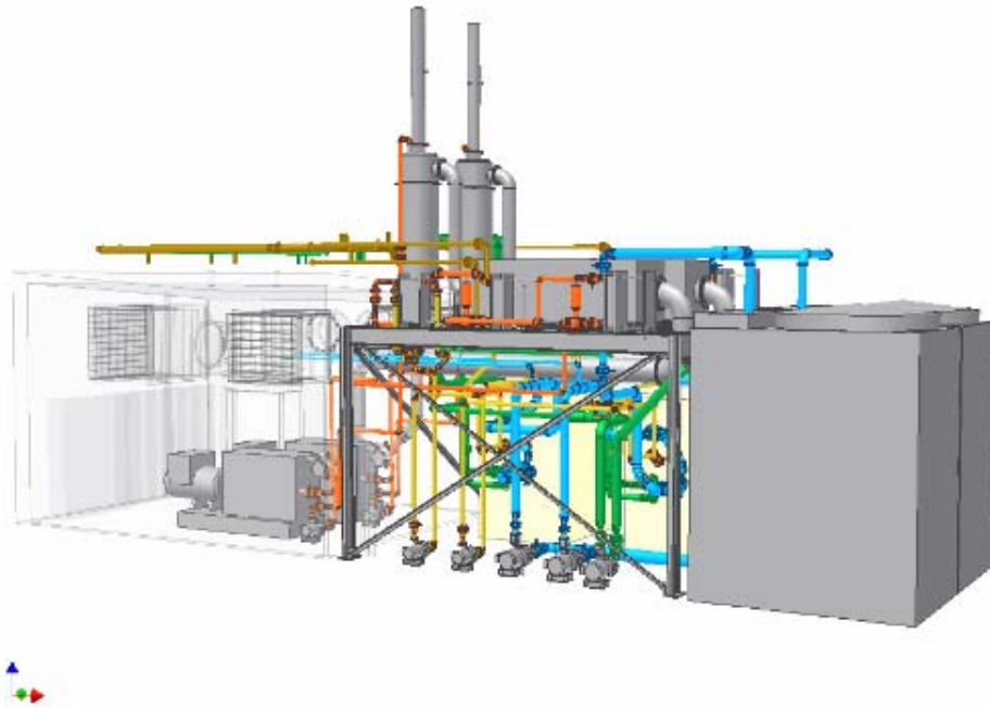
Figure 36: System Layout
