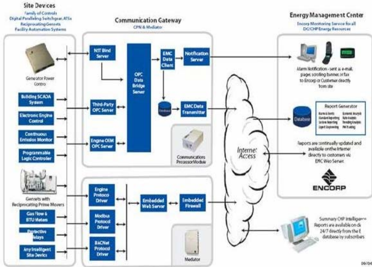
Figure 9: EMC System Architecture
