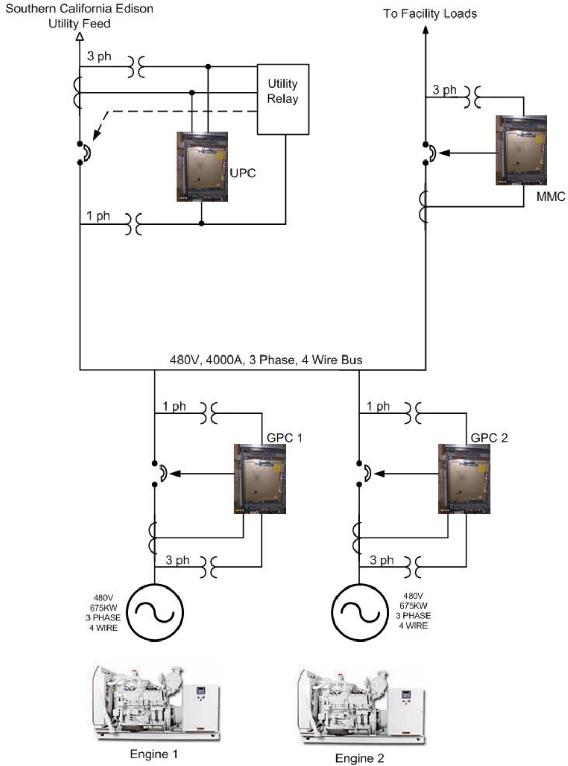
Figure 37: One-Line Diagram
