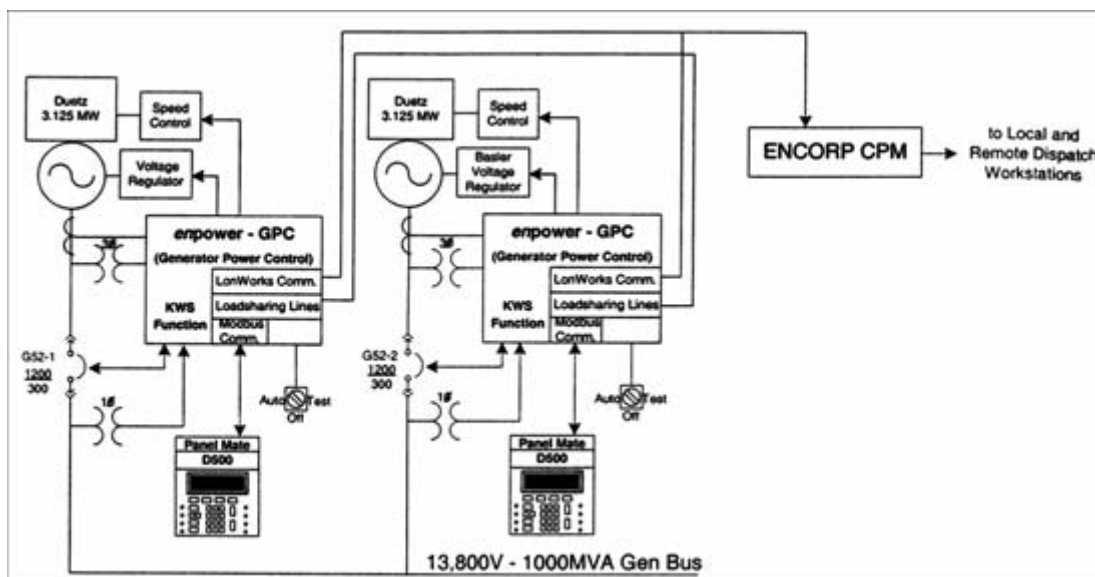
Figure 23: Typical Chowchilla II Two-Engine Configuration
