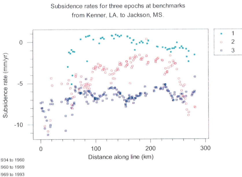
Figure 11. Subsidence rates from Kenner, Louisiana, at left to Jackson, Mississippi, at right.
