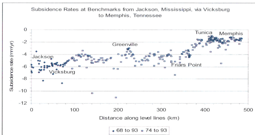
Figure 7. Subsidence rates at benchmarks.
