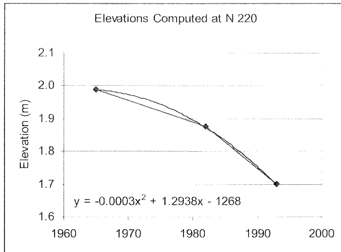
Figure 9. Changes in elevation over time at N 220.
