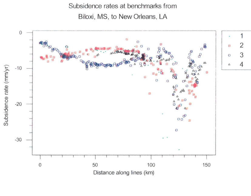
Figure 12. Subsidence rates from Biloxi, Mississippi, at left, to New Orleans, Louisiana, at right.
