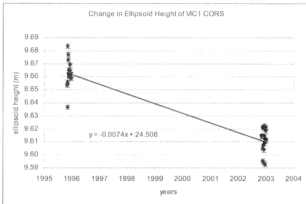
Figure 14. Vertical displacement derived from GPS observations.
