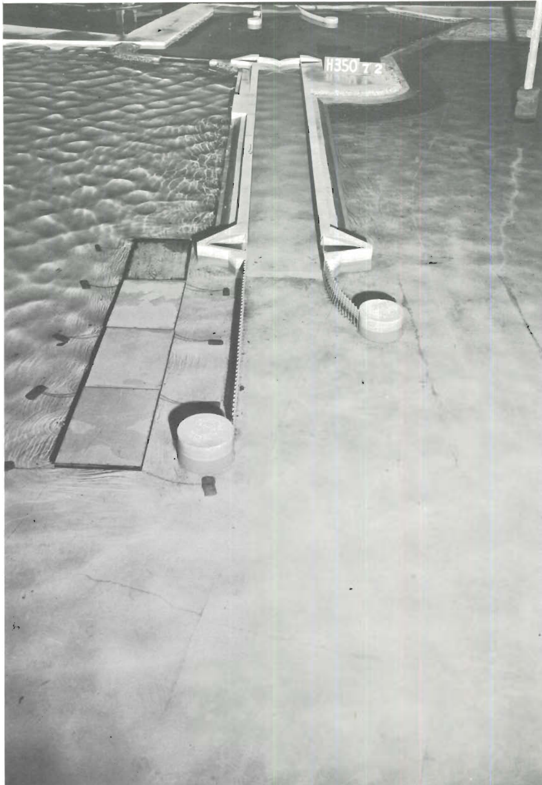
Photo 70. Typical wave patterns at lock entrance for Plan 17C; 3-sec, 4-ft waves from NNW; swl = +1 ft msl
