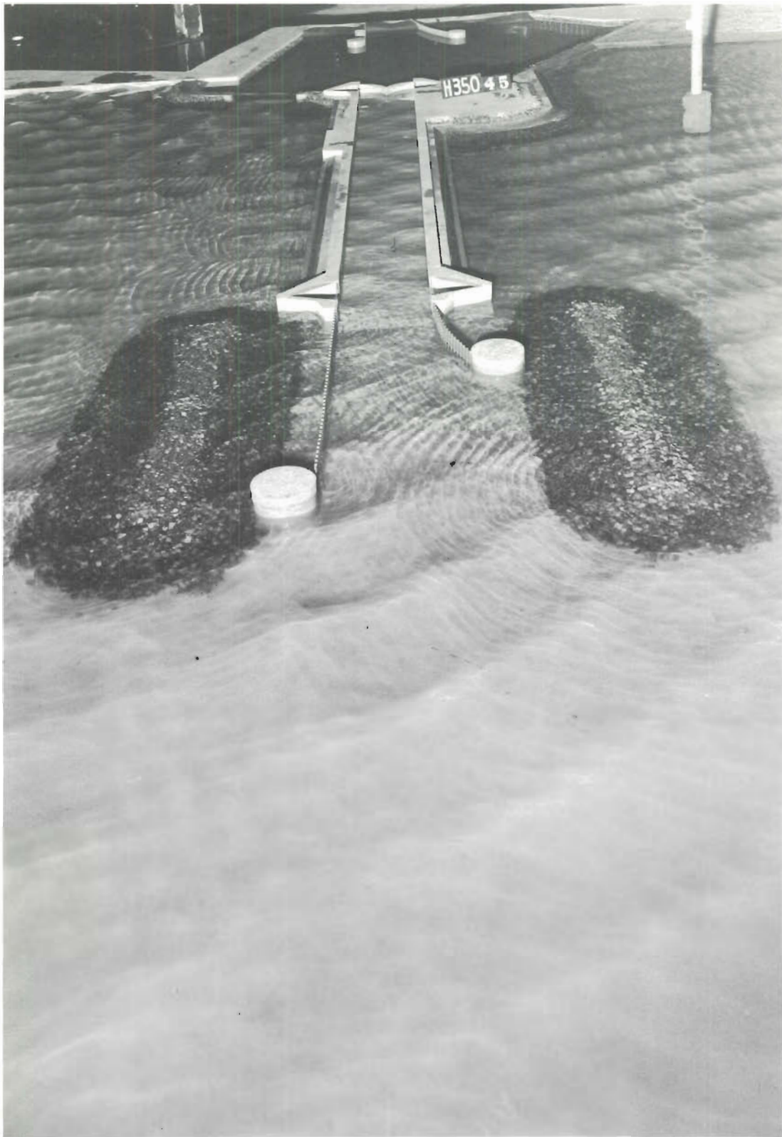
Photo 47. Typical wave patterns at lock entrance for Plan 9; 4-sec, 4-ft waves from NW; swl = +1 ft msl
