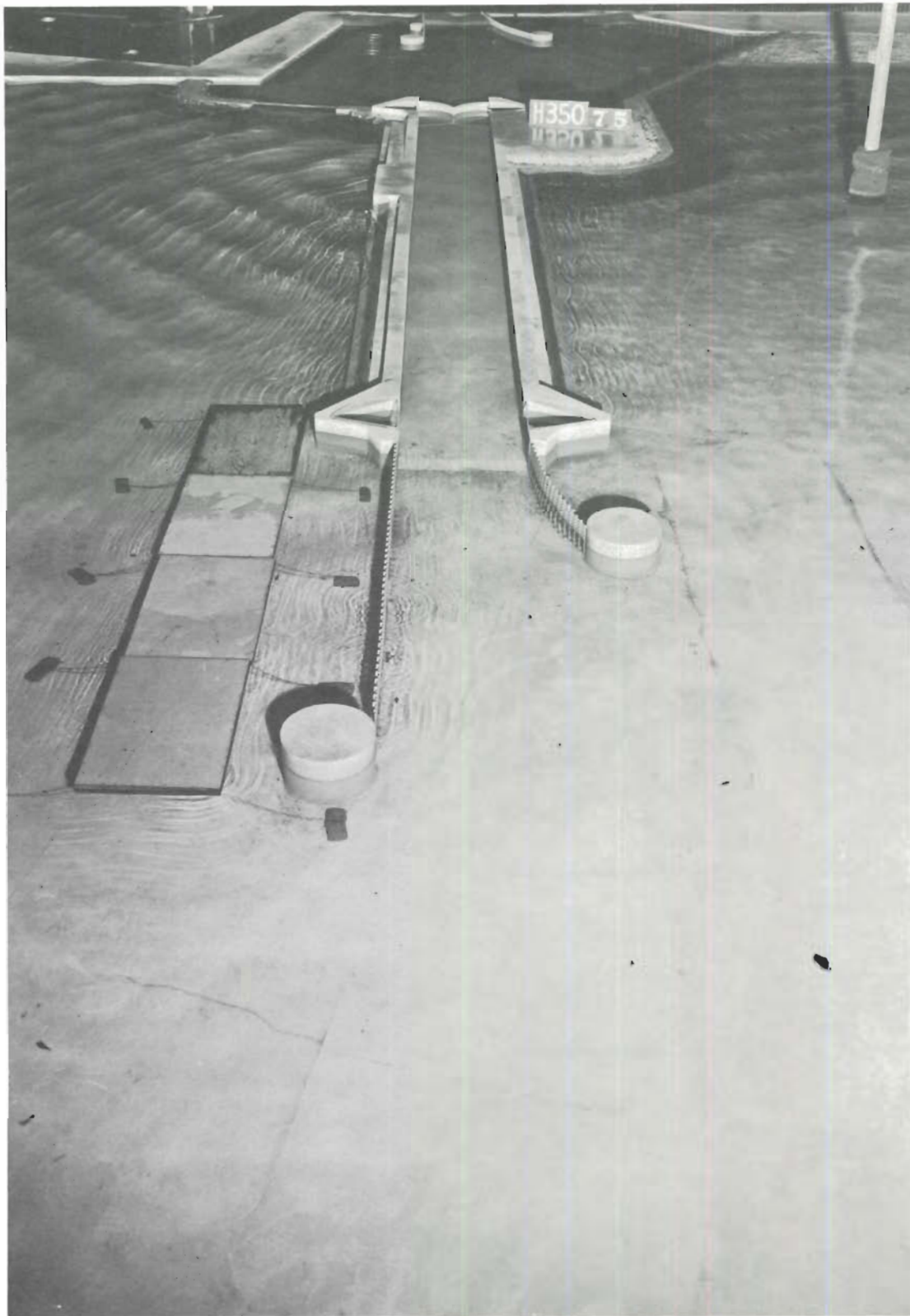
Photo 74. Typical wave patterns at lock entrance for Plan 17C; 4-sec, 4-ft waves from NW; swl = +4 ft msl
