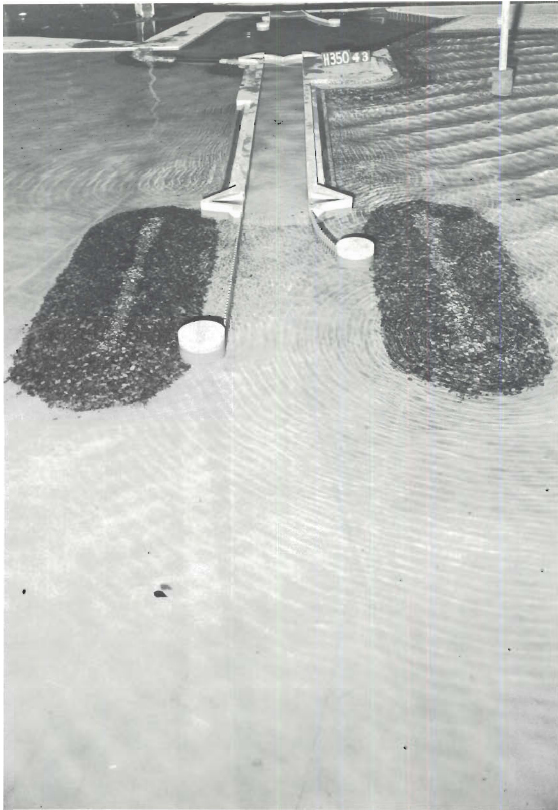
Photo 40. Typical wave patterns at lock entrance for Plan 8; 4-sec, 4-ft waves from NW; swl = +4 ft msl
