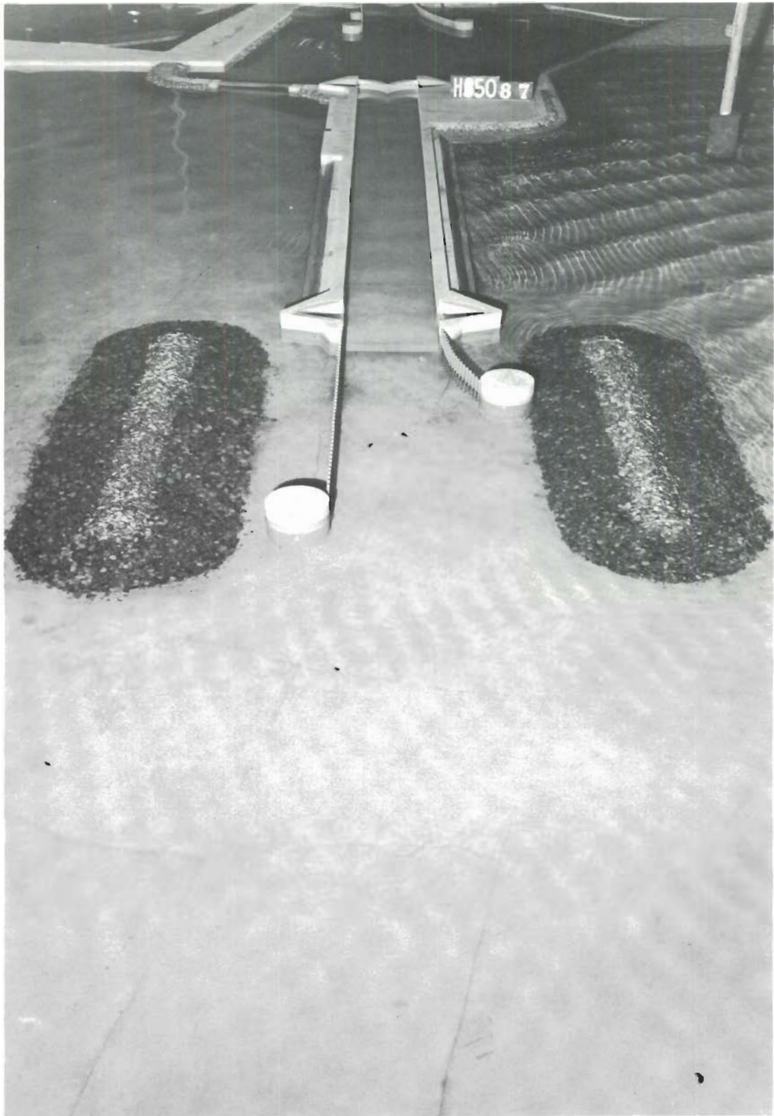
Photo 85. Typical wave patterns at lock entrance for Plan 20A; 4-sec, 4-ft waves from NW; swl = +1 ft msl
