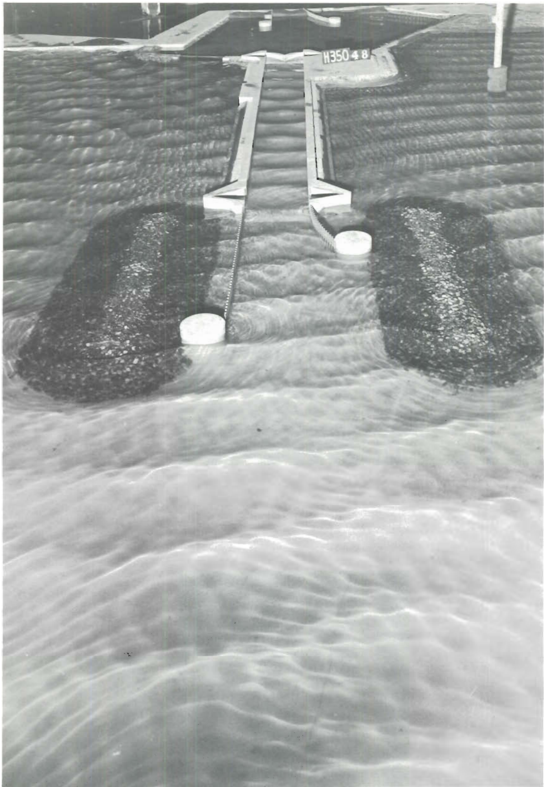
Photo 45. Typical wave patterns at lock entrance for Plan 9; 4-sec, 4-ft waves from NNW; swl = +1 ft msl
