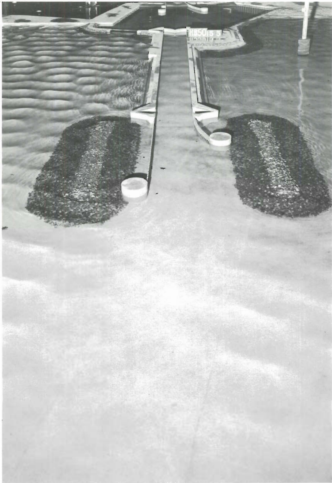
Photo 61. Typical wave patterns at lock entrance for Plan 12A; 4-sec, 5-ft waves from N; swl = +1 ft msl
