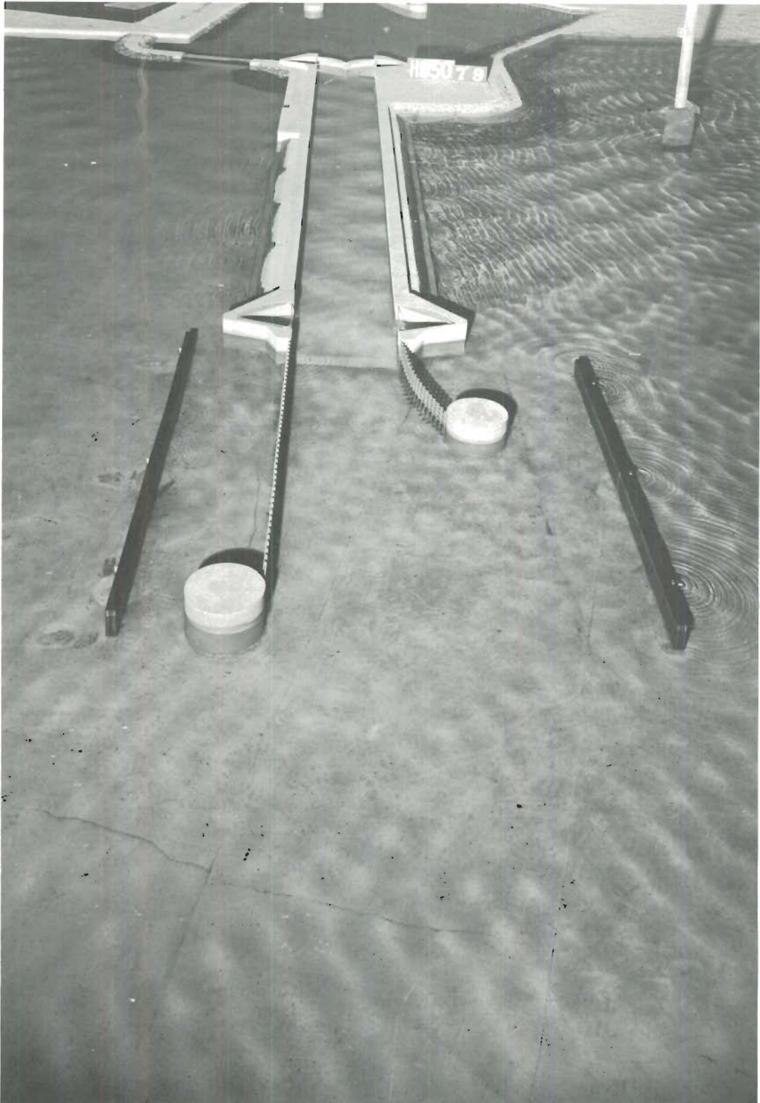
Photo 79. Typical wave patterns at lock entrance for Plan 19F; 4-sec, 4-ft waves from NW; swl = +1 ft msl
