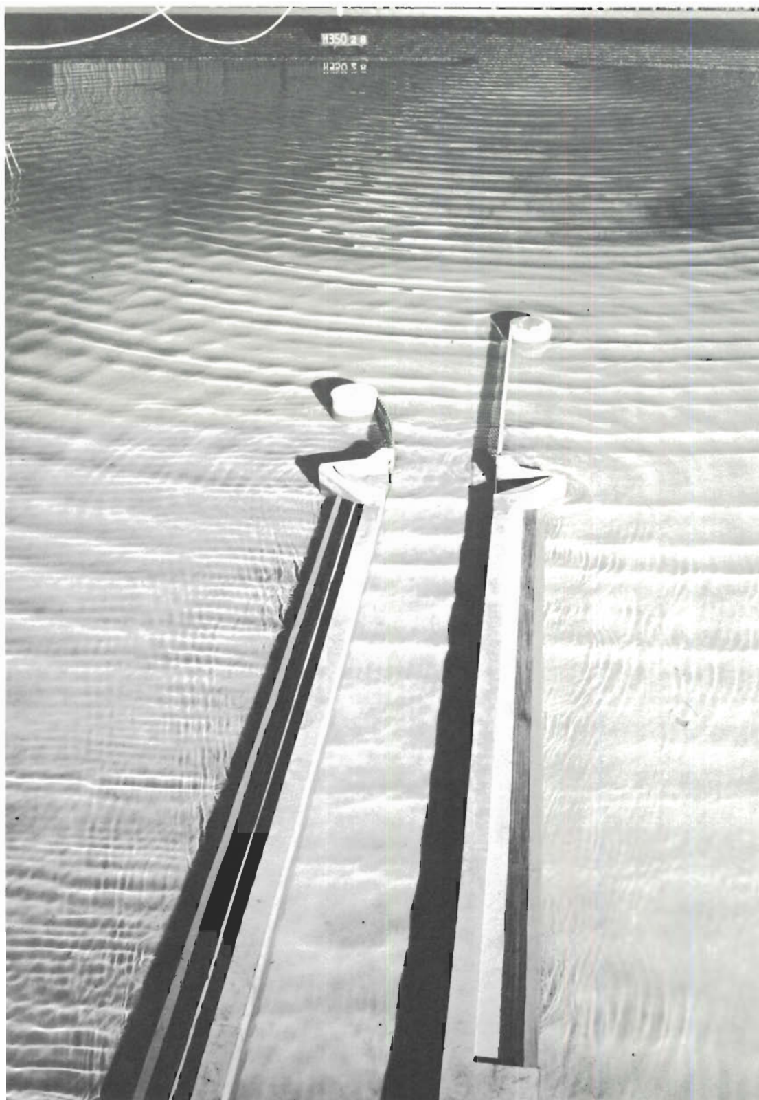
Photo 26. Typical wave patterns for Plan 3A; 3-sec, 4-ft waves from NNW; swl = +1 ft msl
