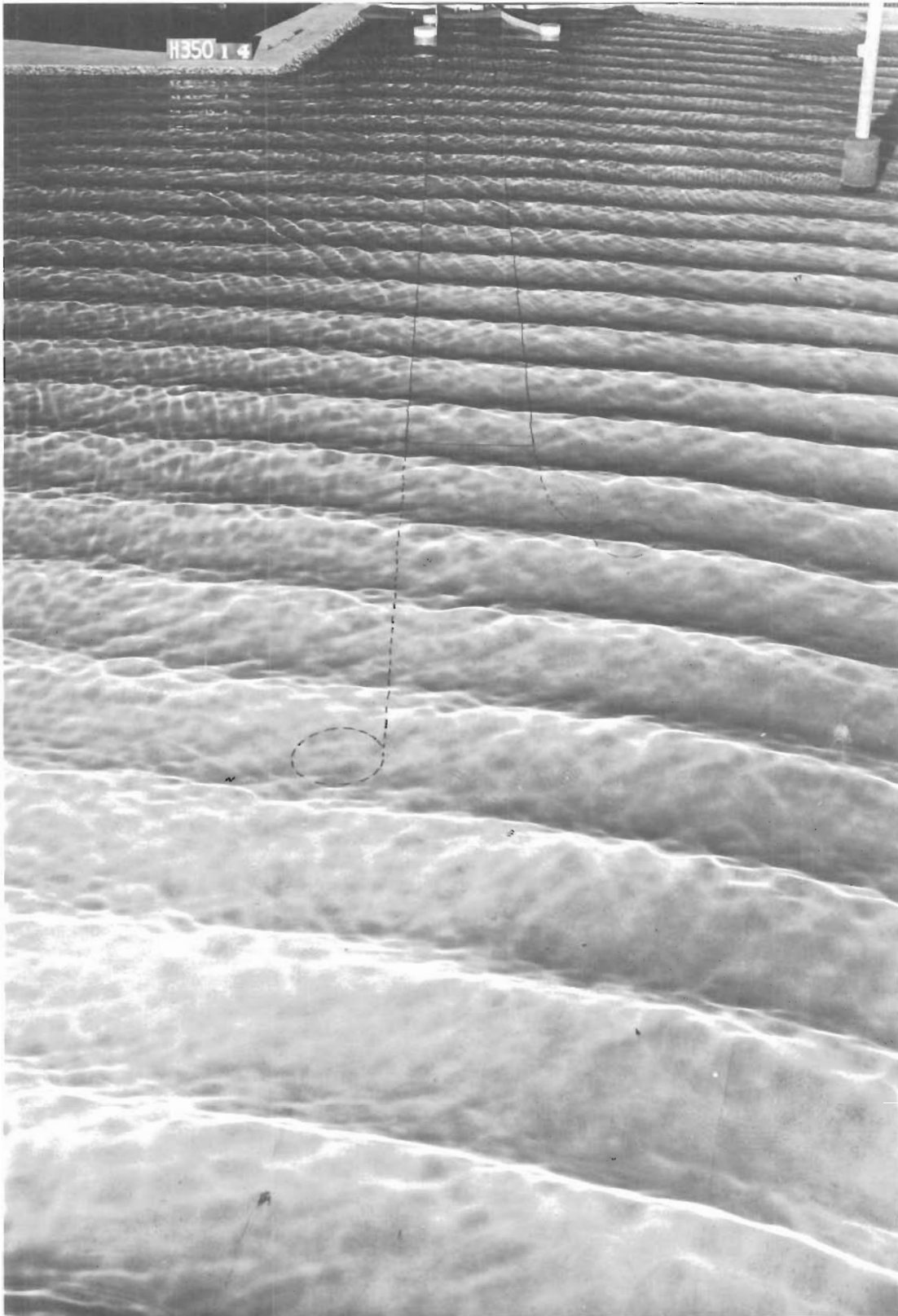
Photo 9. Typical wave patterns for Plan 1; 4-sec, 5-ft waves from N; swl = +1 ft msl
