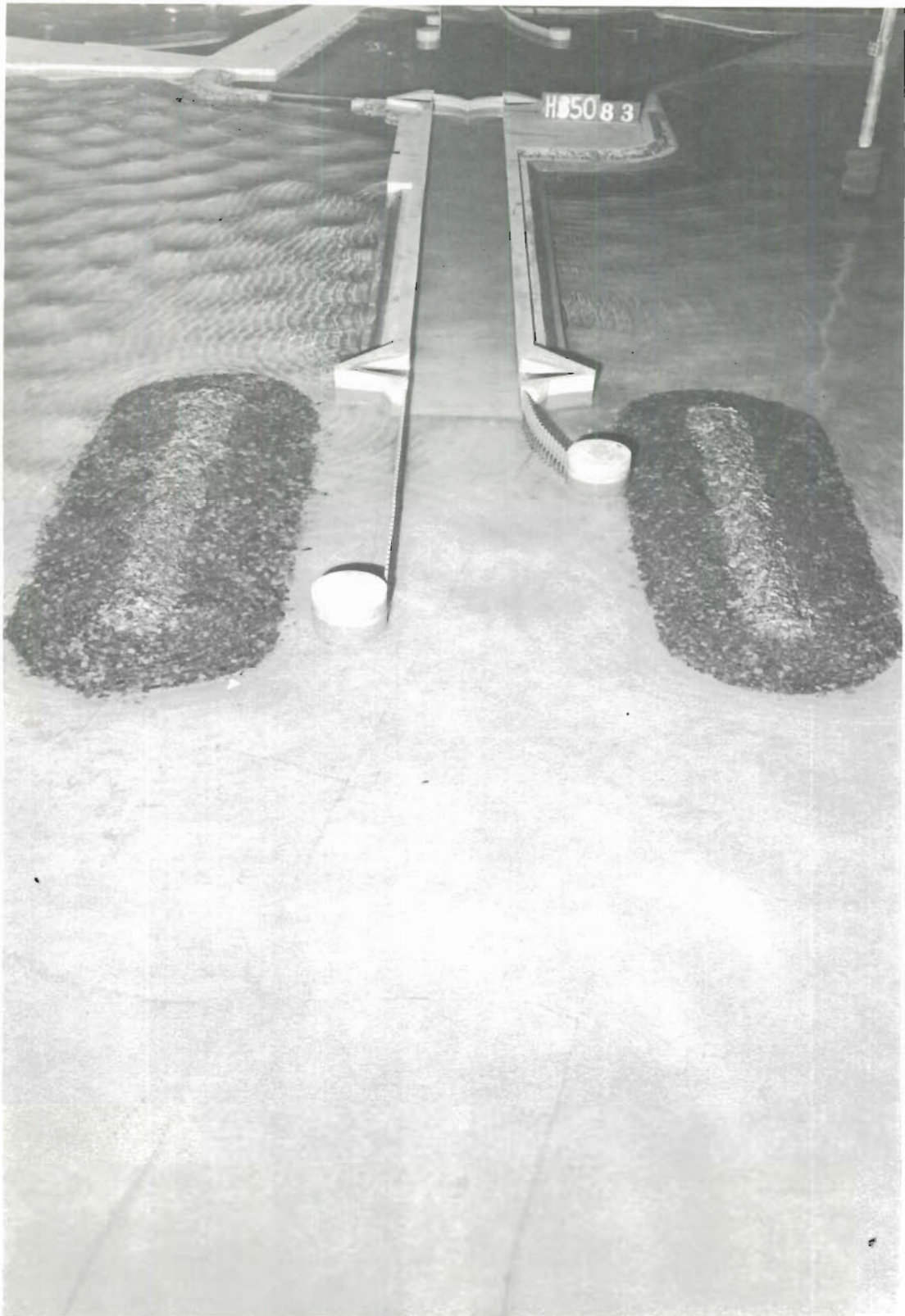
Photo 83. Typical wave patterns at lock entrance for Plan 20A; 4-sec, 4-ft waves from NNW; swl = +1 ft msl
