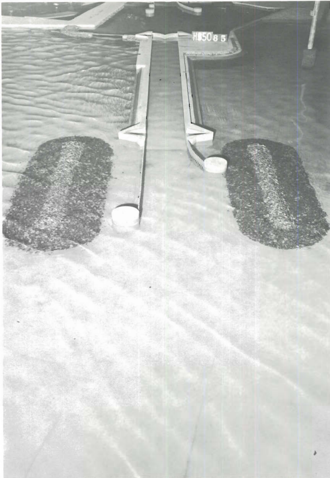
Photo 80. Typical wave patterns at lock entrance for Plan 20A; 3-sec, 4-ft waves from N; swl = +1 ft msl
