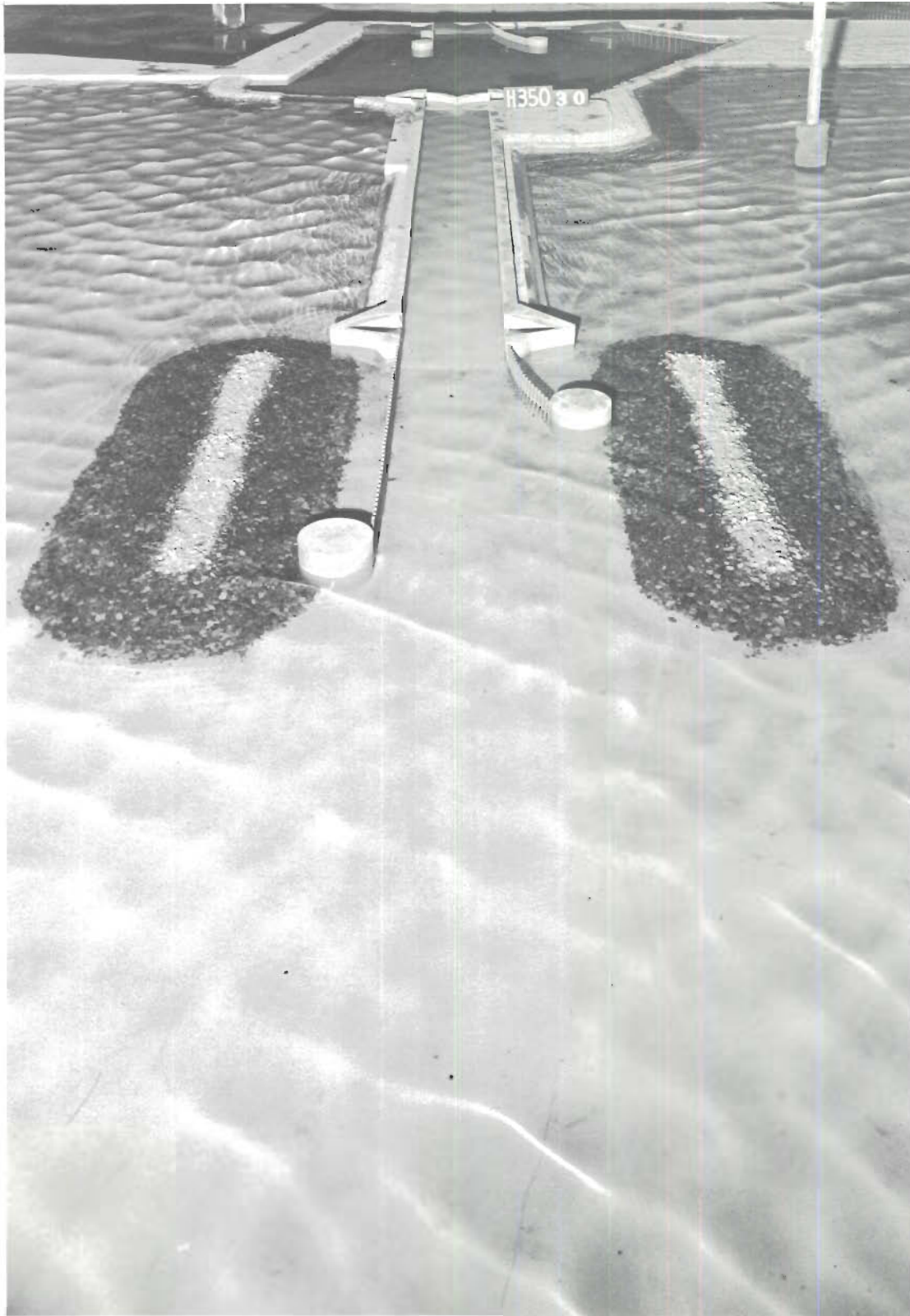
Photo 32. Typical wave patterns at lock entrance for Plan 8; 3-sec 4-ft waves from NNW; swl = +1 ft msl
