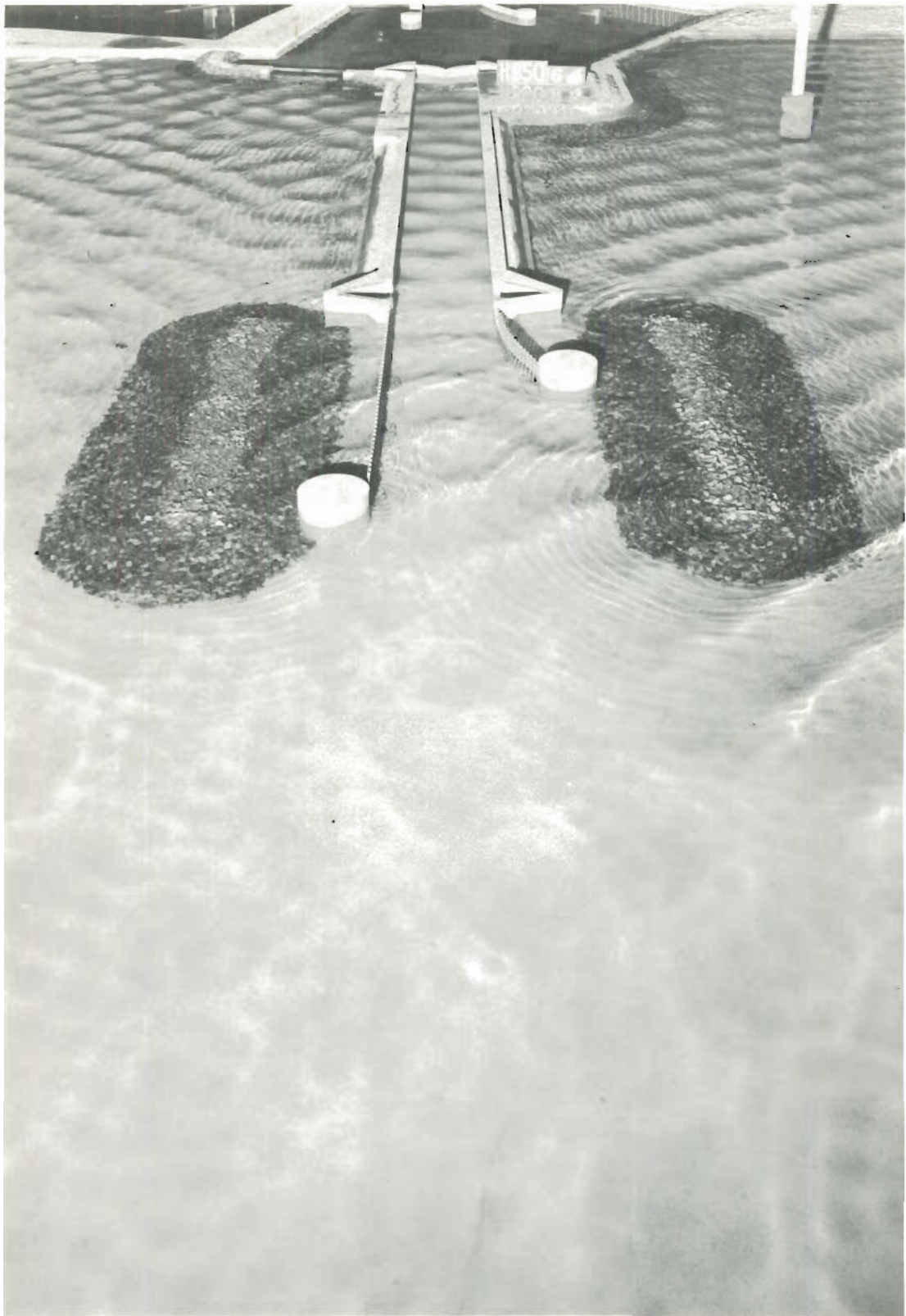
Photo 51. Typical wave patterns at lock entrance for Plan 10A; 4-sec, 4-ft waves from NW; swl = +1 ft msl
