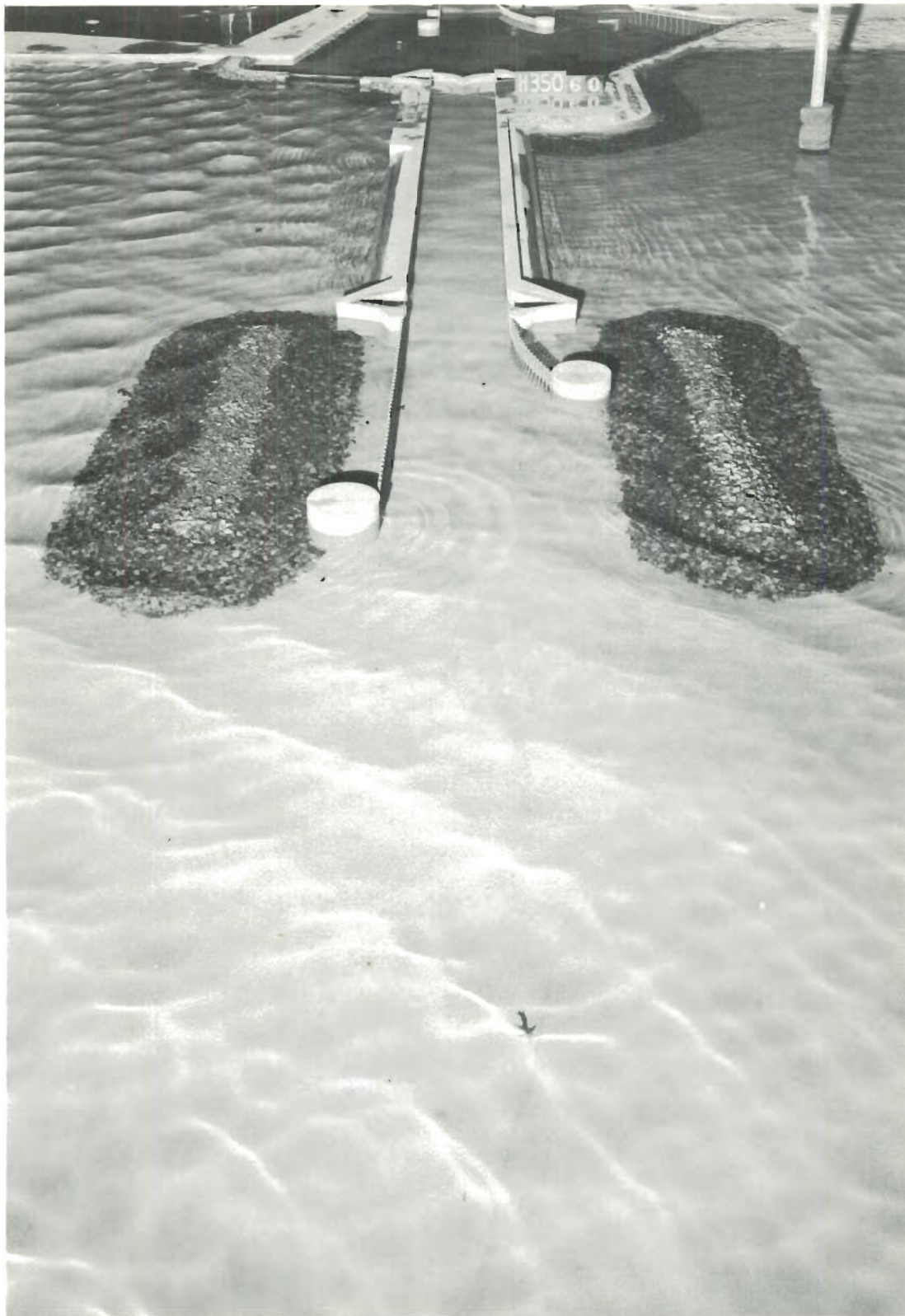
Photo 55. Typical wave patterns at lock entrance for Plan 11B; 4-sec, 5-ft waves from N; swl = +1 ft msl
