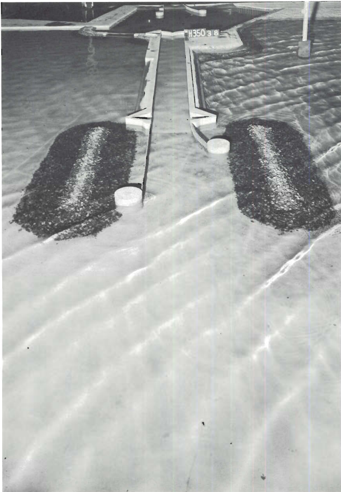
Photo 36. Typical wave patterns at lock entrance for Plan 8; 3-sec, 4-ft waves from NW; swl = +1 ft msl
