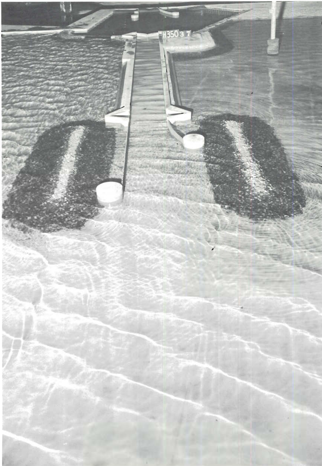
Photo 28. Typical wave patterns at lock entrance for Plan 8; 3-sec, 4-ft waves from N; swl = +1 ft msl
