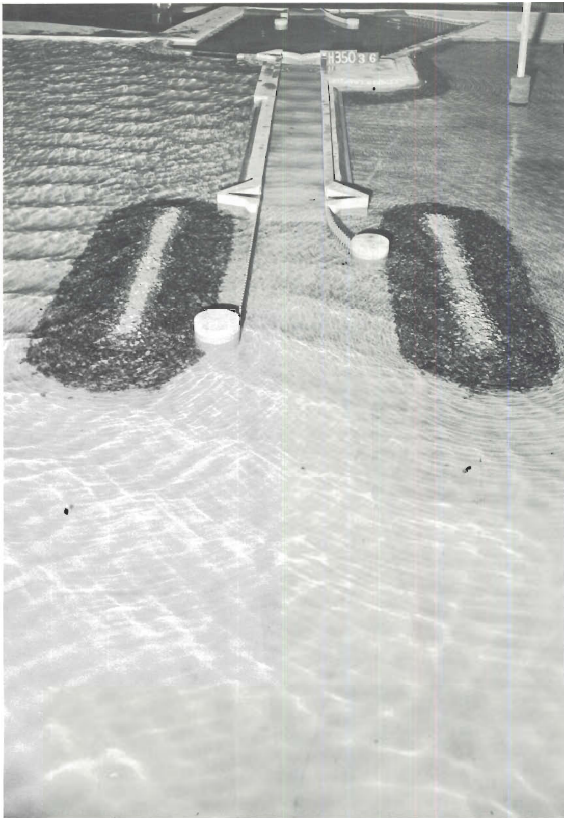
Photo 30. Typical wave patterns at lock entrance for Plan 8; 4-sec, 5-ft waves from N; swl = +1 ft msl
