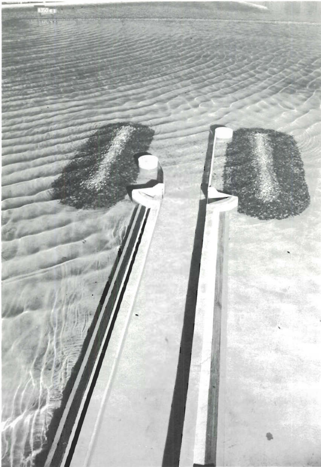
Photo 37. Typical wave patterns for Plan 8; 3-sec, 4-ft waves from NW; swl = +1 ft msl
