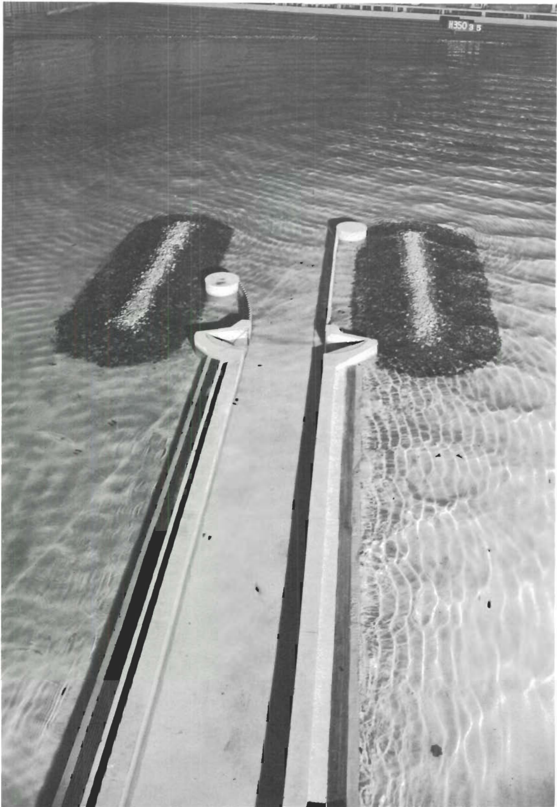
Photo 31. Typical wave patterns for Plan 8; 4-sec, 5-ft waves from N; swl = +1 ft msl
