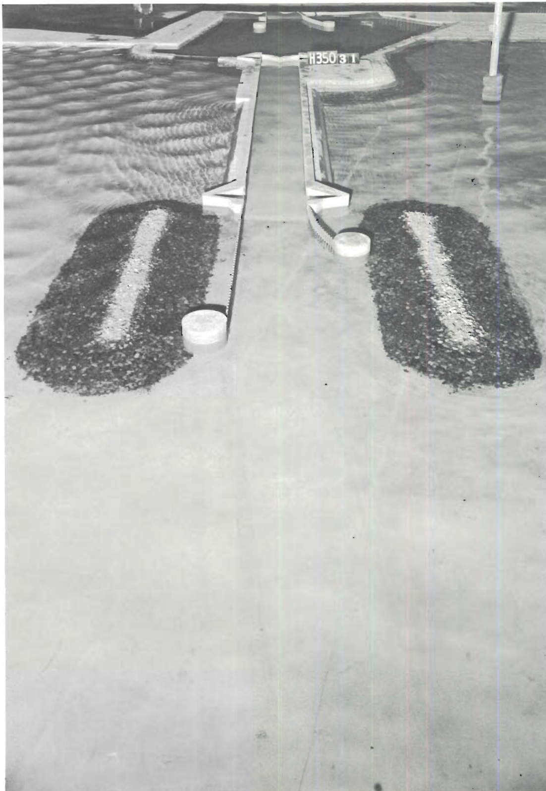
Photo 34. Typical wave patterns at lock entrance for Plan 8; 4-sec, 4-ft waves from NNW; swl = +1 ft msl
