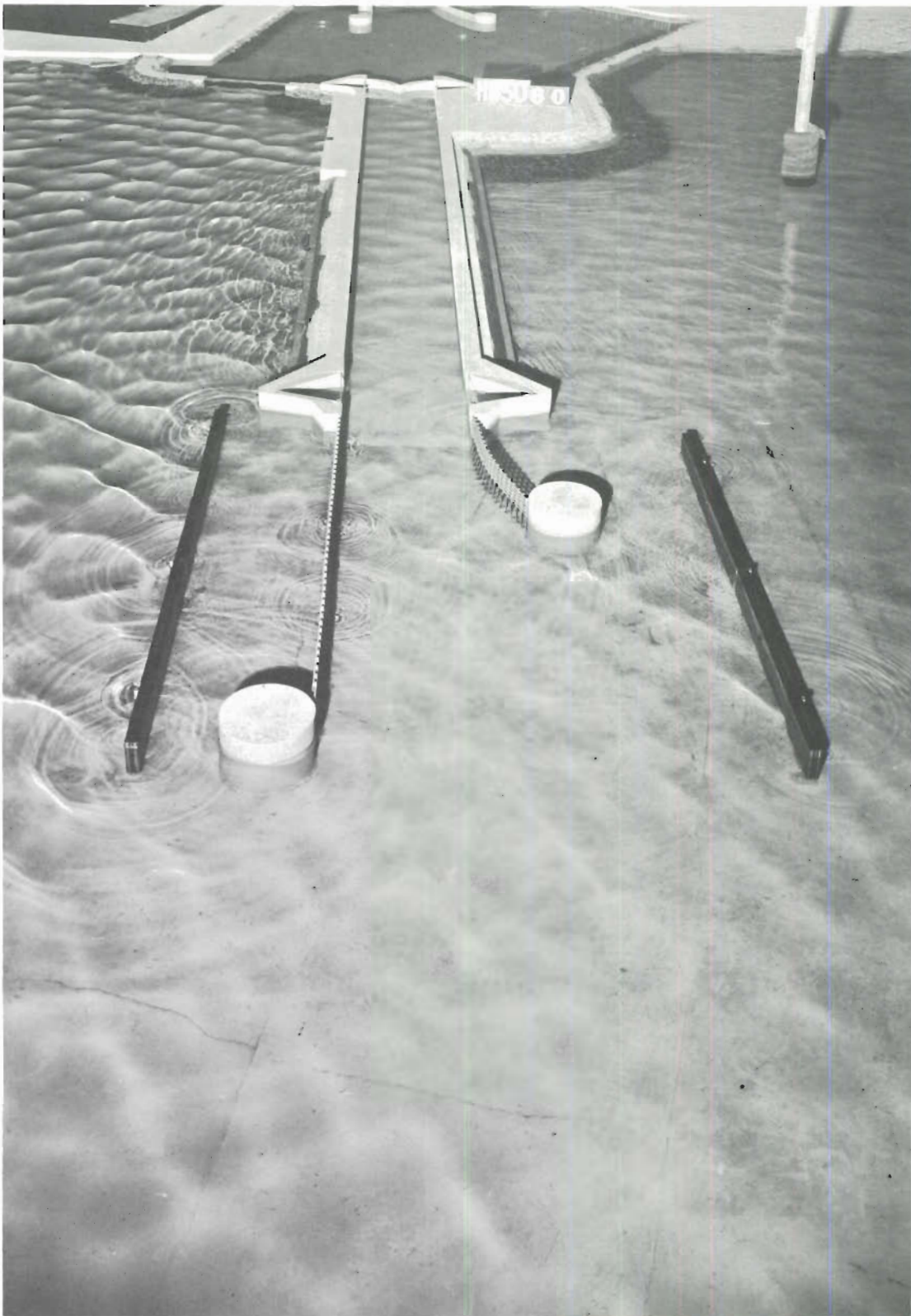
Photo 76. Typical wave patterns at lock entrance for Plan 19F; 3-sec, 4-ft waves from N; swl = +1 ft msl
