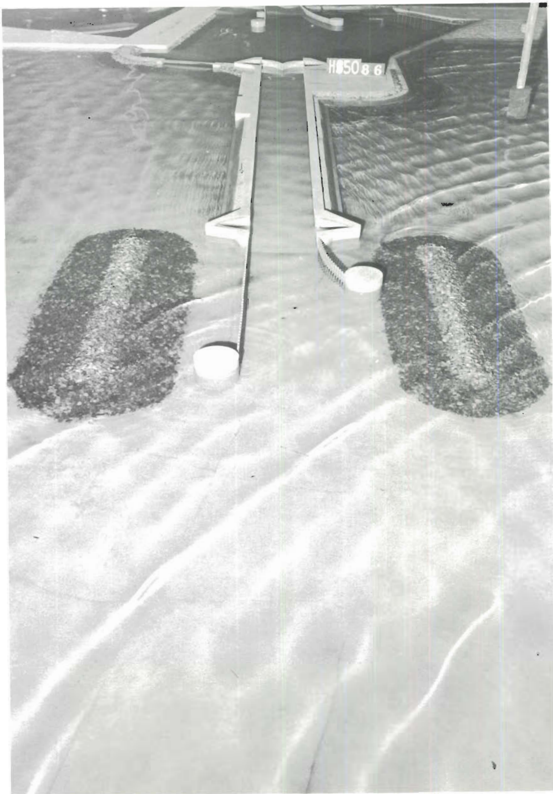
Photo 84. Typical wave patterns at lock entrance for Plan 20A; 3-sec, 4-ft waves from NW; swl = +1 ft msl
