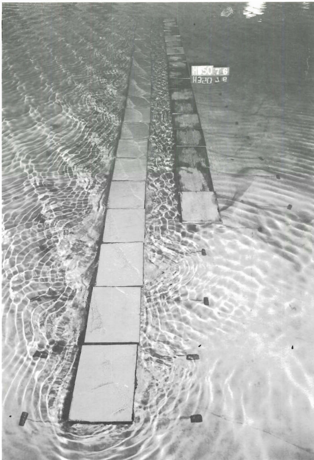
Photo 75. Typical wave patterns at breakwater for Plan 17C; 4-sec, 4-ft waves from NW; swl = +4 ft msl
