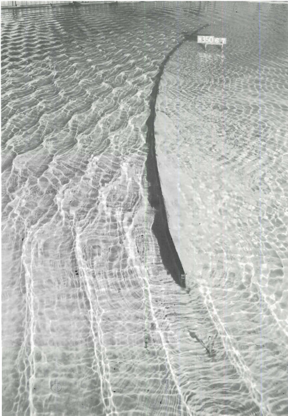
Photo 60. Typical wave patterns at breakwater for Plan 11B; 4-sec, 4-ft waves from NW; swl = +4 ft msl
