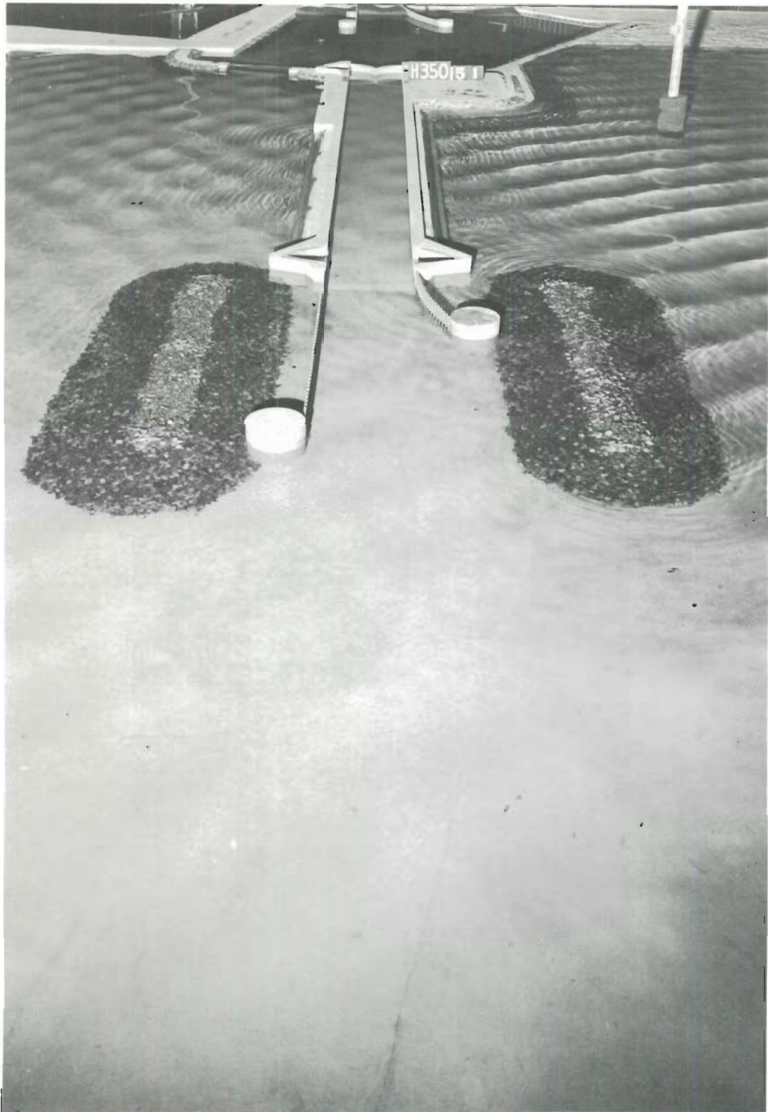
Photo 63. Typical wave patterns at lock entrance for Plan 12A; 4-sec, 4-ft waves from NW; swl = +1 ft msl
