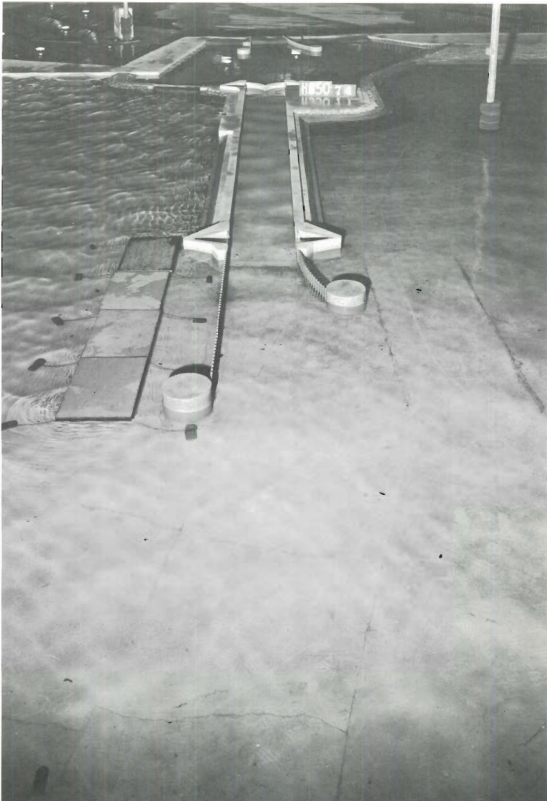
Photo 67. Typical wave patterns at lock entrance for Plan 17C; 4-sec, 5-ft waves from N; swl = +1 ft msl
