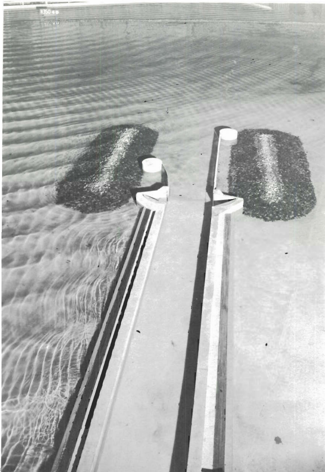
Photo 39. Typical wave patterns for Plan 8; 4-sec, 4-ft waves from NW; swl = +1 ft msl
