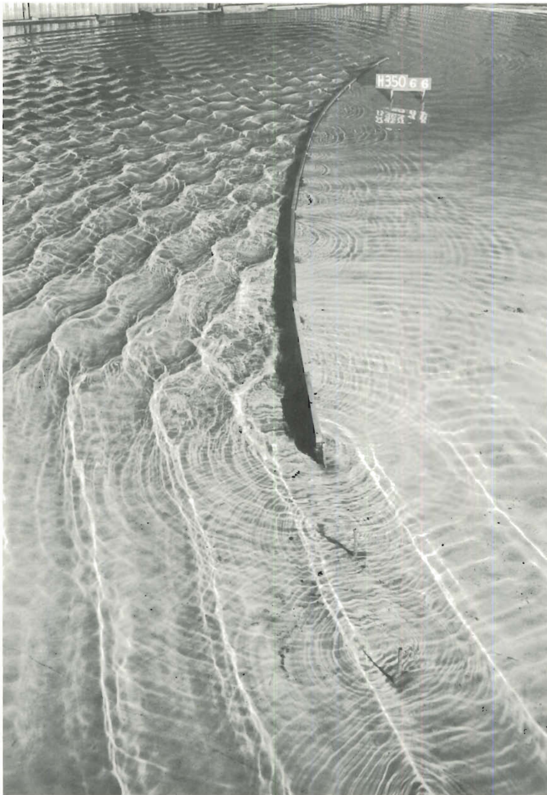
Photo 54. Typical wave patterns at breakwater for Plan 10A; 4-sec, 4-ft waves from NW; swl = +4 ft msl
