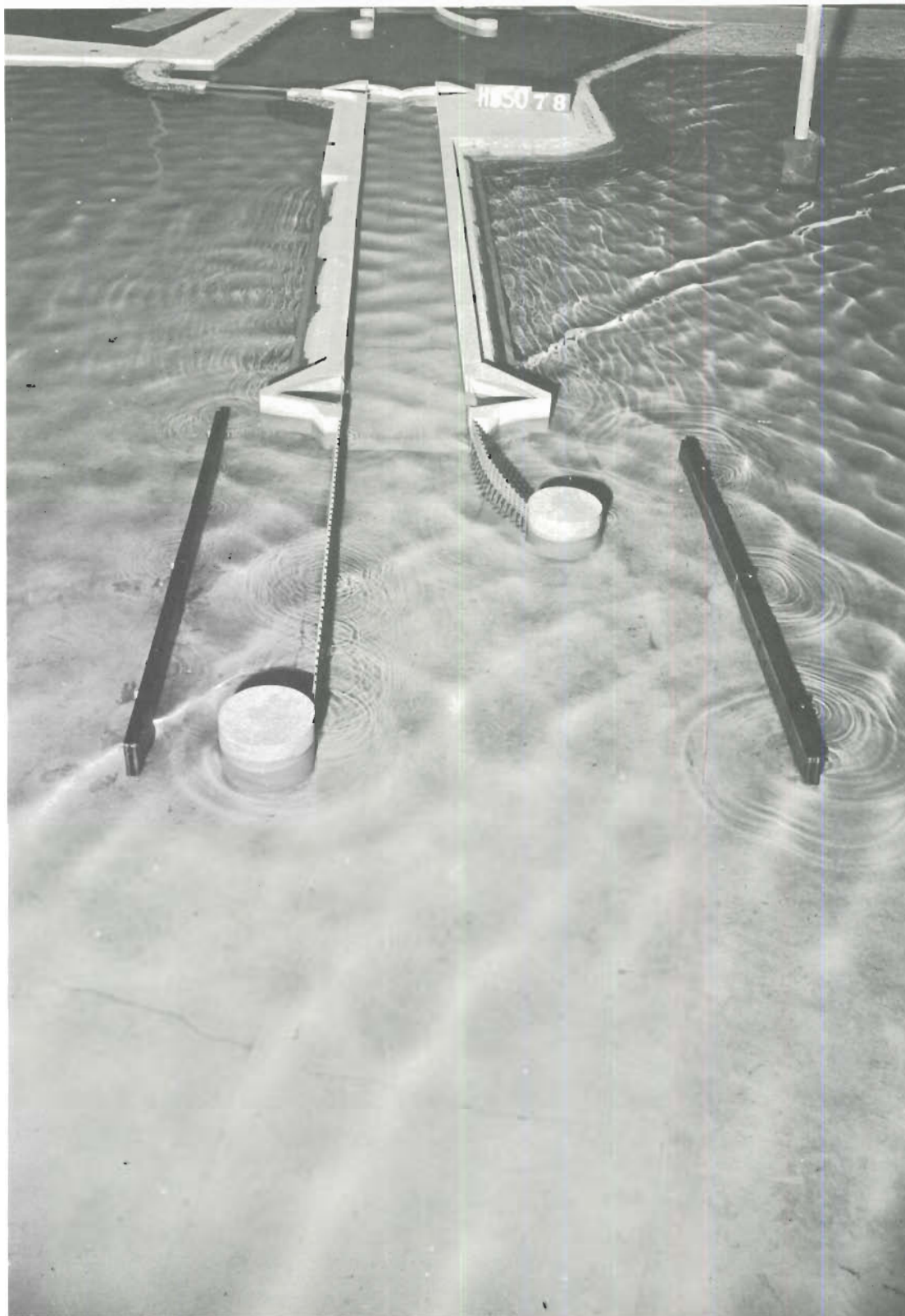
Photo 78. Typical wave patterns at lock entrance for Plan 19F; 3-sec, 4-ft waves from NW; swl = +1 ft msl
