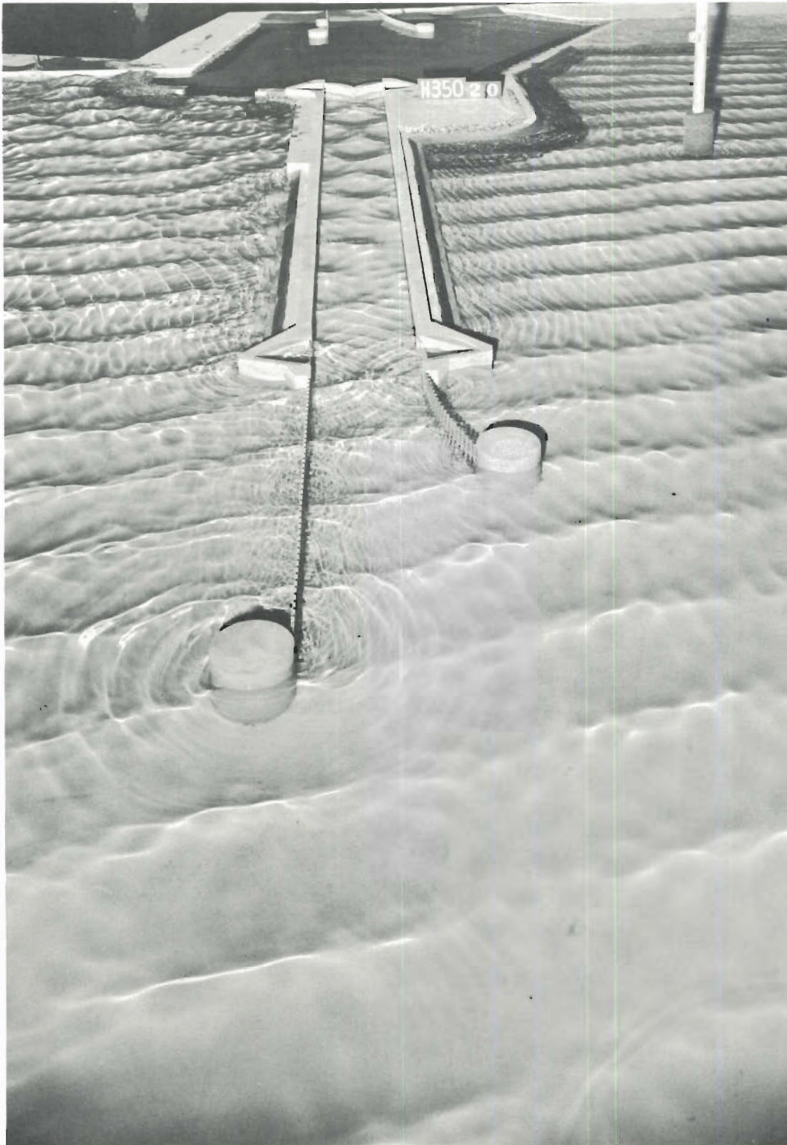
Photo 18. Typical wave patterns at lock entrance for Plan 2; 4-sec, 4-ft waves from NNW; swl = +1 ft msl
