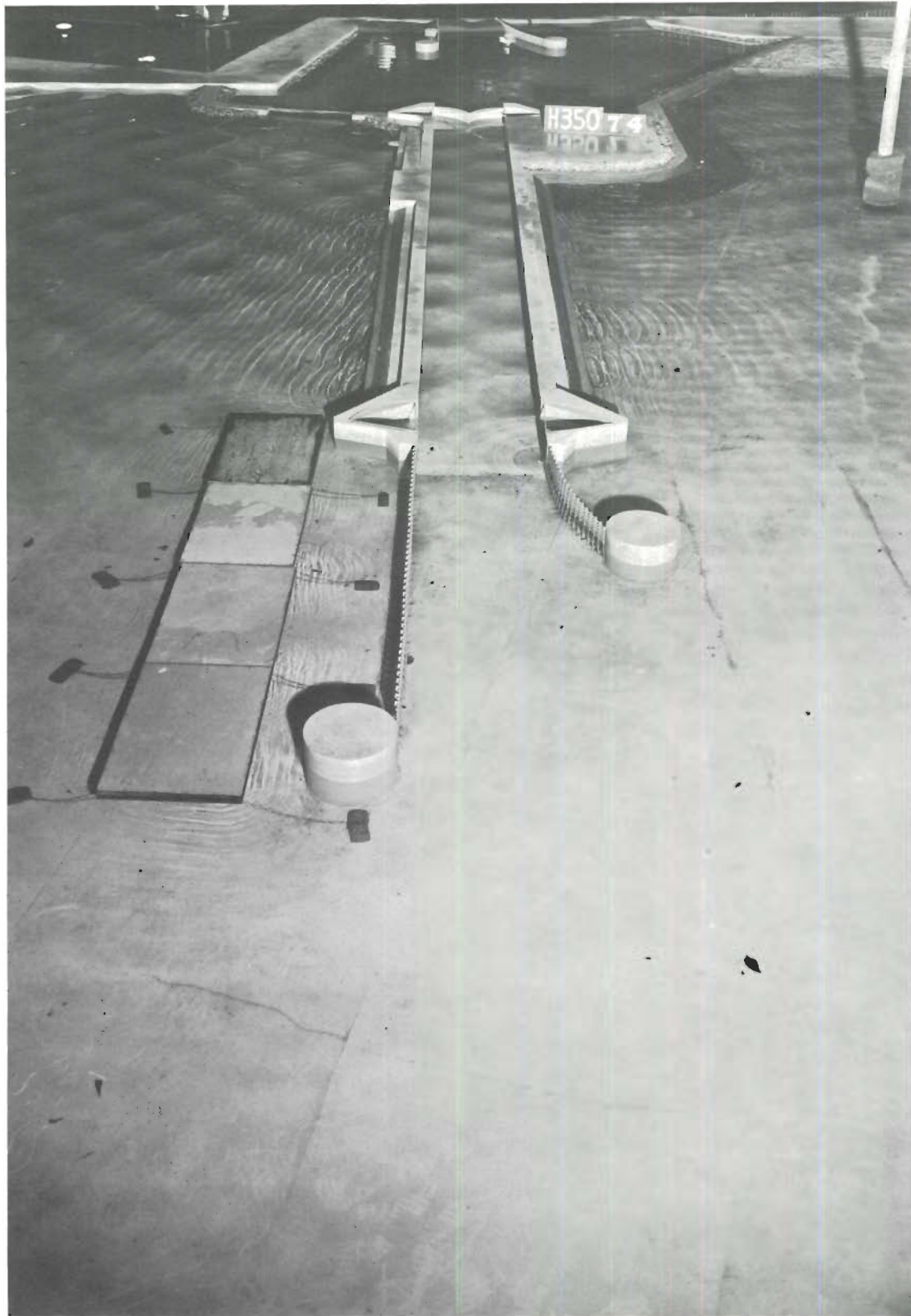
Photo 72. Typical wave patterns at lock entrance for Plan 17C; 4-sec, 4-ft waves from NW; swl = +1 ft msl
