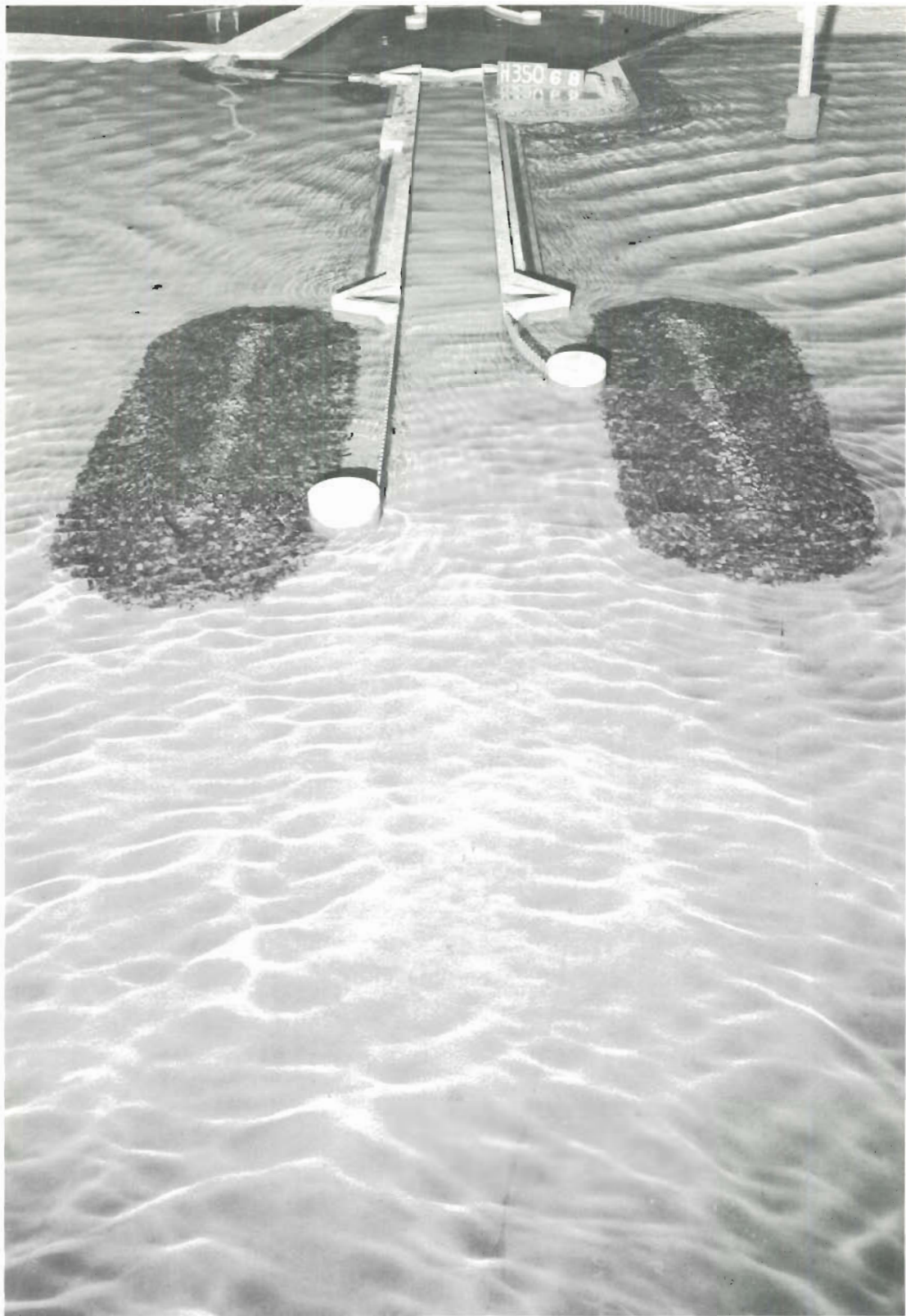
Photo 59. Typical wave patterns at lock entrance for Plan 11B; 4-sec, 4-ft waves from NW; swl = +4 ft msl
