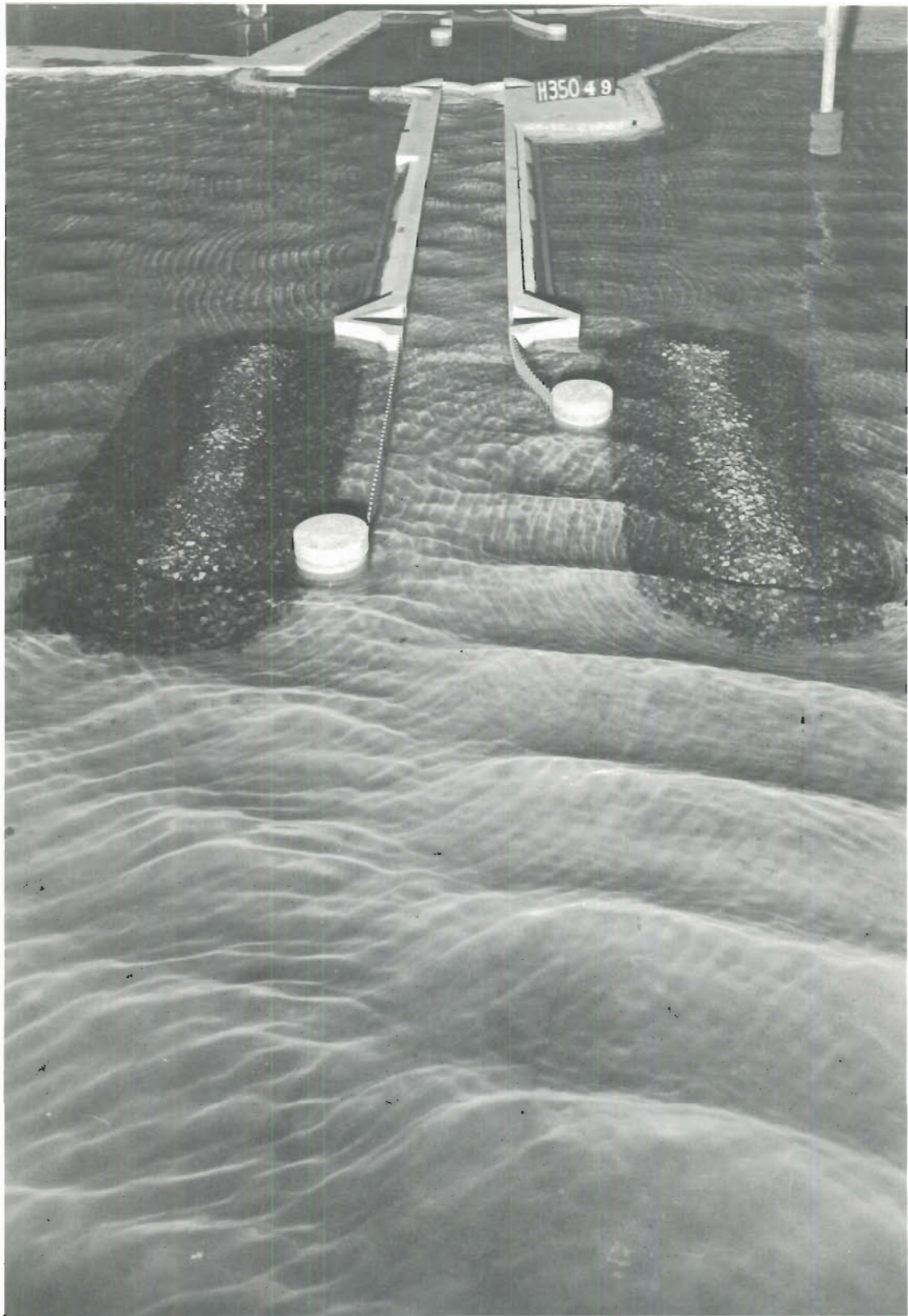
Photo 43. Typical wave patterns at lock entrance for Plan 9; 4-sec, 5-ft waves from N; swl = +1 ft msl
