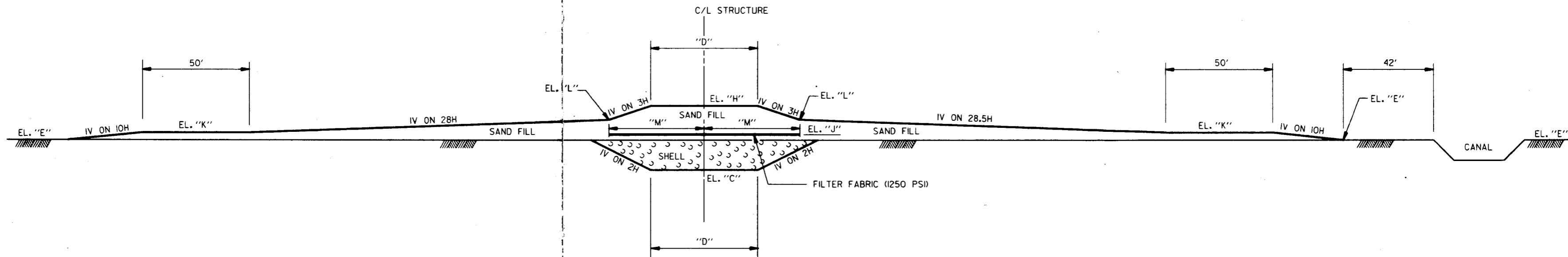
TYPICAL PRELOAD SECTION ALONG CL LEVEL
