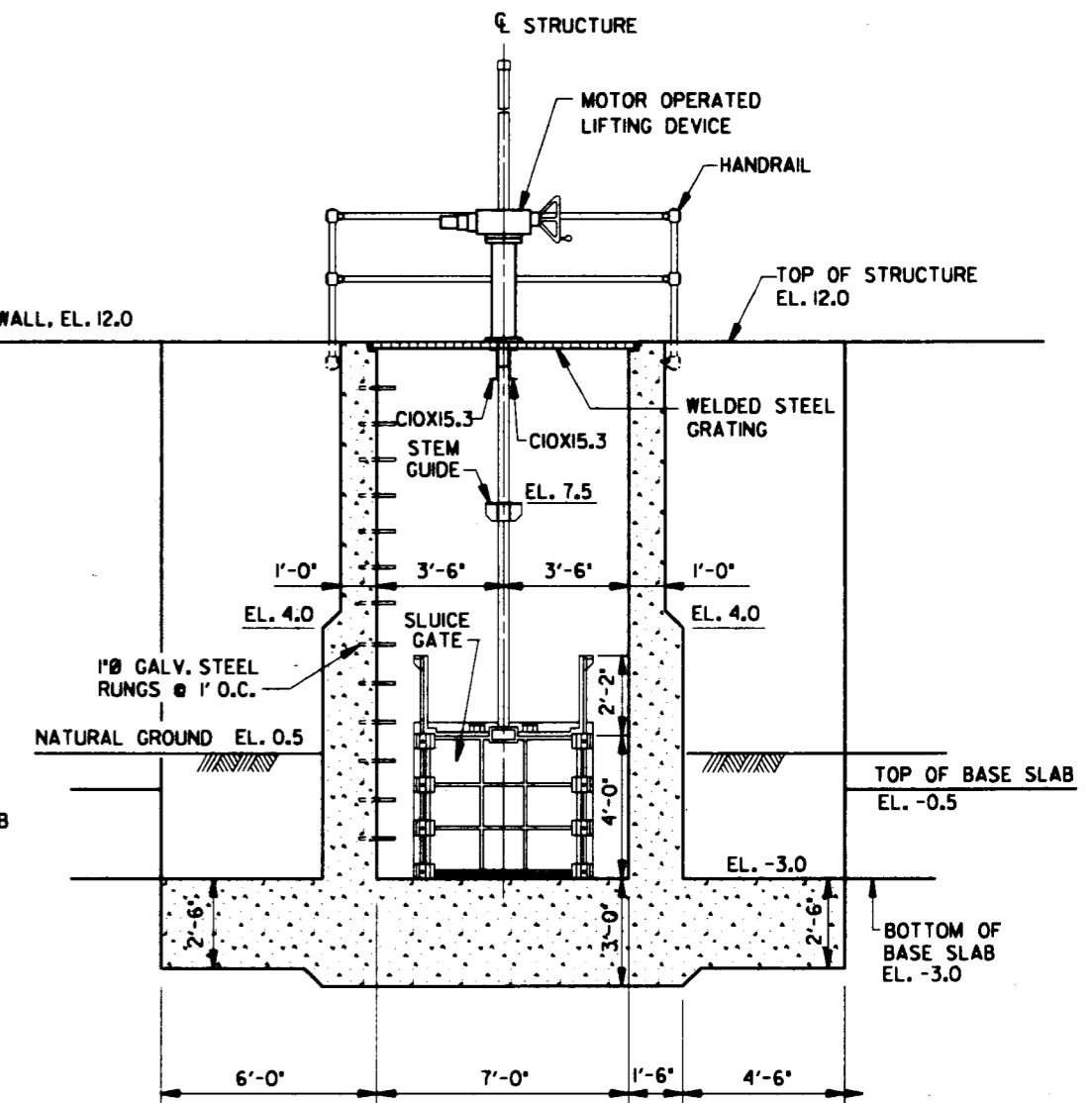
SECTIONAL ELEVATION PARISH LINE CANAL DRAINAGE STRUCTURE
