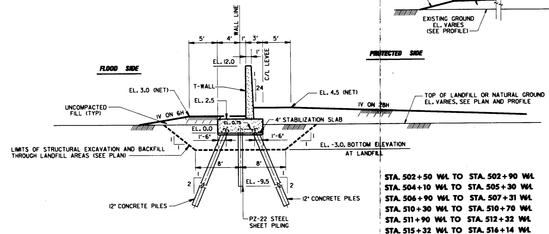
TYPICAL SECTIONS
