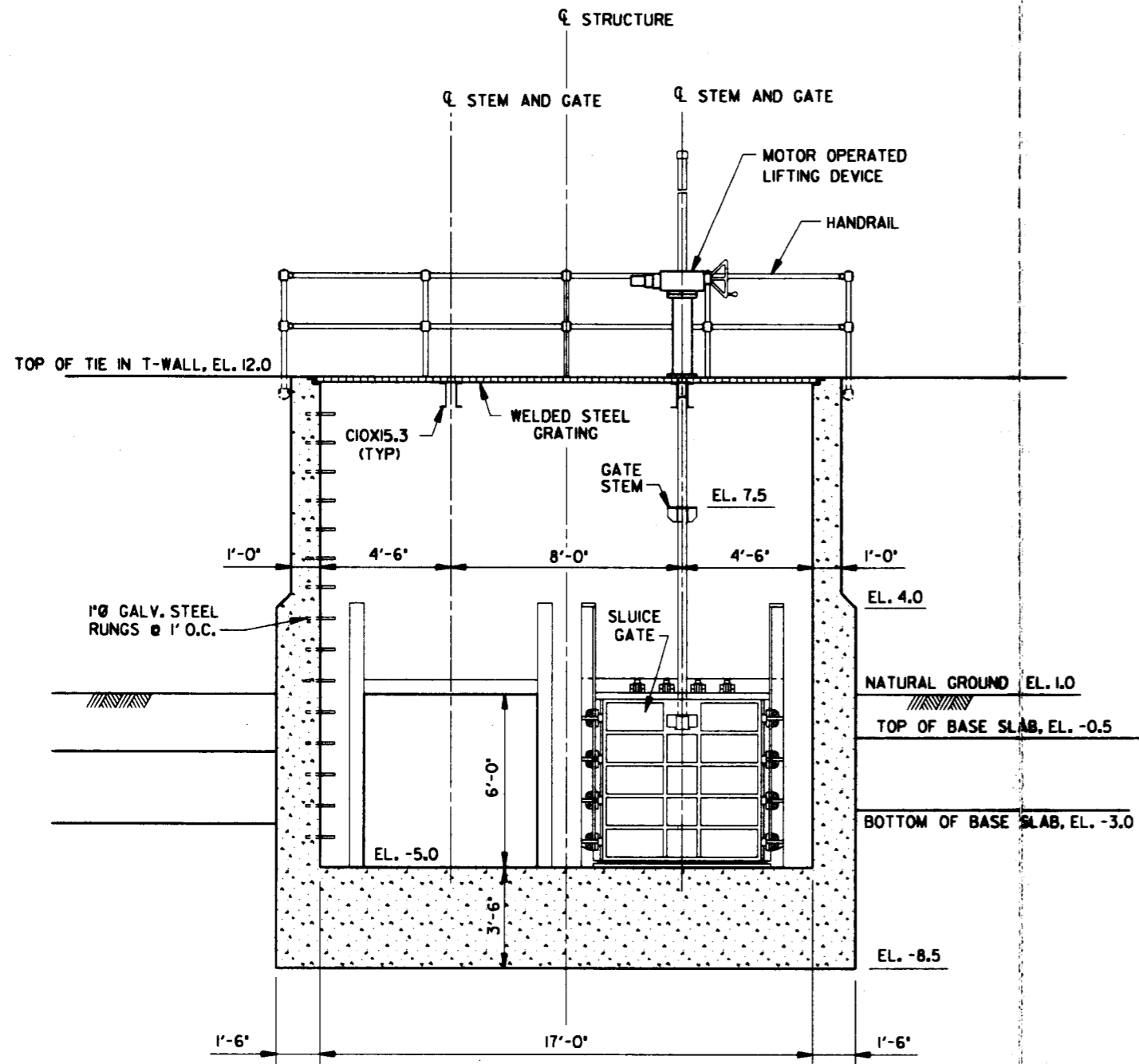
SECTIONAL ELEVATION ST. ROSE DRAINAGE STRUCTURE
