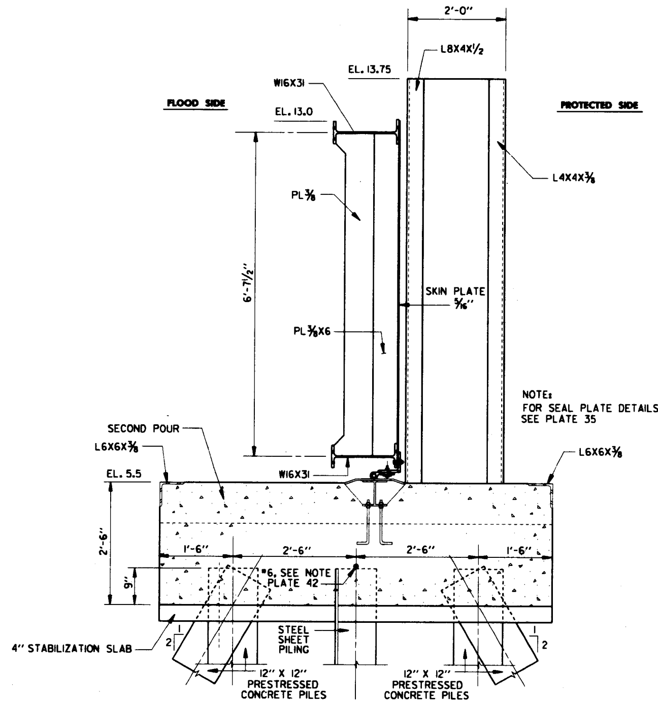
TYPICAL SECTION SCALE: 1" = 1'-0"
