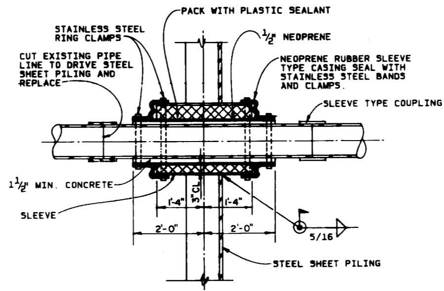
SECTION B TYPICAL GAS PIPE THRU STEEL SHEET PILING SCALE: 3/4" = 1'-0"
