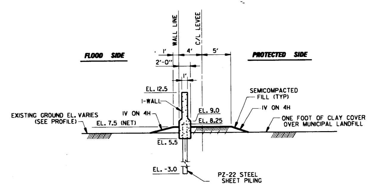
TYPICAL SECTION STA. 500+59 WL TO STA. 501+30 WL
