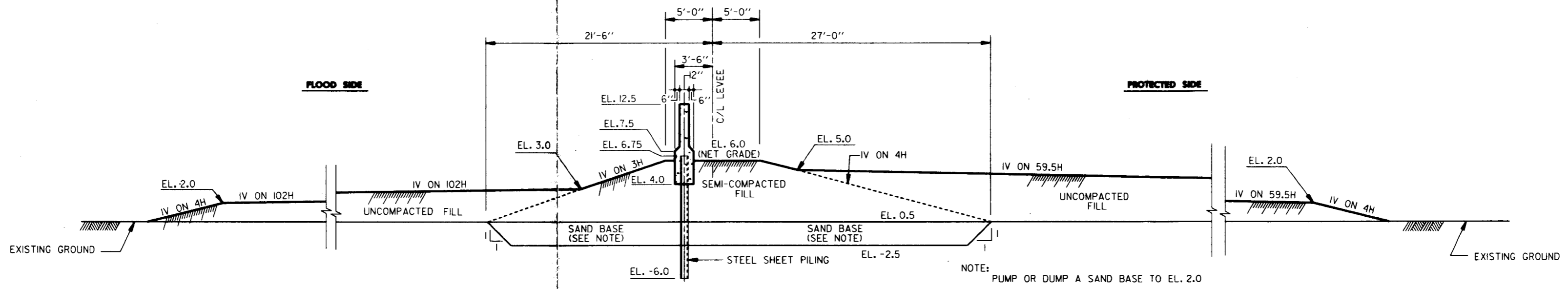
TYPICAL I-WALL SECTION (ALTERNATE PLAN)
