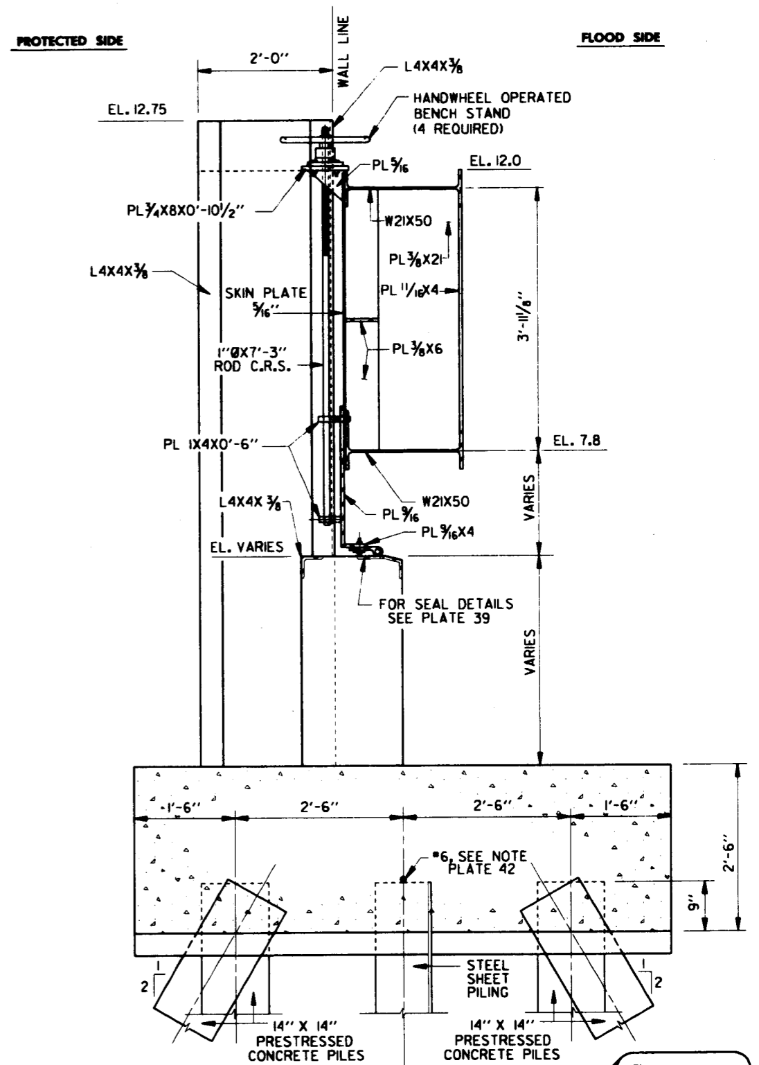
TYPICAL SECTION SCALE: 1" = 1'-0"
