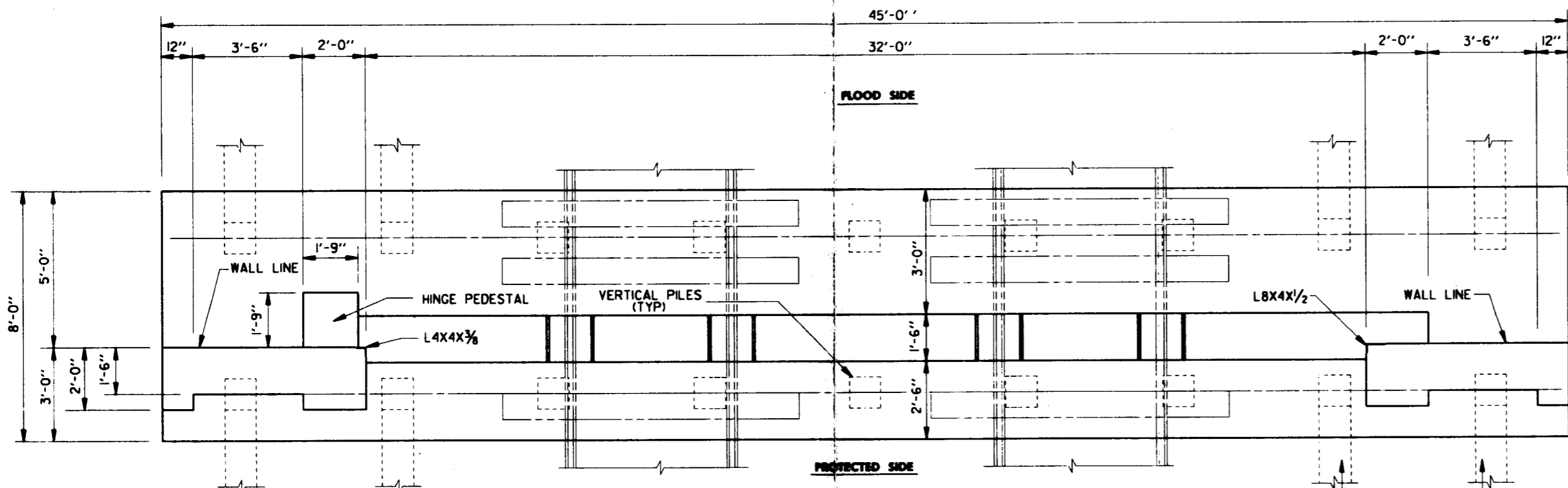
PLAN AT EL. 18.0 SCALE: 1/2" = 1'-0"
