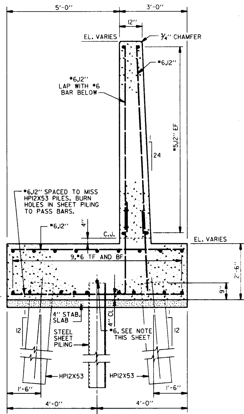
TYPICAL WING WALL SECTION AT SLUICE GATE STRUCTURES SCALE: 3/4" = 1'-0"
