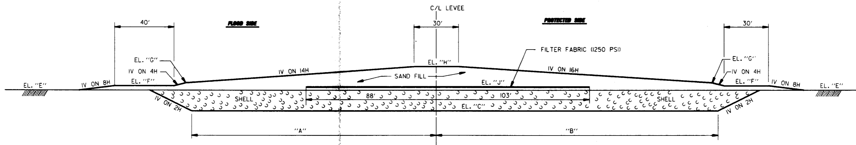
TYPICAL PRELOAD SECTION THRU CL STRUCTURE
