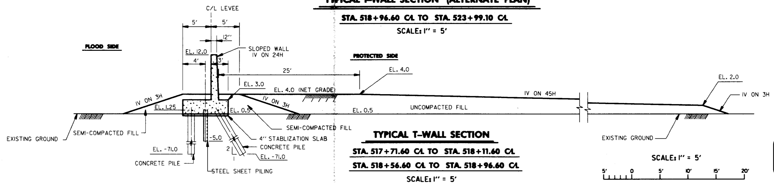
TYPICAL I-WALL SECTION (ALTERNATE PLAN)
