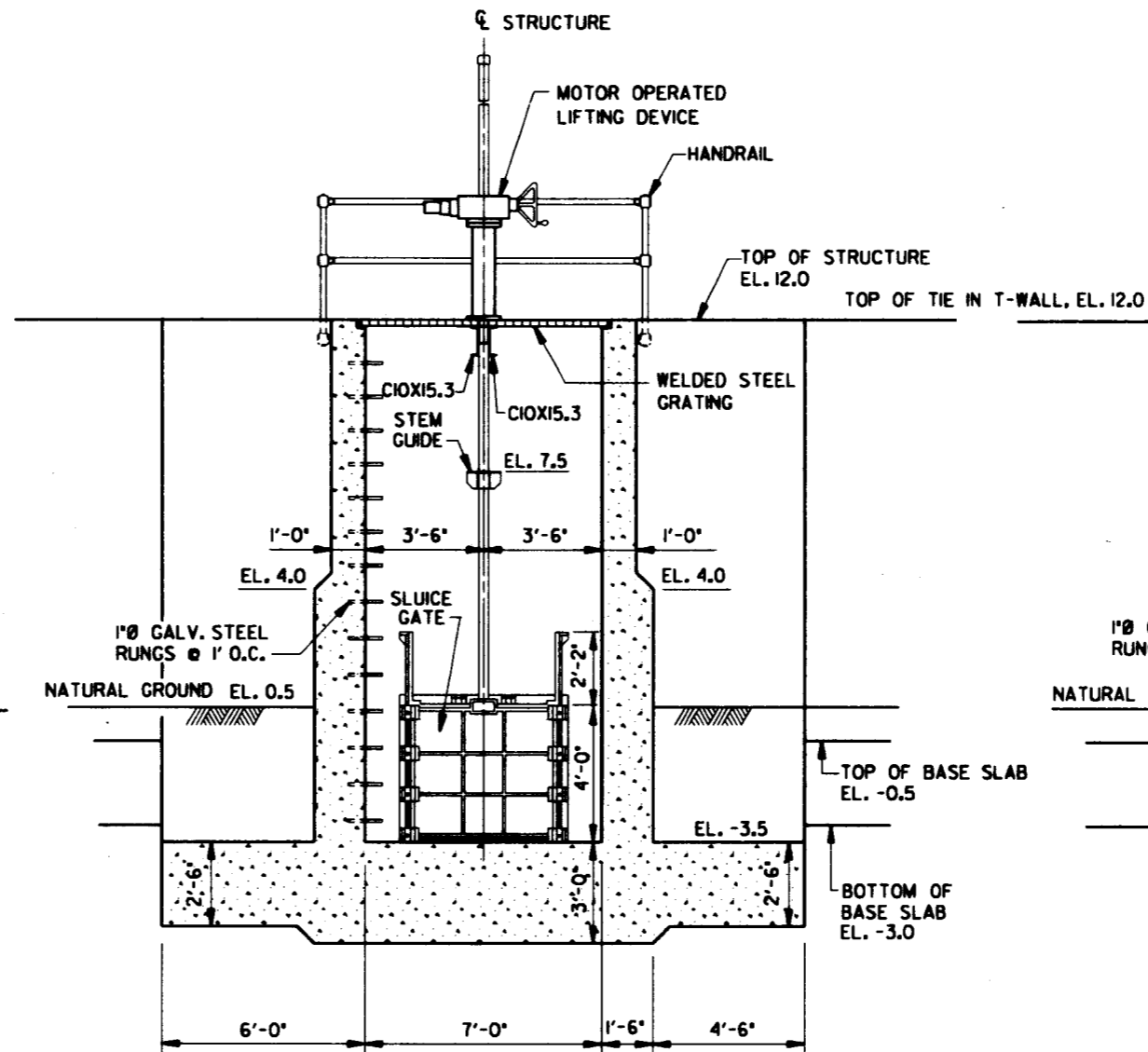
SECTIONAL ELEVATION WALKER CANAL DRAINAGE STRUCTURE
