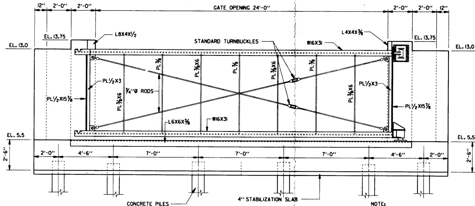
FLOOD SIDE ELEVATION SCALE: 1/2" = 1'-0"
