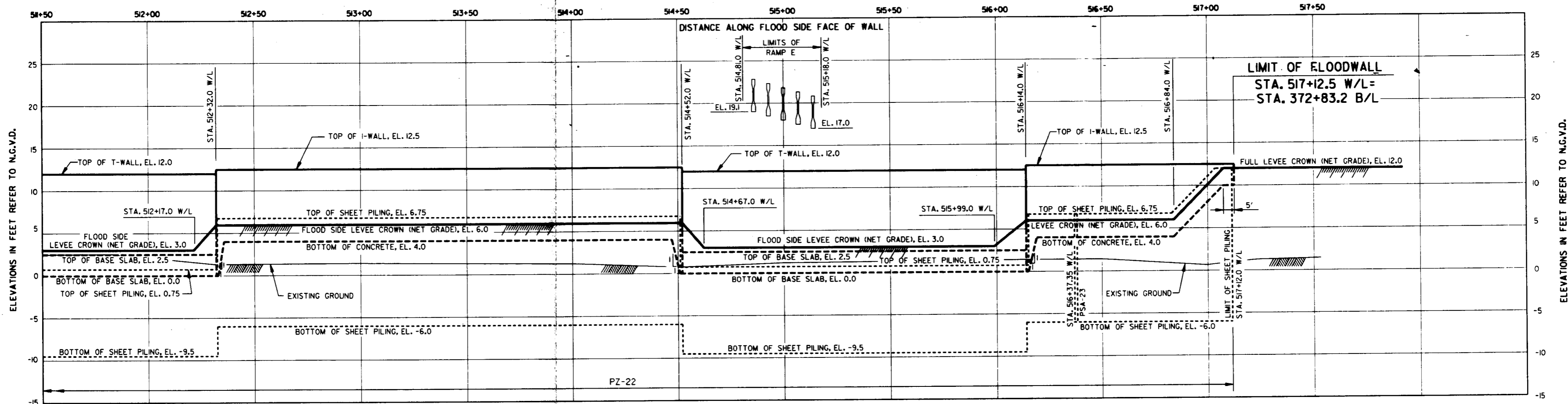
PROFILE SCALE: HOR. 1" = 20' VERT. 1" = 5'
