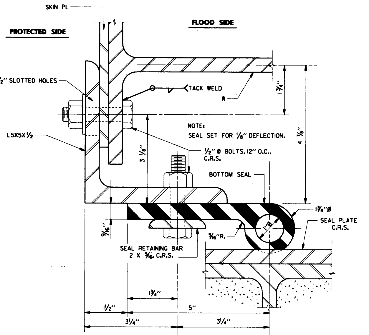
SECTION THRU BOTTOM SEAL SCALE: FULL SIZE
