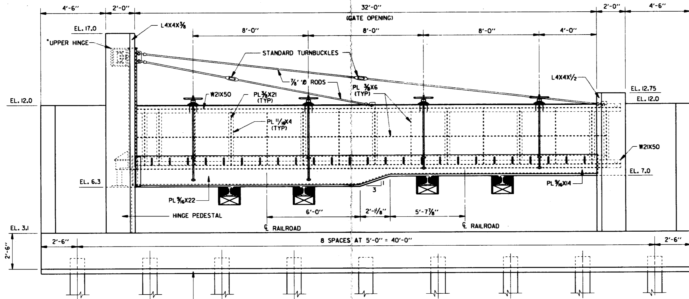
PROTECTED SIDE ELEVATION SCALE: 1/2" = 1'-0"
