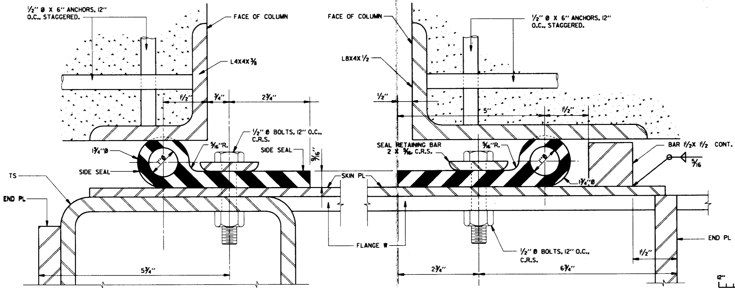
DETAIL 2
