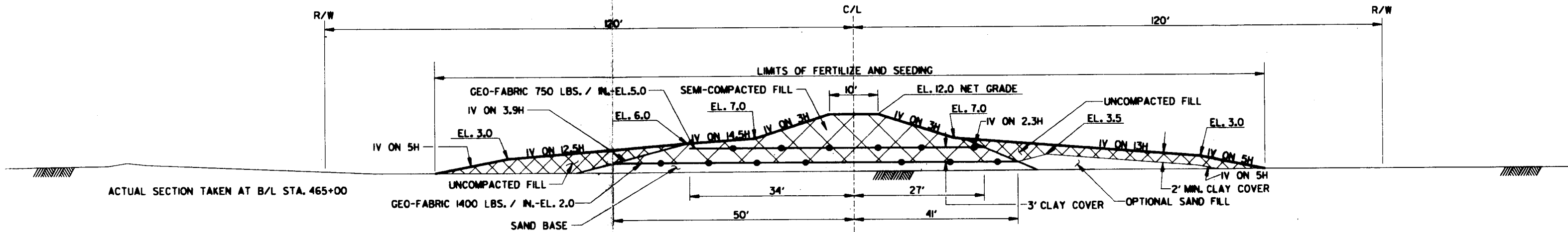
TYPICAL DESIGN SECTION VII NOT TO SCALE C/L STA. 430+00 TO STA. 439+75 C/L STA. 450+50 TO STA. 470+00 (500' TRANSITION FROM STA. 470+00 TO 475+00)
