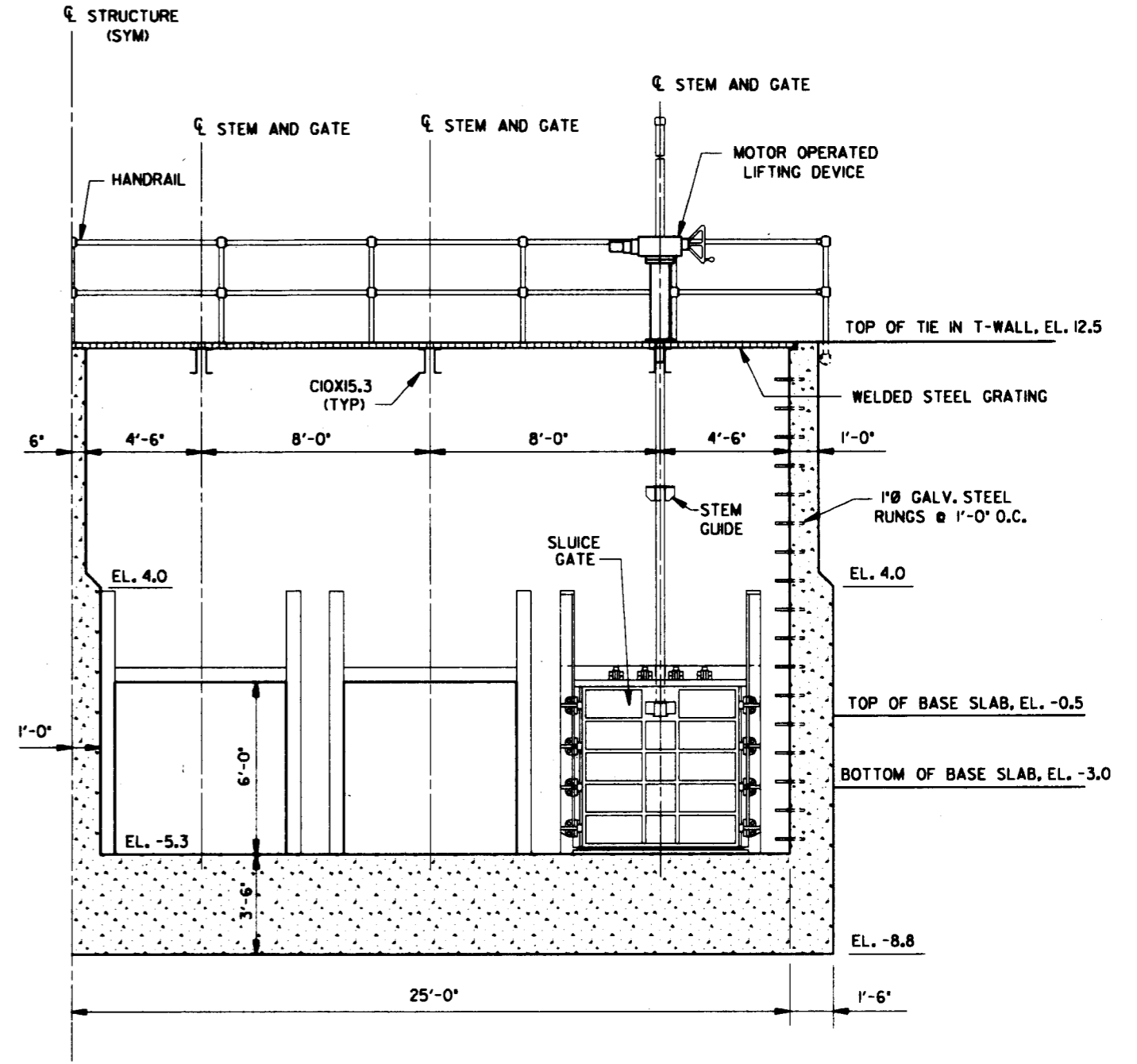
SECTIONAL ELEVATION CROSS BAYOU DRAINAGE STRUCTURE
