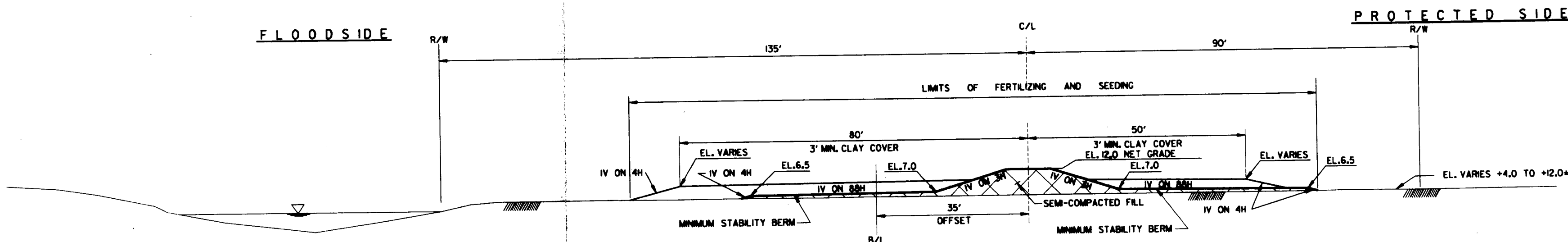
TYPICAL LANDFILL SECTION XV C/L STA. 440+75 TO STA. 449+50 (NOT-CONTINUOUS) NOT TO SCALE
