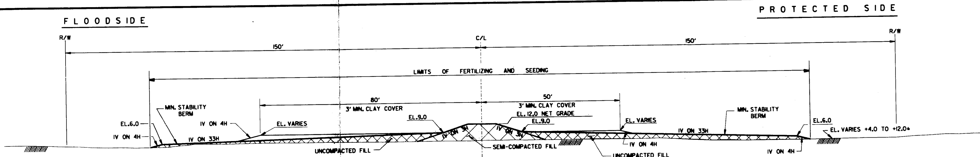
TYPICAL LANDFILL SECTION XIV C/L STA. 331+05 TO STA. 356+32 (NOT-CONTINUOUS) NOT TO SCALE
