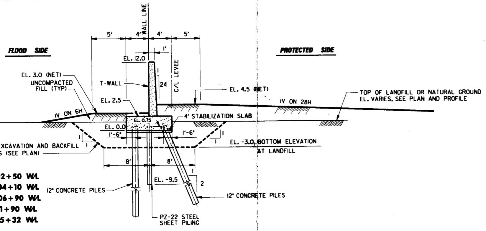
TYPICAL SECTIONS
