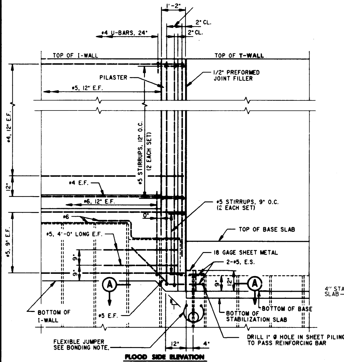
REINFORCEMENT - I-WALL TO T-WALL SCALE: 3/4" = 1'-0"
