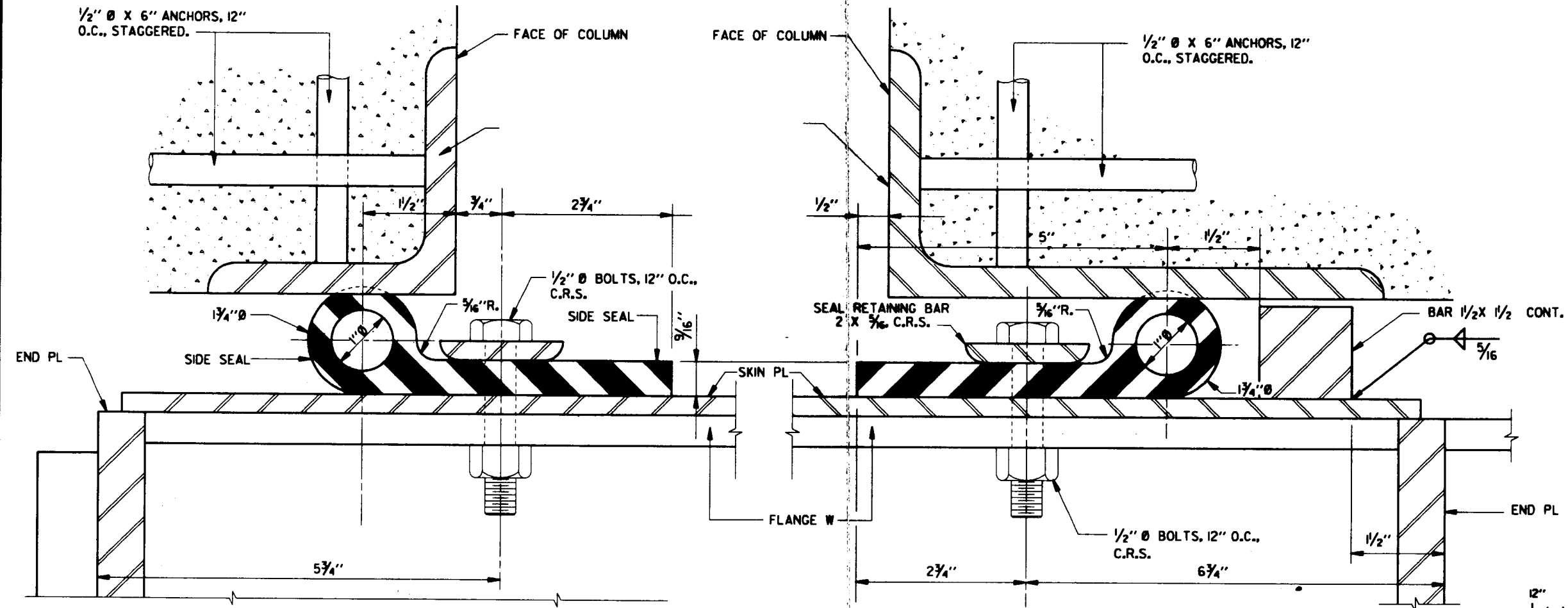
DETAIL 1 SCALE: FULL SIZE
