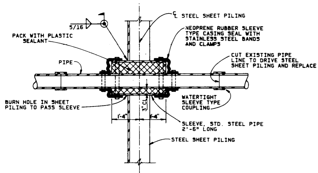
SECTION A TYPICAL PIPE THRU STEEL SHEET PILING SCALE: 3/4" = 1'-0"
