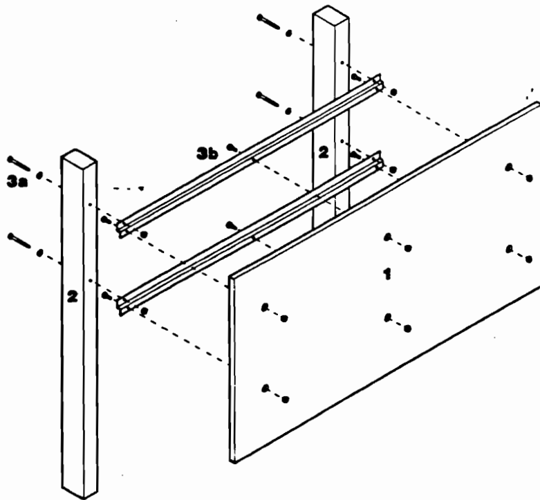
Exploded View
