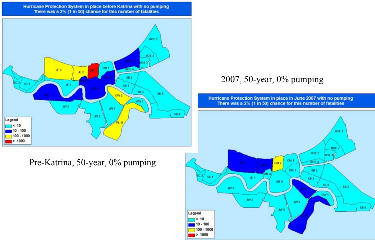
Figure 55. Loss of life risk maps comparing pre-Katrina HPS and 2007 HPS for 50-year (2%) flood frequency, no pumping.
