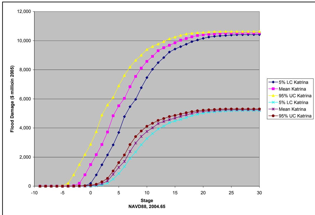
Figure 30. Comparison of flood damage – water level (in feet) relationships for pre- and post-Katrina scenarios for Orleans sub-basin 5. LC and UC represent the lower and upper confidence limits of the data.
