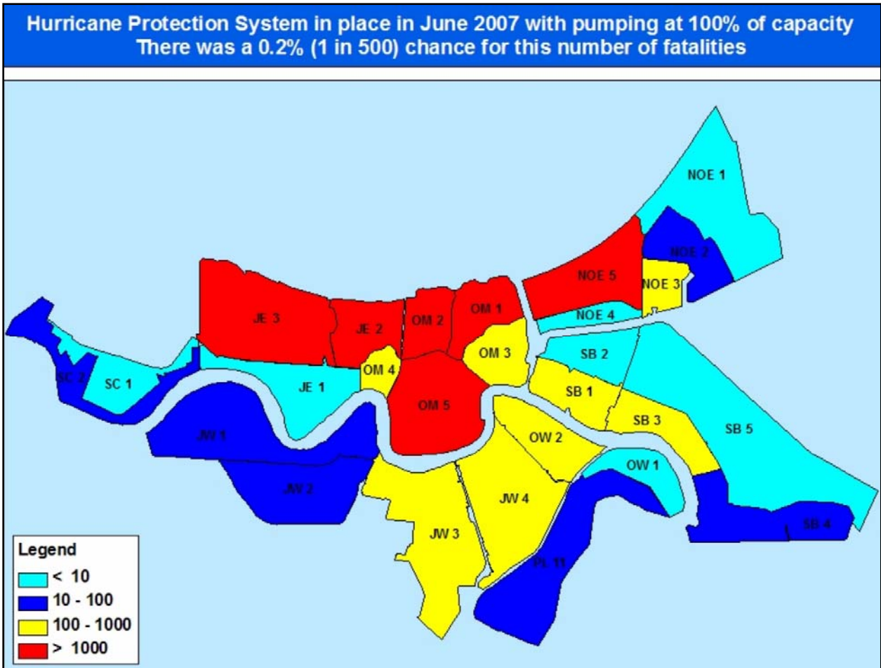
Figure 11-18. Loss of life risk map, 0.2% (1/500 return period) for June 2007 HPS and 100% pumping.
