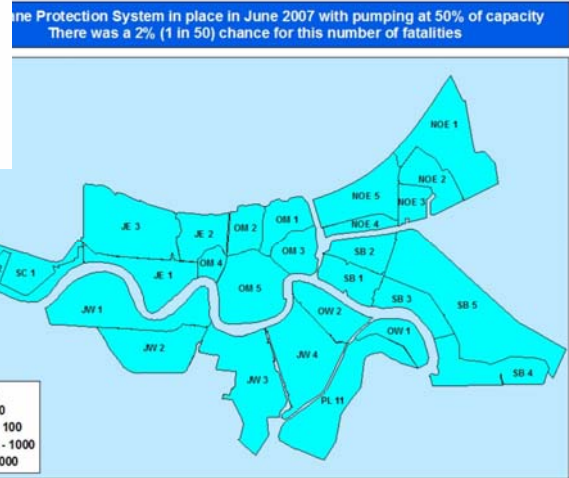
2007, 50-year, 50% pumping
