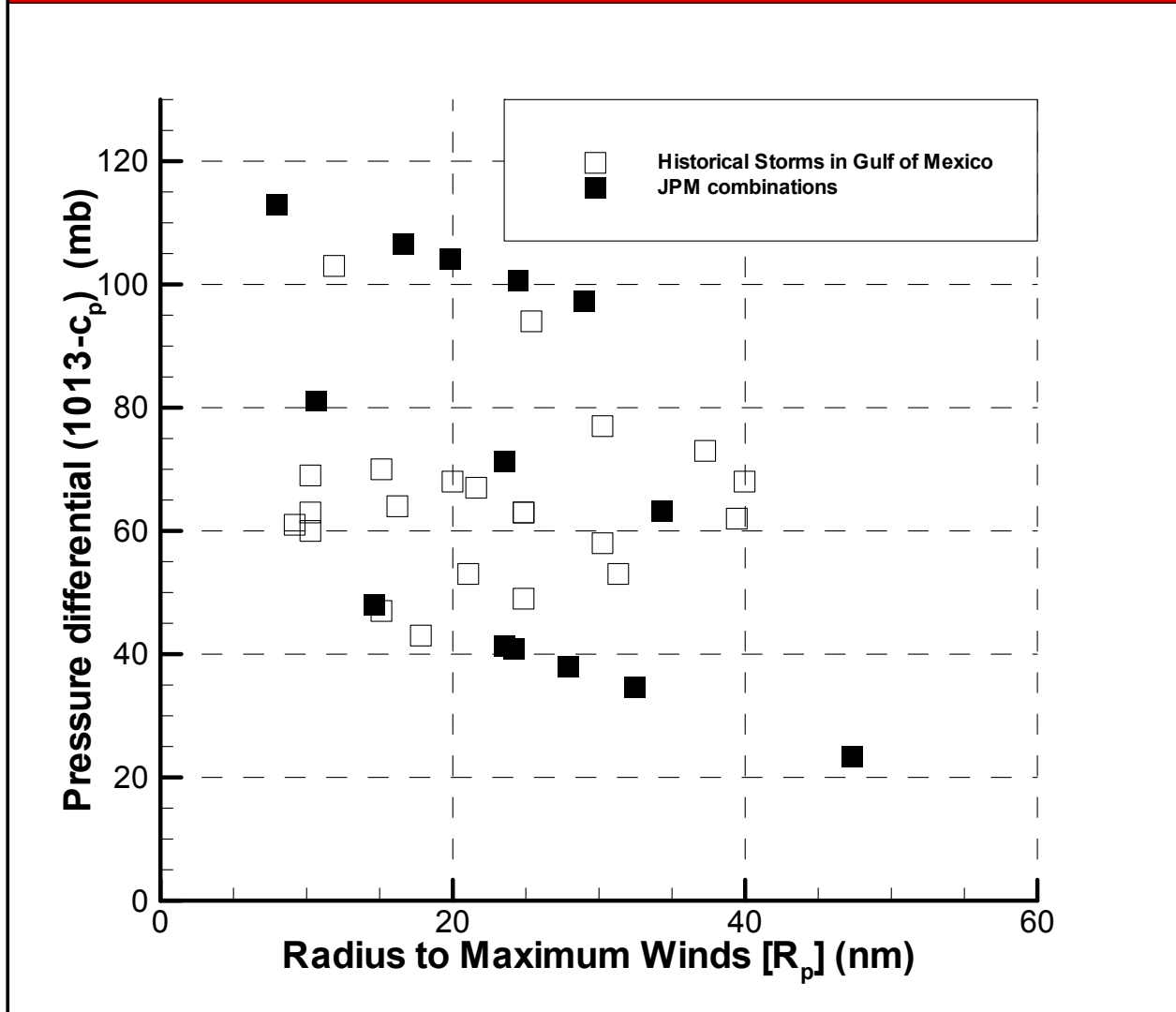
Figure 36. Plot comparing the pressure deficit-size combinations of historical and JPM-OS storms used to define the hazard for the risk assessment (Irish et al.).
