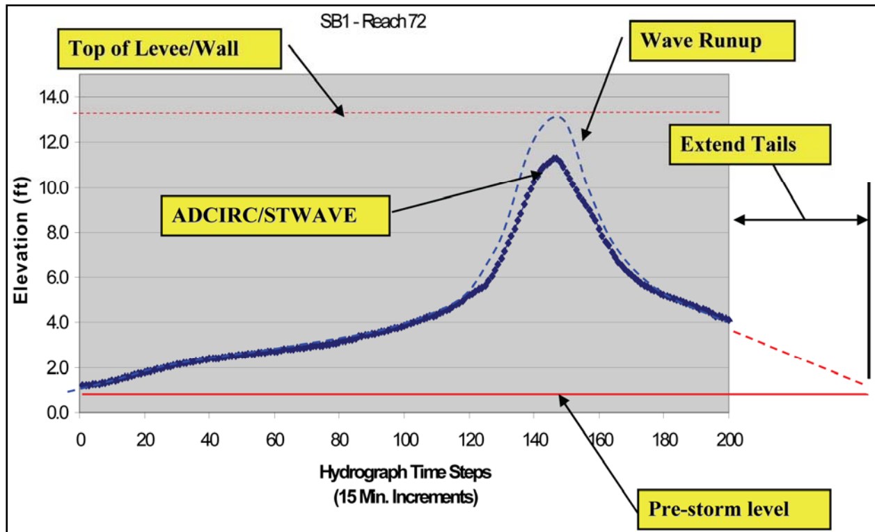
Figure 37. Illustration of storm hydrograph for a location. Graph shows specific process augmentation after ADCIRC/STWAVE simulation which includes wave setup.
