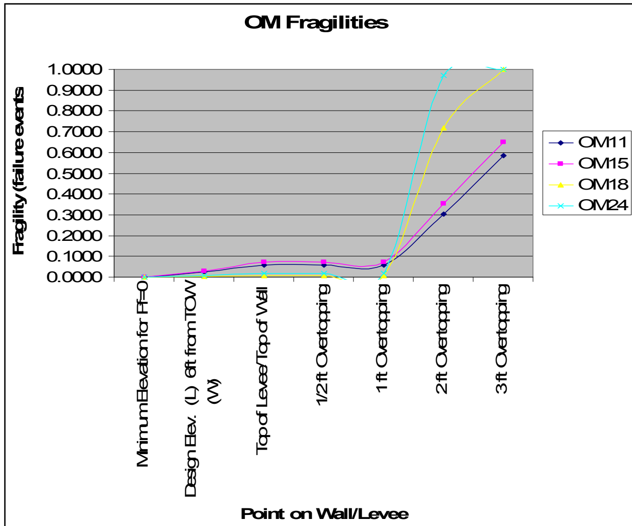
Figure 39. Fragility curves for a sample of reaches in the Orleans Main (OM) Basin. OM11 and 15 are along the south shore of Lake Pontchartrain, OM18 is on the west side of the IHNC, and OM24 is a portion of the Mississippi River main line levee.
