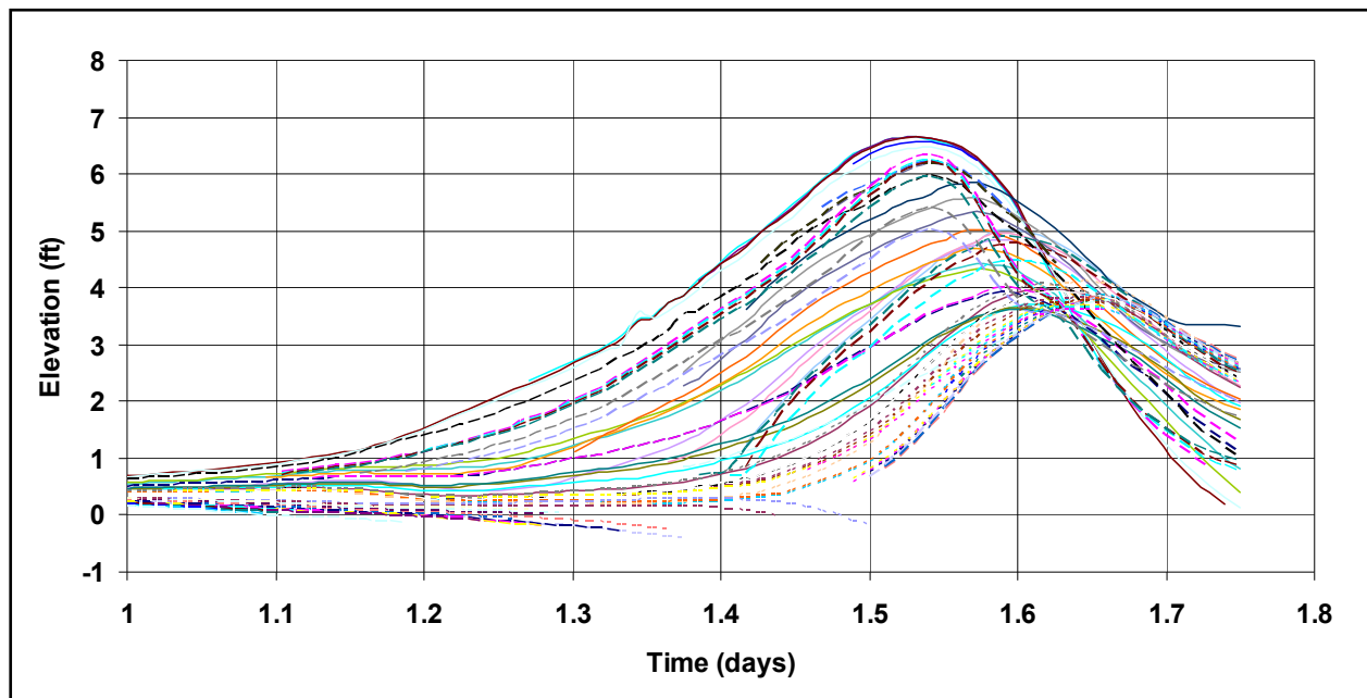
Figure 38. Example of hydrographs for a variety of locations around the HPS from a single storm.
