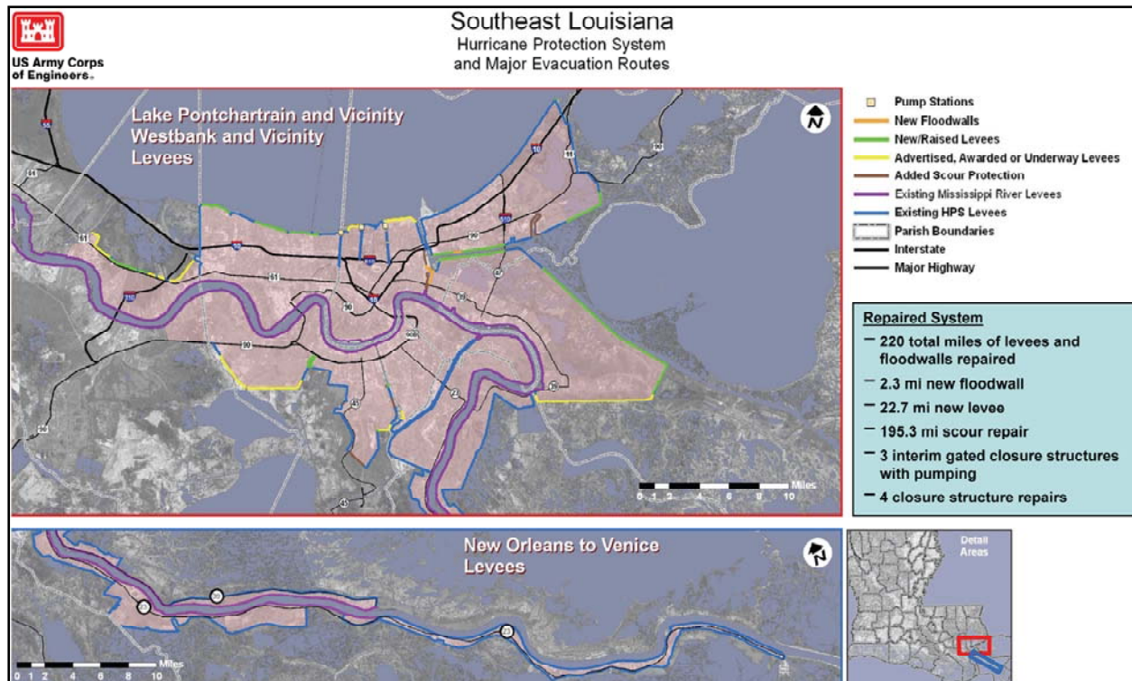
Figure 34. General configuration of 2007 HPS and list of major repairs and upgrades included in the 2007 HPS. Structures shown in yellow, indicating contracts pending for construction, were modeled in their existing June 2007 condition for this analysis. Source: U.S. Army Corps of Engineers.
