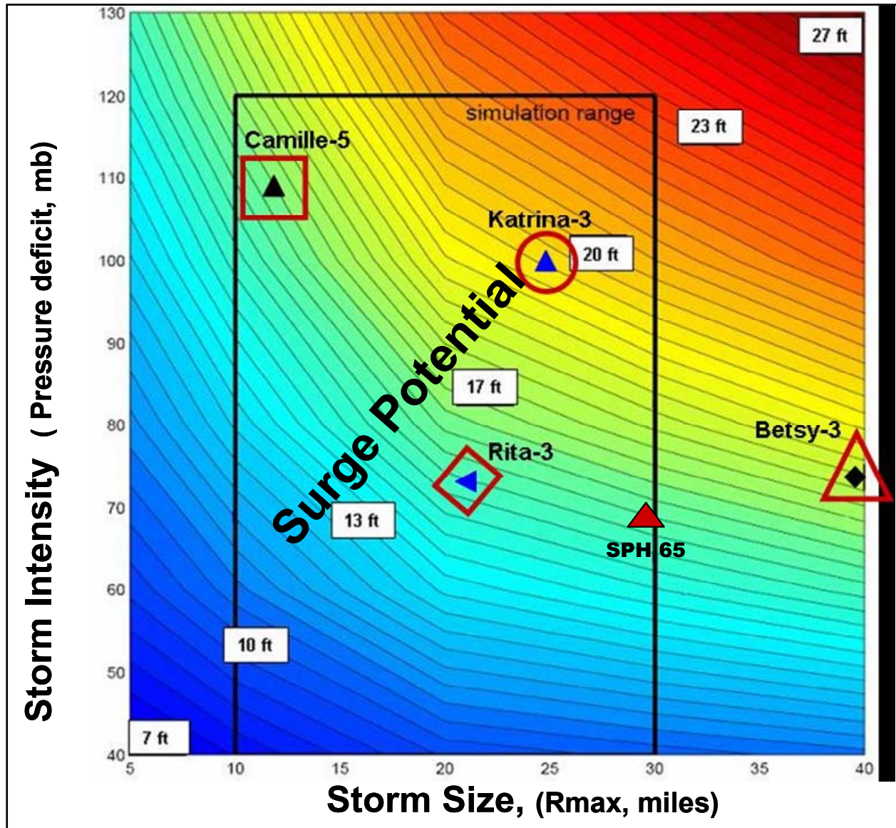
Figure 35. Relationship of intensity (central pressure deficit) to size of historical storms including their Saffir-Simpson category at landfall. Assumes simple straight-line shoreline with a 1:1000 ocean bottom slope (Irish et al.). As such, the surge values here are not necessarily those that particular storms produced for the complex shoreline and subsurface geometries of Mississippi and Louisiana.
