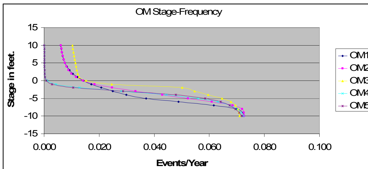
Figure 42. Example of water elevation – frequency of occurrence (exceedence) relationships for OM sub-basins. These curves do not include the impact of flow of water between sub-basins by natural drainage which is considered separately.
