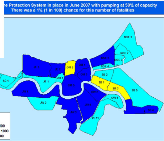
Figure 59. Loss of life risk maps comparing pre-Katrina HPS and 2007 HPS for 100-year (1%) flood frequency, 50% pumping.
