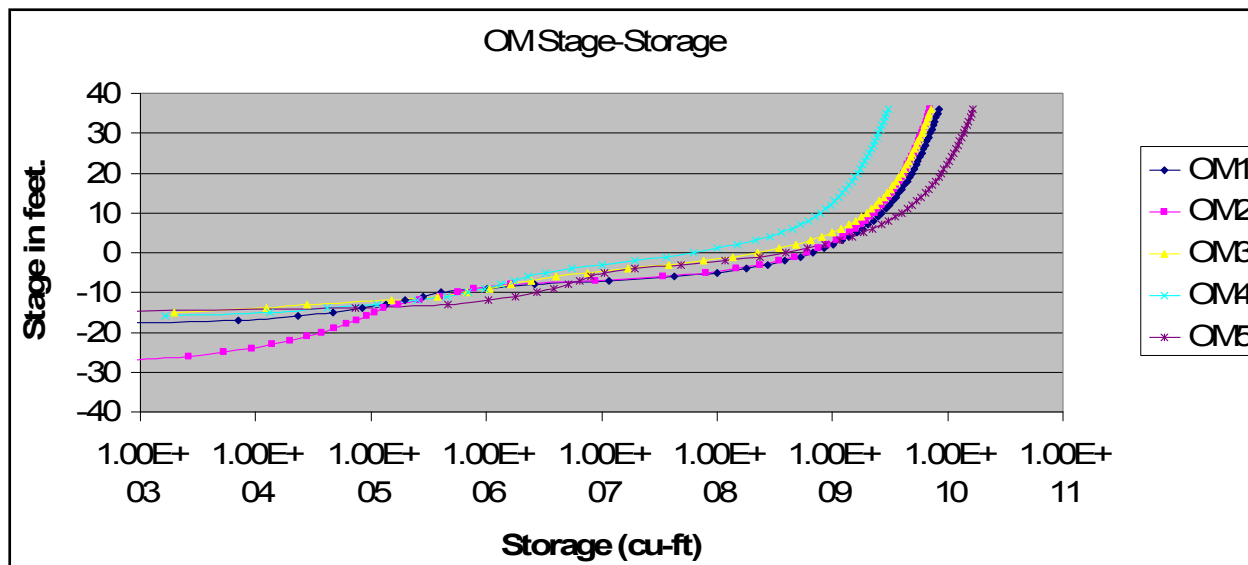
Figure 41. Example of relationship between the volume of water in a sub-basin (storage) and the resulting water elevation for OM sub-basins.
