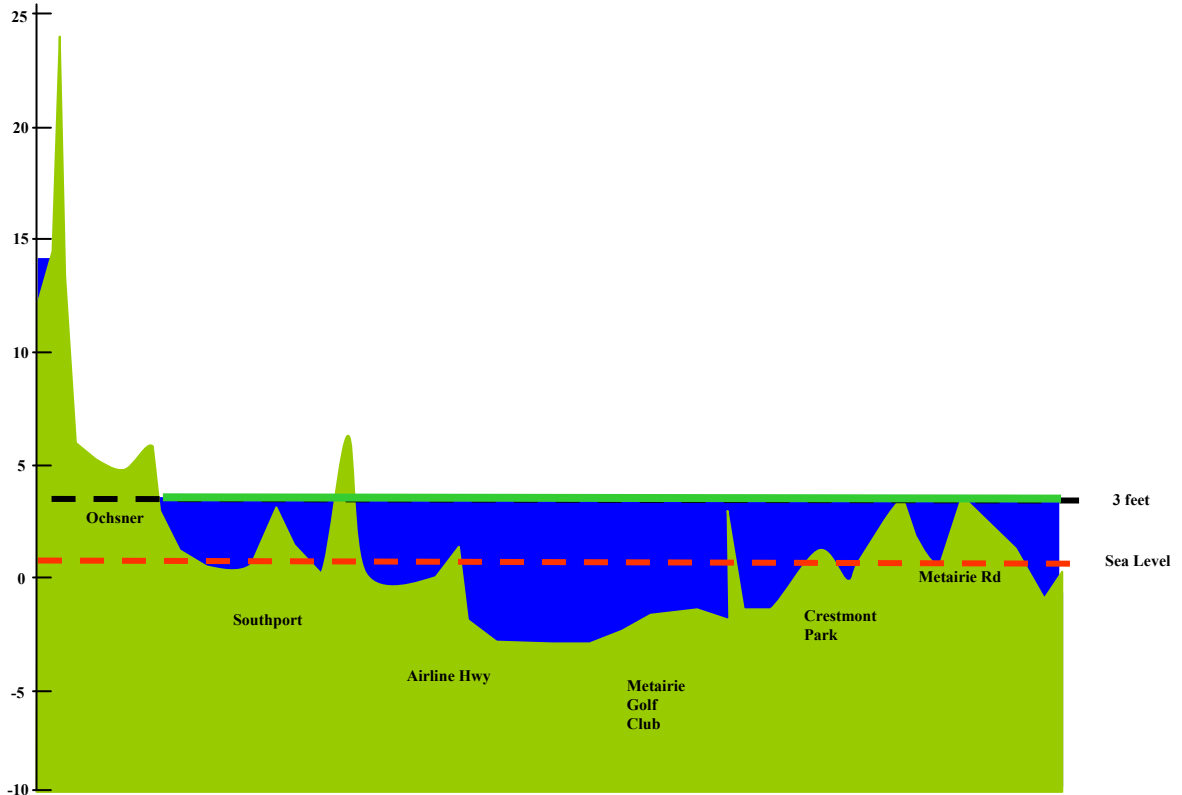
Figure 50. Flood depth information desired by local officials to better understand and communicate vulnerability.
