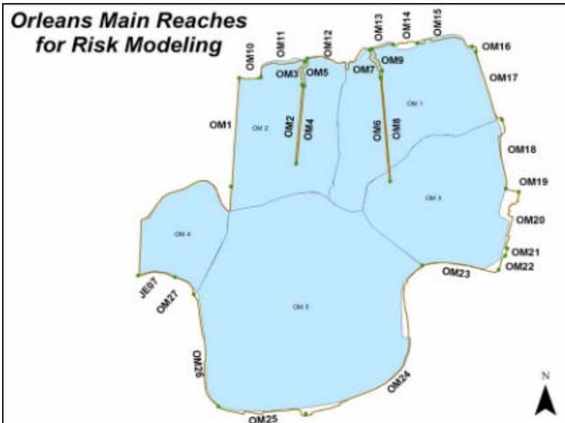
Figure 33b. Definition of reaches for Orleans Main Basin risk assessment. Reach definitions for all basins and sub-basins are given in IPET Volume VIII.
