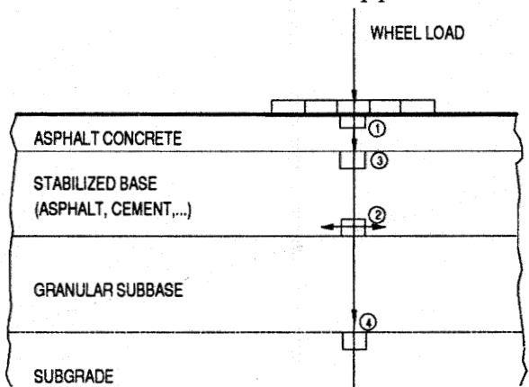
TYPICAL FLEXIBLE PAVEMENT WITH STABILIZED BASE
