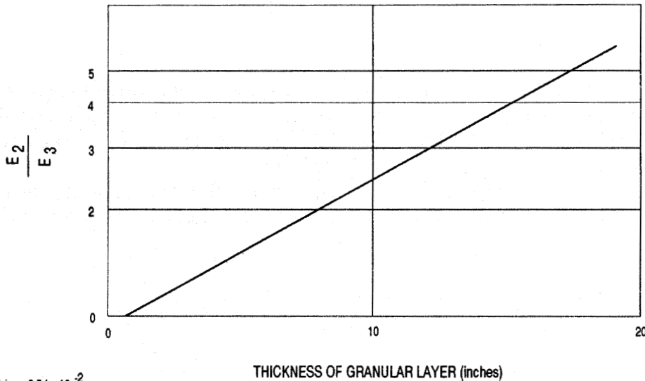
Figure 38. Relation of modular ratio to granular base thickness. (55)
