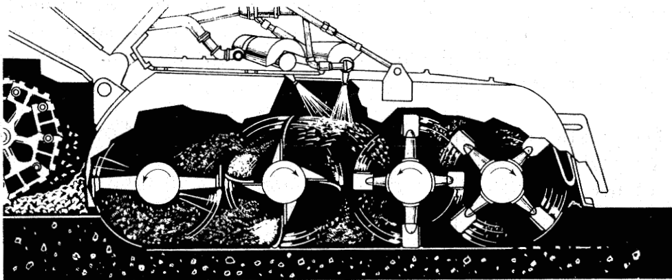
Figure 15. Multiple-shaft rotary mixer. (37)
