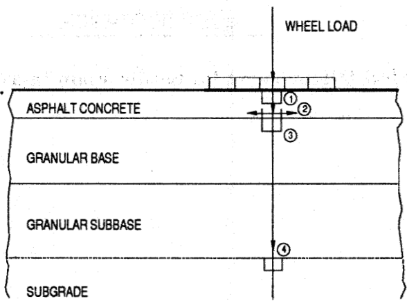
TYPICAL FLEXIBLE PAVEMENT WITH GRANULAR BASE
