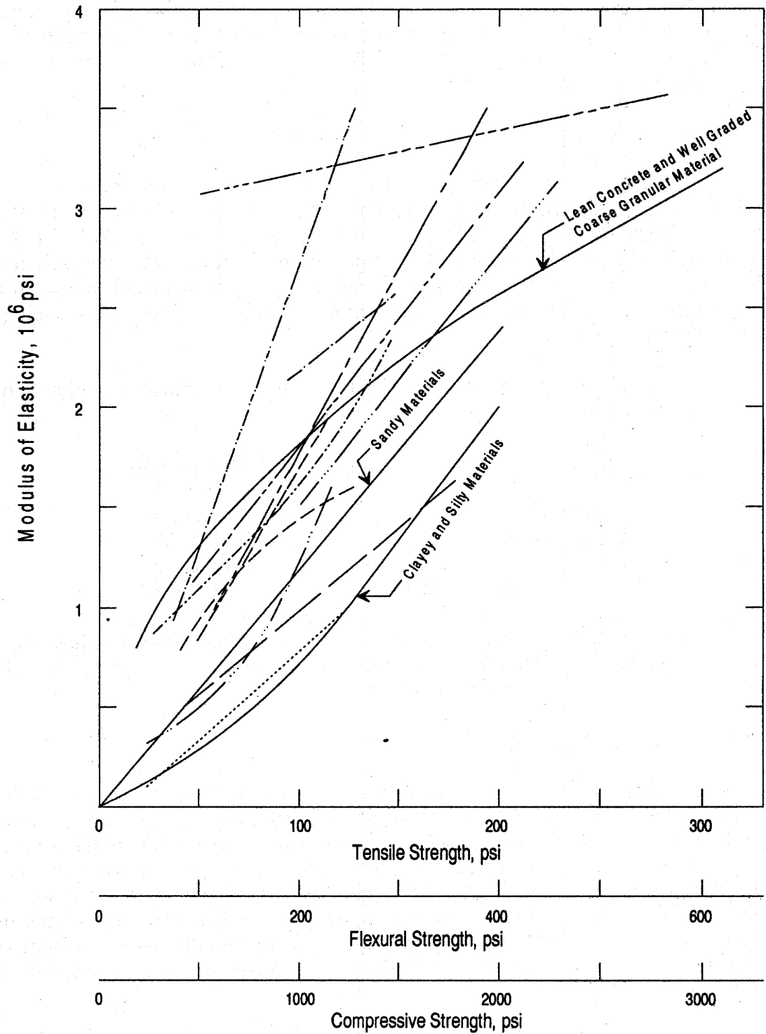
Figure 49. Recommended modulus-strength relations superimposed on reported relations. (69)
