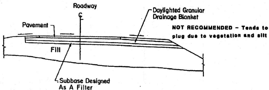
Figure 5. Drainage blanket.
