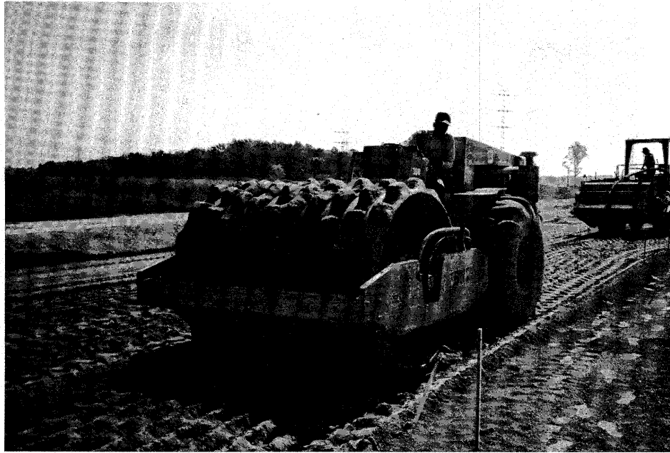
Figure 19. Vibratory sheepfoot roller.
