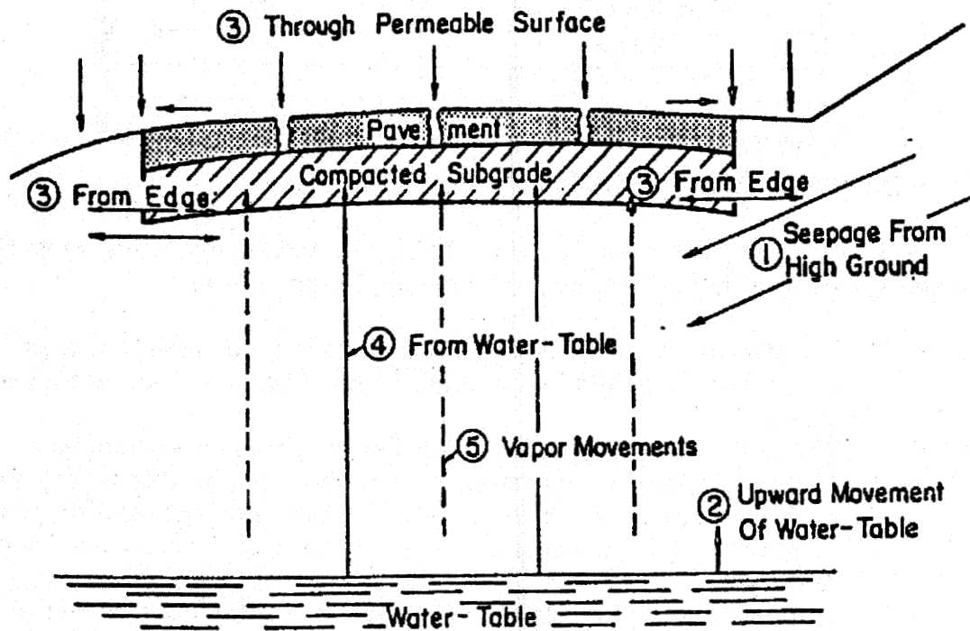
Figure 2. Sources of moisture in pavement systems.
