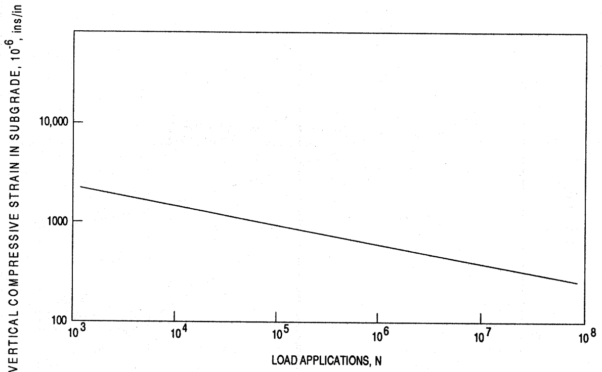
Figure 35. Typical fatigue curve for permanent deformation in a silty-clay subgrade. (53)
