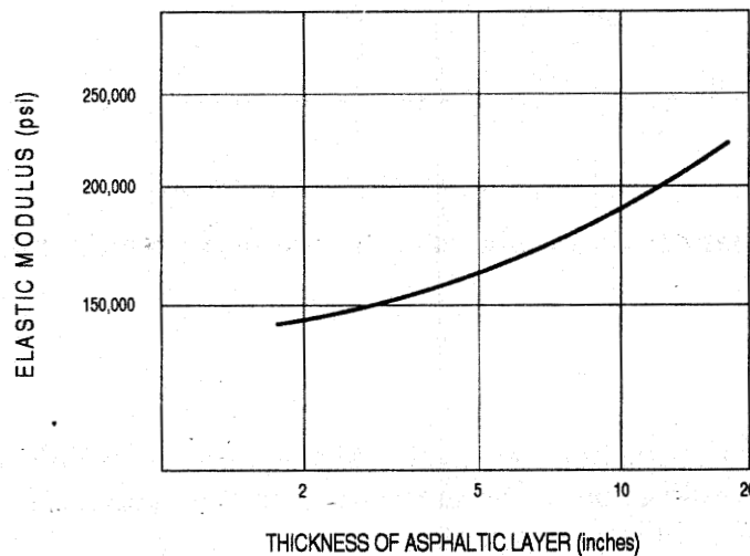
1 psi = 6.89 \times 10^{-2} Pa 1 in. = 2.54 \times 10^{-2} m 2 Figure 37. Relation of asphalt layer modulus to thickness of layer (air temperature of 95 °F [35 °C]). (55)
