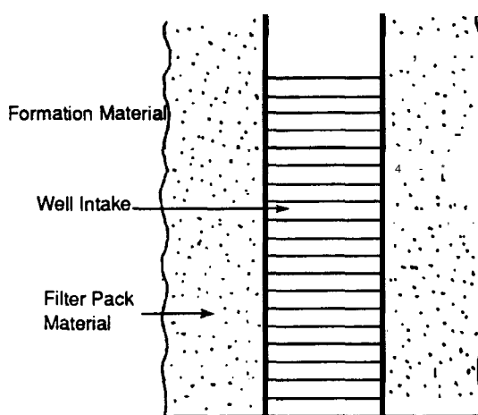
Figure 58. Envelope of coarse-grained material emplaced around an artificially filter-packed well.
