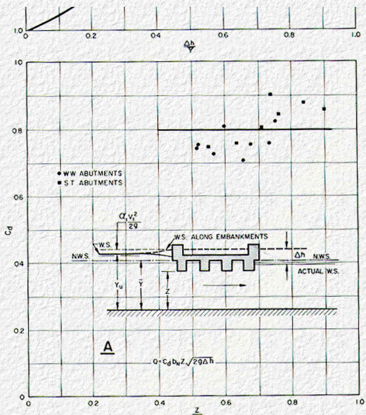
Figure 22. Discharge coefficient for all girders in flow (case II).
