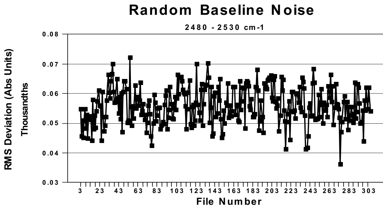
Figure 7. Random baseline noise measured between 2480 and 2530 cm -1 .
