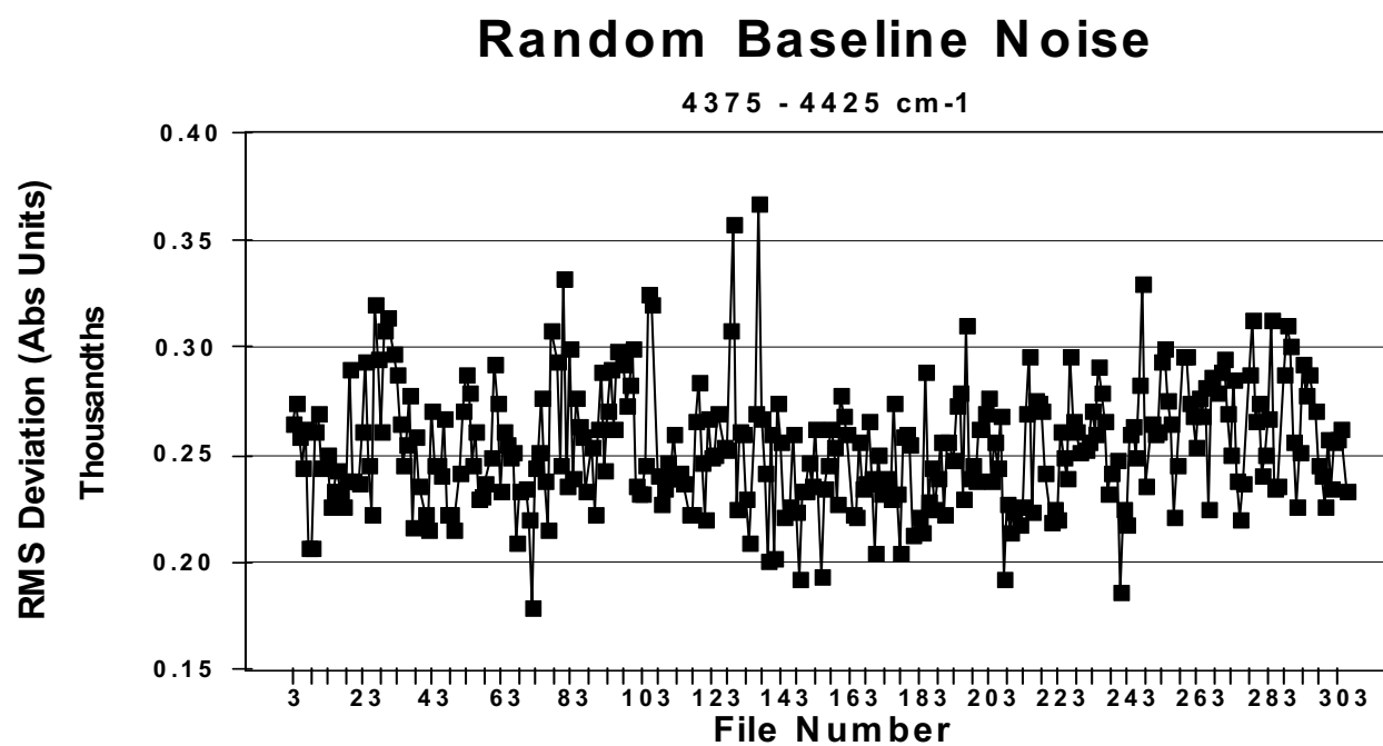
Figure 8. Random baseline noise measured between 4375 and 4425 cm -1 .
