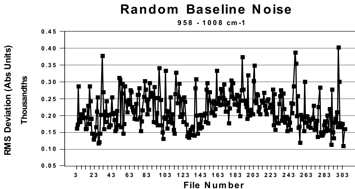
Figure 6. Random baseline noise measured between 958 and 1008\text{ cm}^{-1} .
