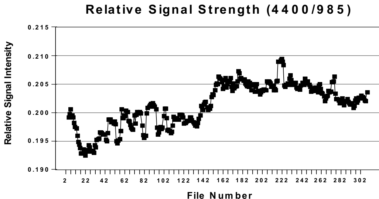
Figure 5. Relative single-beam signal intensity at 4400\text{ cm}^{-1} ratioed to that at 985\text{ cm}^{-1} .
