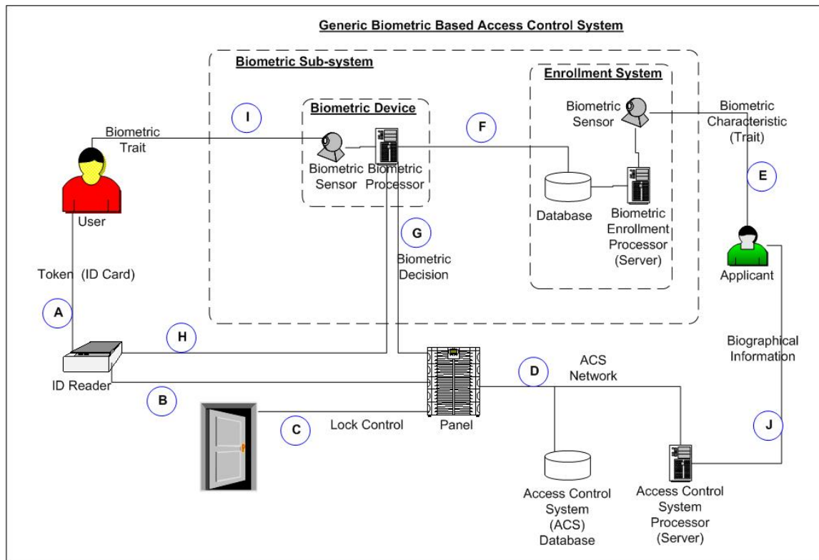
Figure 4.1 Generic Biometric-based Access Control System (ACS)
