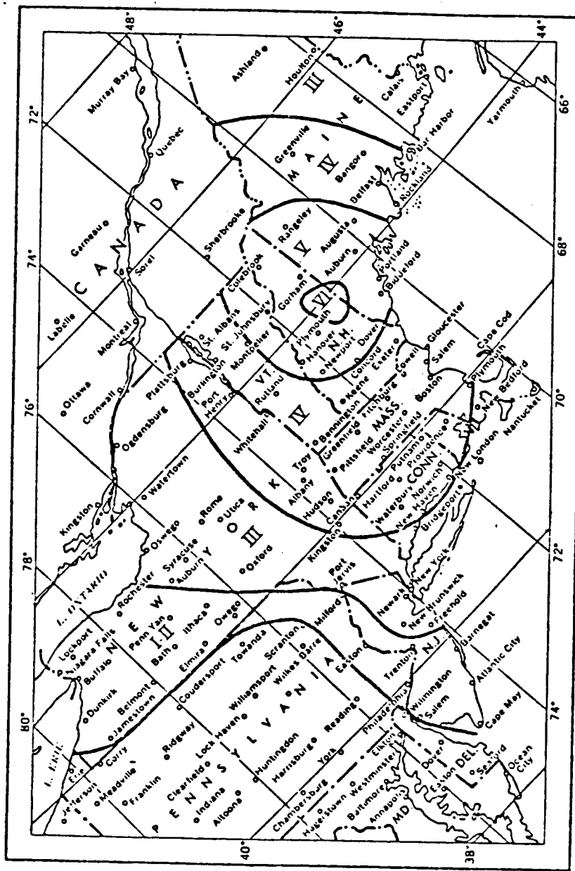
FIGURE 4.—Isoseismals of the New Hampshire earthquakes of December 20 and 24, based on investigations of Northeastern Seismological Association.
