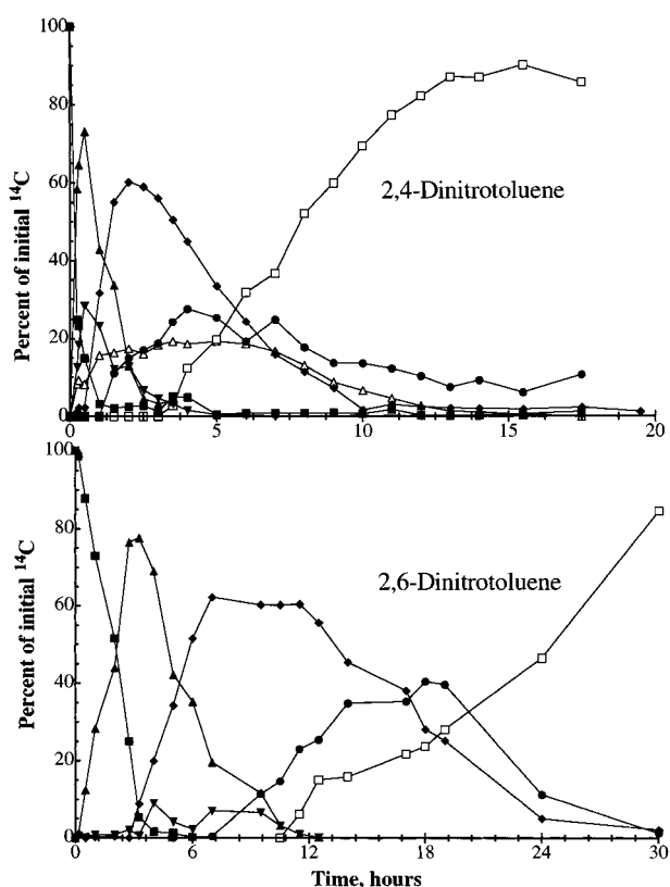
FIGURE 2. Temporal concentrations of identifiable compounds during the transformation of 2,4-dinitrotoluene (top) and 2,6-dinitrotoluene (bottom) in cell extracts of C. acetobutylicum . Symbols in the top figure denote percent of 14 C present as 2,4-dinitrotoluene (■), hydroxylaminonitrotoluenes (▲), 4-amino-2-nitrotoluene (▼), 2,4-dihydroxylaminotoluene (◆), aminohydroxylaminotoluene (●), 2,4-diaminotoluene (□), and an unknown (△). Symbols in the bottom figure denote percent of 14 C present as 2,6-dinitrotoluene (■), 2-hydroxylamino-6-nitrotoluene (▲), 2-amino-6-nitrotoluene (▼), 2,6-dihydroxylaminotoluene (◆), 2-amino-6-hydroxylaminotoluene (●), and 2,6-diaminotoluene (□).
