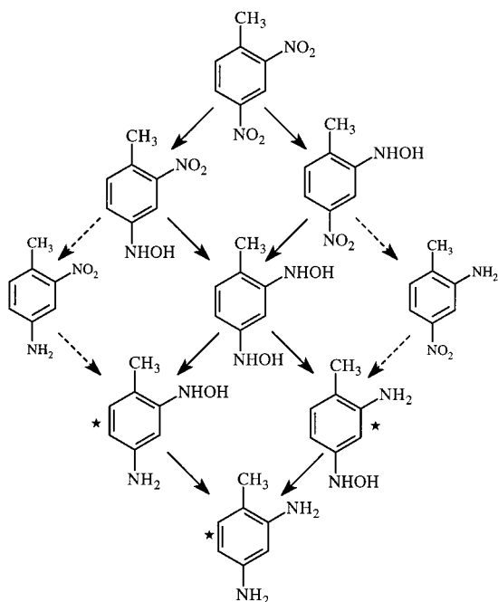
FIGURE 3. Observed transformation pathway for the transformation of 2,4-dinitrotoluene in cell culture and cell extracts. Dashed arrows represent minor pathways. The symbol ★ is placed by compounds observed only in extract systems.
