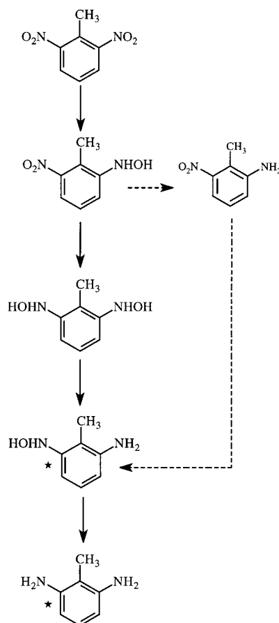
FIGURE 4. Observed transformation pathway for the transformation of 2,6-dinitrotoluene in cell culture and cell extracts. Dashed arrows represent minor pathways. The symbol ★ is placed by compounds observed only in extract systems.
