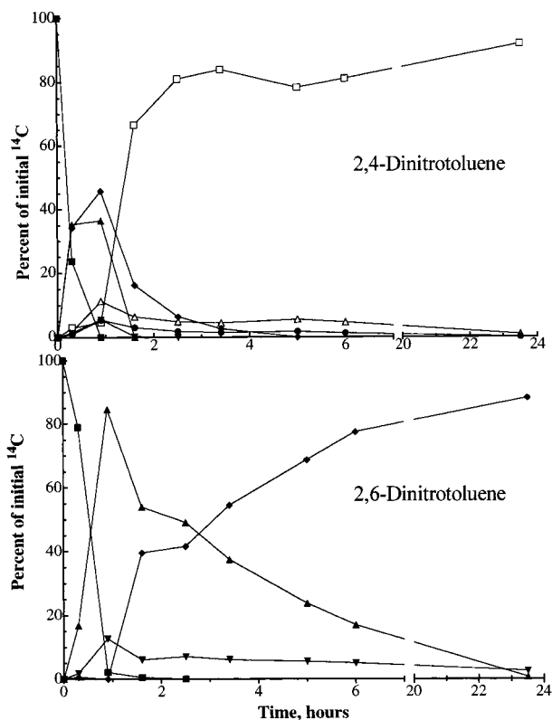
FIGURE 1. Temporal concentrations of metabolites during the transformation of 2,4-dinitrotoluene (top) and 2,6-dinitrotoluene (bottom) in cell cultures of C. acetobutylicum . Symbols in the top figure denote percent of ^{14}\text{C} present as 2,4-dinitrotoluene (■), 2-amino-4-nitrotoluene (▼), 4-amino-2-nitrotoluene (●), metabolite A_{24\text{DNT}} (▲), metabolite B_{24\text{DNT}} (◆), metabolite C_{24\text{DNT}} (□), and metabolite D_{24\text{DNT}} (△). Symbols in the bottom figure denote percent of ^{14}\text{C} present as 2,6-dinitrotoluene (■), 2-amino-6-nitrotoluene (▼), metabolite A_{26\text{DNT}} (▲), and metabolite B_{26\text{DNT}} (◆).
