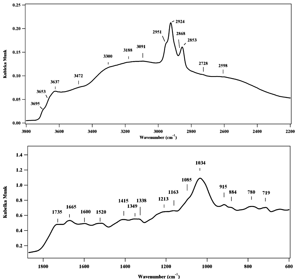
FIGURE 2. Diffuse reflectance FT-IR spectrum for Chelsea soil humic acid.
