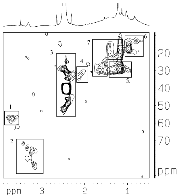
FIGURE 5. Region of the HMQC spectrum (in DMSO- d_6 ) of Chelsea soil humic acid with cross-peaks. Cross-peaks are consistent with the following assignments: 1. aromatic methoxy, 2. hydroxylated carbon, 3. DMSO- d_6 solvent peak, 4. CH 2 adjacent to C=C or COOH, 5. straight chain CH 2 groups that are least two bonds removed from electron withdrawing functionalities such as oxygen, 6. CH 3 groups, and 7. various aliphatic groups that are consistent with CH 2 adjacent to hydroxylated carbon or once removed from double bonds, carboxylic acids or amino side chain carbons.
