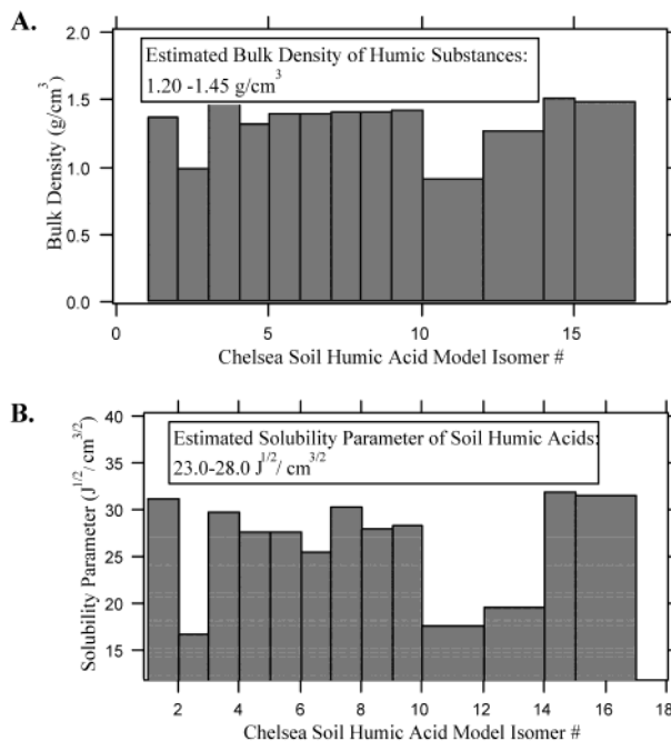
FIGURE 8. Calculated bulk densities (A) and solubility parameters (B) of the SIGNATURE generated 3-D models for Chelsea soil humic acid.
