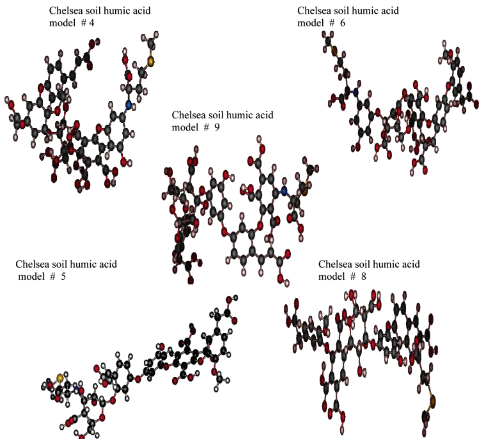
FIGURE 10. 3-D structures and bulk densities ( \rho ) and solubility parameters ( \delta ) of the selected SIGNATURE generated model isomers for Chelsea humic acid (HA). C atoms are in black, O atoms are in red, N atoms are in blue, S atoms are in yellow, and the remaining atoms are H atoms.
