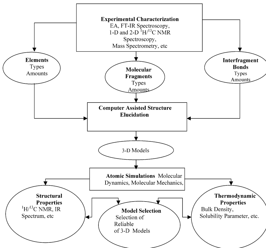
FIGURE 1. The hierarchical approach for modeling the 3-D structures of humic substances.
