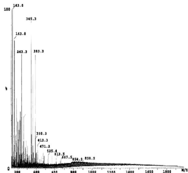
FIGURE 7. Electrospray ionization quadrupole time-of-flight (ESI QqToF) mass spectrum for Chelsea soil humic acid.
