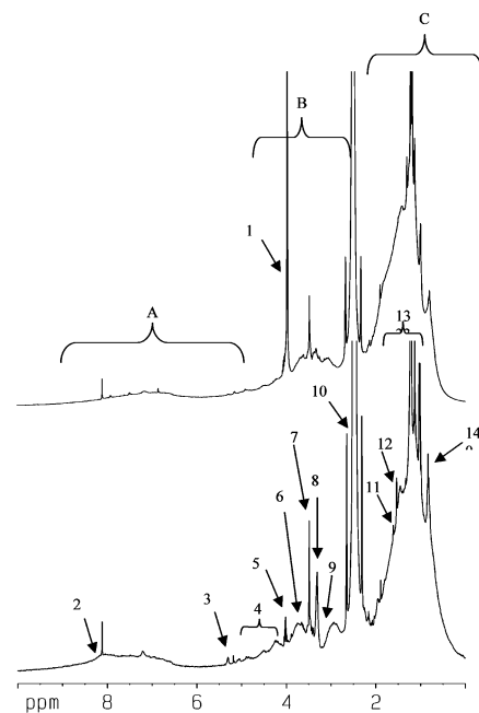
FIGURE 4. 1-D Solution ^1\text{H} NMR spectra for Chelsea soil humic acid at a concentration of 1 mg/mL, in \text{DMSO-}d_6 (top) and \text{DMSO-}d_6 with the addition of 100\ \mu\text{L} of \text{D}_2\text{O} (bottom). The major structural categories are labeled (top) as protons in aromatic and amides (A), sugars, amino acids, methoxy, aliphatic hydroxy (B) and aliphatic, amine protons (C). More detailed assignments are consistent with 1. \text{H}_2\text{O} at high concentration in \text{D}_2\text{O} (results from the addition of the \text{D}_2\text{O} ), 3. double bond protons, 4. protons in sugars or on the \alpha carbon of peptides/amino acids and lignin bridging units, 5. quartet multiplet, 6. broad "hump" from methoxy, sugar protons, or \alpha carbon of peptides/amino acids, 7. strong resonance likely to be from hydroxylated aliphatic carbon, 8. water in \text{DMSO} at low concentration, 9. distortion of baseline from presaturation pulse, 10. \text{DMSO-}d_6 , 11 and 12 exchangeable amine protons such as those in amino acids or terminal residues of peptides, 13 various methylene resonances and 14 methyl units.
