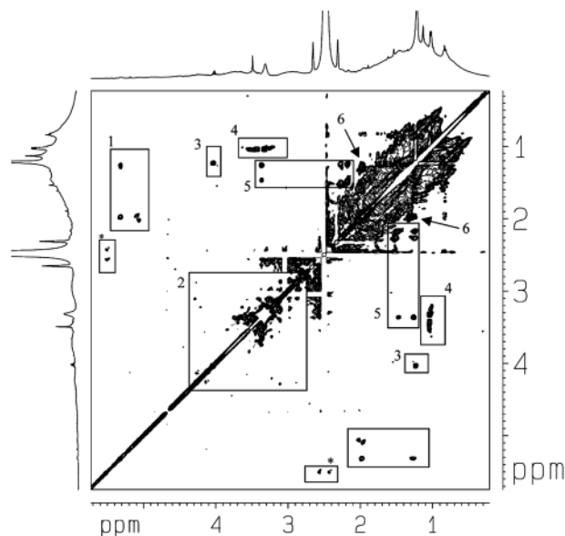
FIGURE 6. Expanded region of the TOCSY spectrum of Chelsea soil humic acid in DMSO- d_6 . * Represents an artifact resulting from the symmetrisation of the spectrum. The labels are consistent with the following assignments: 1. couplings from double bond protons to CH 2 protons in aliphatic chains, 2. couplings in sugar moieties, 3. \alpha - \beta couplings in alanine or possible in an acetyl structure, 4. couplings from hydroxylated aliphatic carbon to carbon in aliphatic chains -(CH_2)_nCOH(CH_2)_n- , 5. \alpha - \beta - \gamma couplings in amino acid residues, and 6. a strong coupling that is likely to result from aliphatic CH 2 groups once removed from a double bond (i.e., CH=CH-CH 2 -CH 2 ) or aliphatic acids components (HOOC-CH 2 -CH 2 -CH 2 ). The intense region from 1 to 2.5 ppm contains a multitude of partially resolved couplings that are difficult to observe in the printed spectrum. These are consistent with a distribution of couplings within a series of slightly different aliphatic compounds that may be variously substituted and branched.
