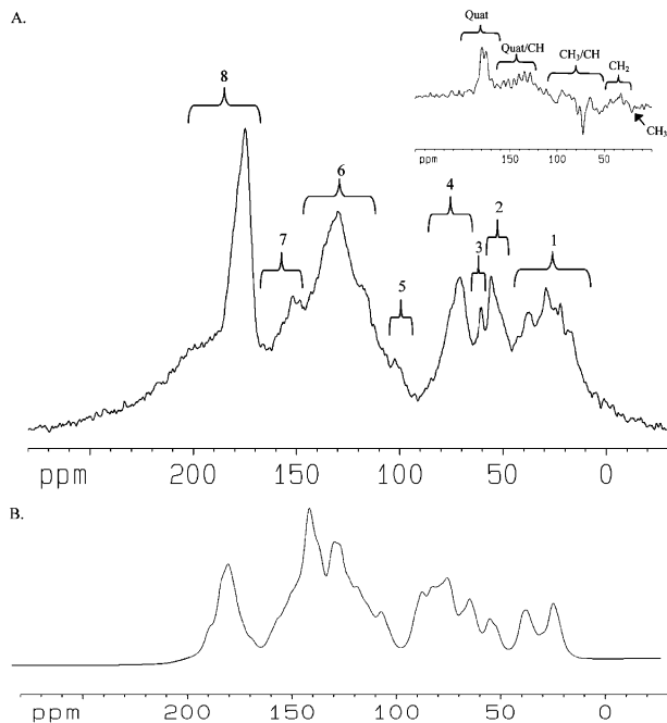
FIGURE 3. 1-D Solution ^{13}\text{C} NMR spectra for Chelsea soil humic acid. A. Measured carbon spectrum acquired under quantitative experimental conditions in \text{D}_2\text{O}/\text{NaOD} . The assignments are consistent with the following: 1. aliphatic, 2. methoxy, 3. \alpha carbon in amino acids and peptides, 4. sugars carbon, 5. anomeric sugar carbon, 6. aromatic carbon, 7. oxygen substituted aromatic carbon, and 8. carboxylic acid and carbonyl carbon. Assignments are confirmed by the PENDING edited carbon spectrum (insert) which is phased so that quaternary carbon point up, CH carbons point down, \text{CH}_2 carbon point up and \text{CH}_3 carbon point down. B. Simulated ^{13}\text{C} NMR spectrum of an equimolar mixture of the SIGNATURE generated Chelsea soil humic acid models from Figure 10.
