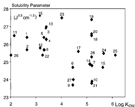
FIGURE 9. Solubility parameters for "humic organic matter" (HOM) estimated by Poerschman and Kopinke (62) from literature sorption data. The solubility parameter ( \delta ) is defined as the square root of the cohesive density (see eq 7) and thus is readily calculated from heat of vaporization and molar volume data. Because direct measurements of these thermodynamic properties for humic acids are not feasible in most cases, fitting measured organic normalized soil binding constants ( K_{oc} ) of hydrophobic organic compounds (HOCs) to a Flory-Huggins model has become the "standard" method for determining the solubility parameters of humic substances in the environmental science literature (62). The solubility parameters data shown in this figure were calculated by Poerschman and Kopinke (62) by fitting literature data of HOC sorption onto HOM to a Flory-Huggins model. They found their range of values to be "quite narrow" (i.e., 23.0–28.0 J 1/2 /cm 3/2 ). Reprinted with permission from Poerschman, J.; Kopinke, F. D. Environ. Sci. Technol. 2001, 35, 1142. Copyright 2001 American Chemical Society.
