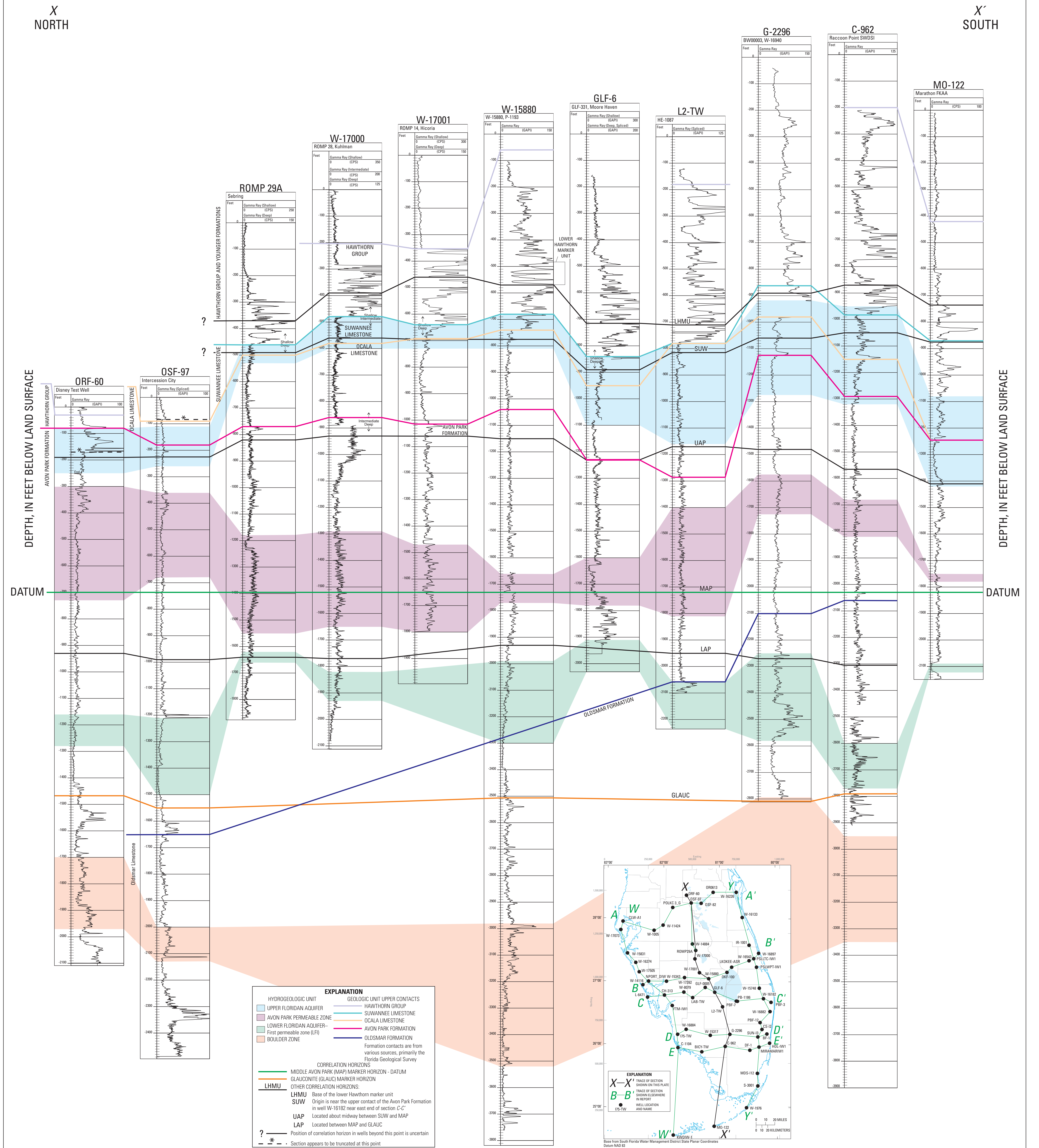
STRATIGRAPHIC SECTION X-X' By Ronald S. Reese and Emily Richardson 2007
