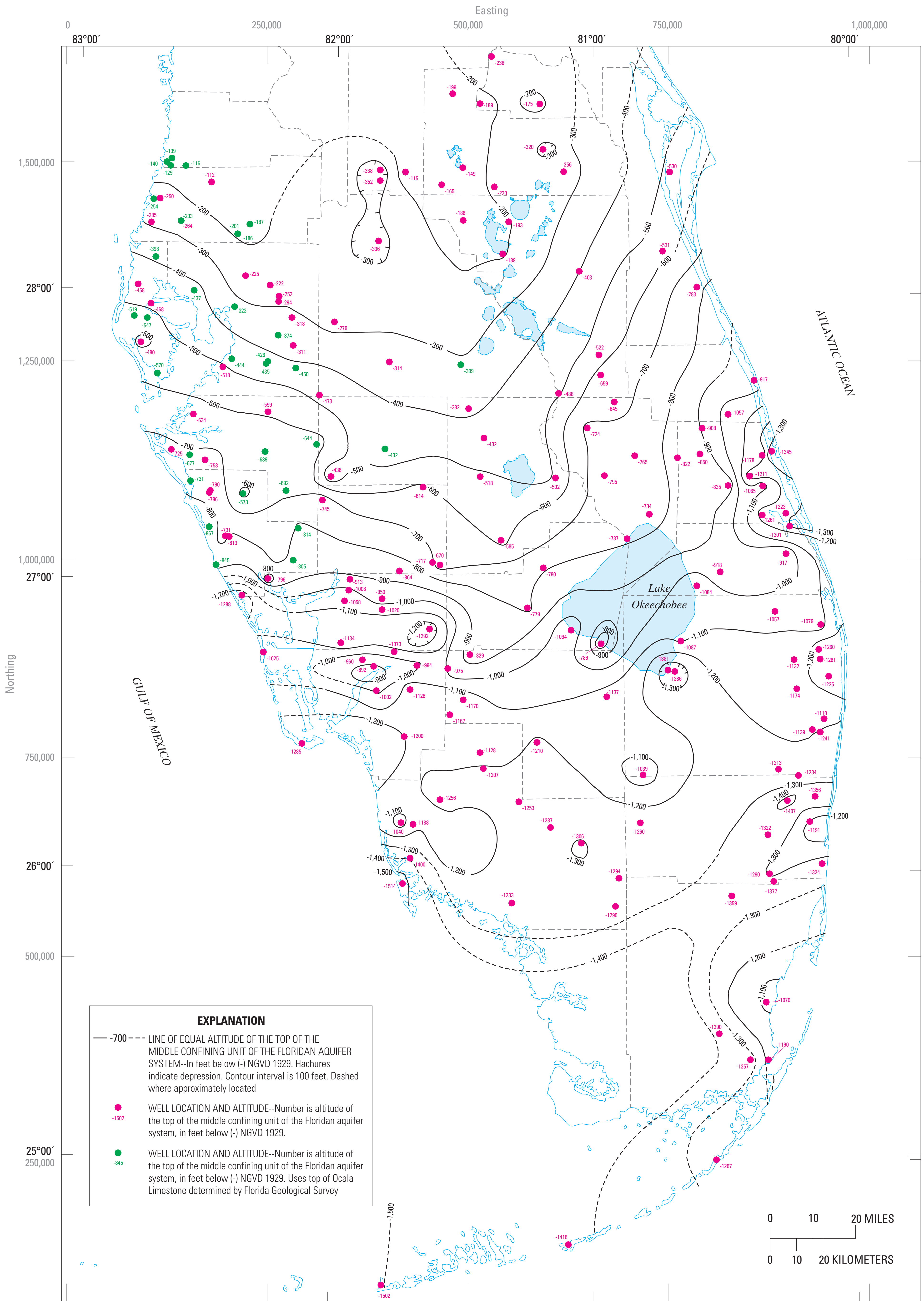
Figure A6. Altitude of the top of the middle confining unit (MCI) of the Floridan aquifer system.
