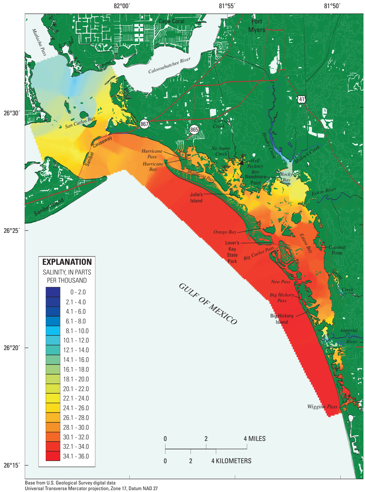
Figure 19f. Salinity patterns in Estero Bay, January 10, 2003.
