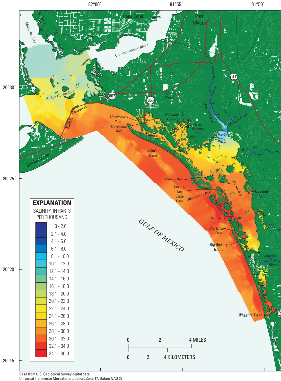
Figure 19b. Salinity patterns in Estero Bay, August 19, 2002.
