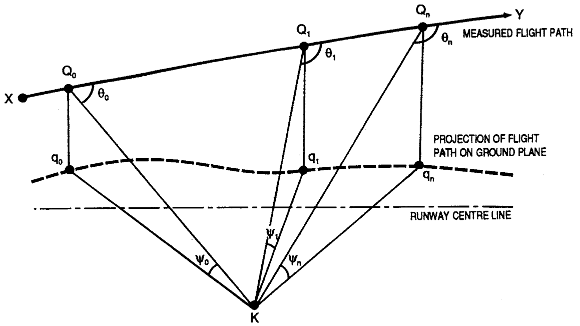
Figure A36-11(a). Measured flight path
