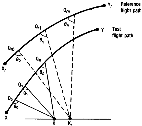
Figure A36-10. Correspondence between measured and reference flight paths for the application of the integrated method of adjustment
