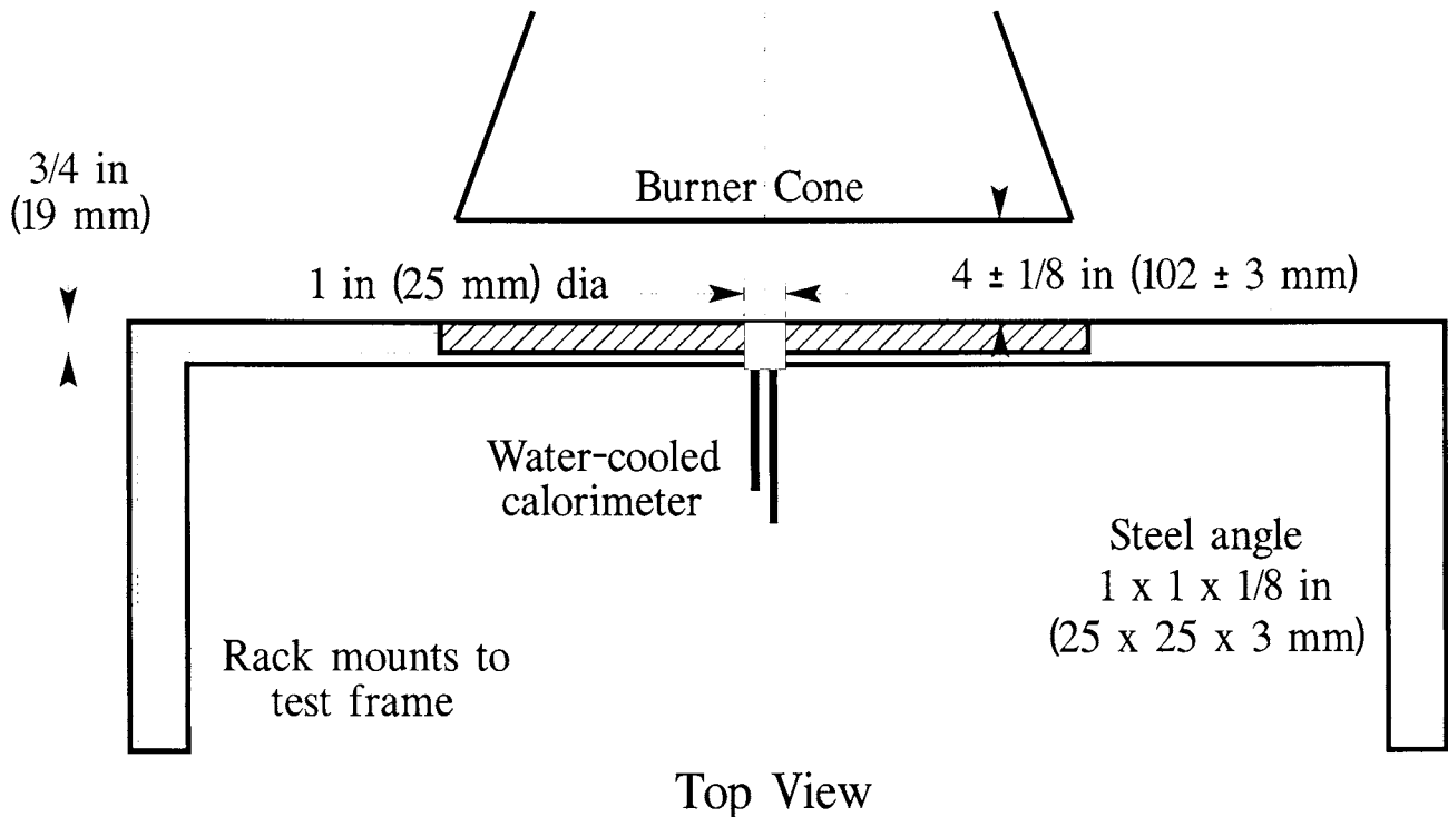
Figure 4 - Calorimeter Position Relative to Burner Cone
