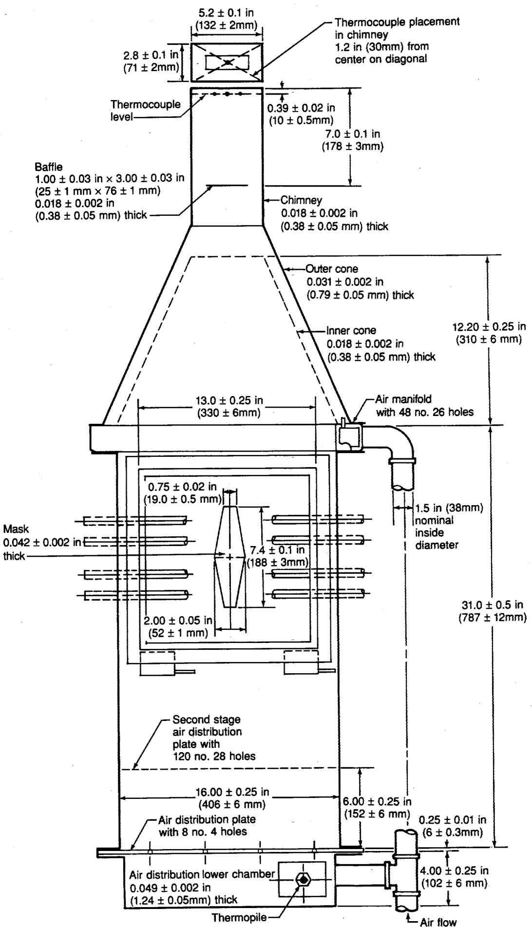
Figure 1A Rate of Heat Release Apparatus
