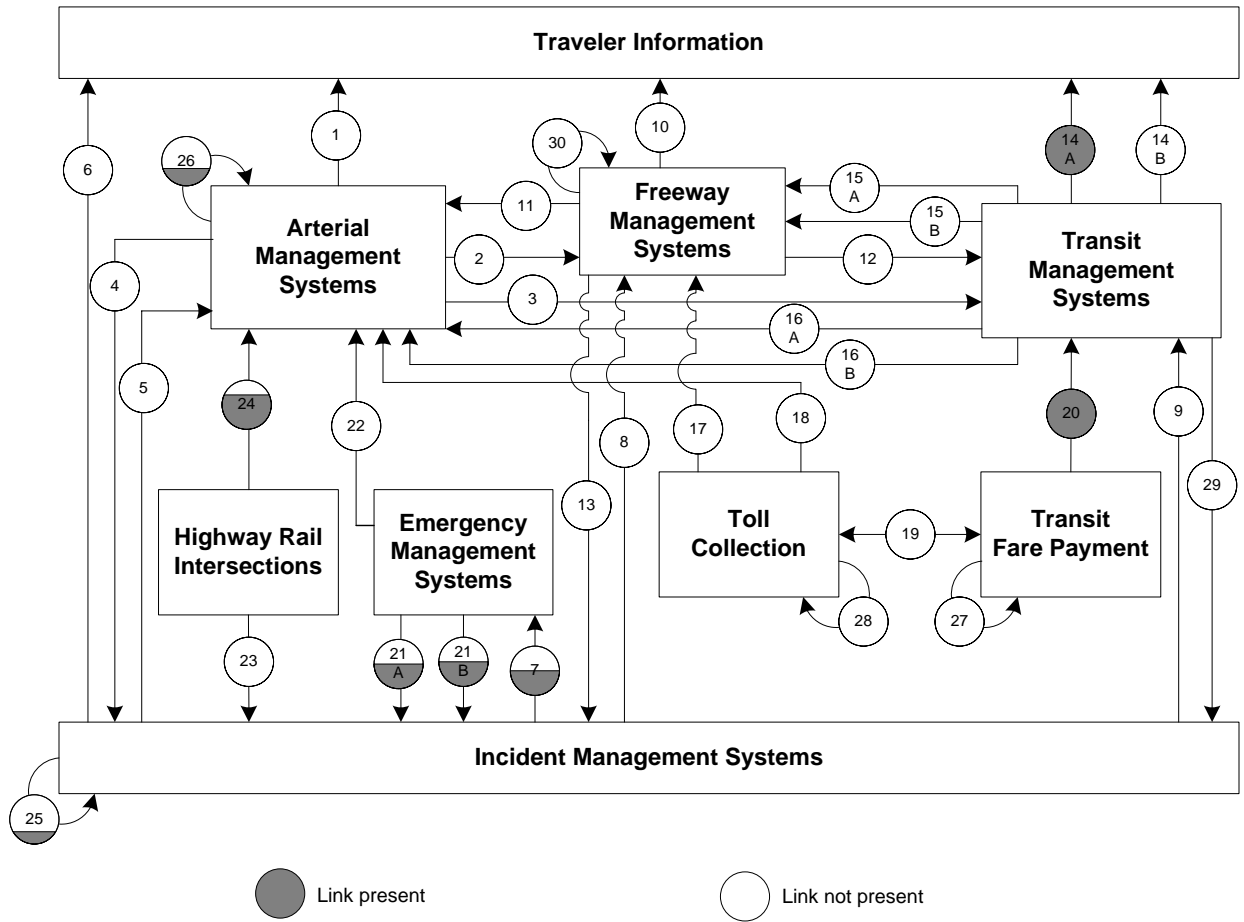
Figure 9 - Toledo Integration Links
