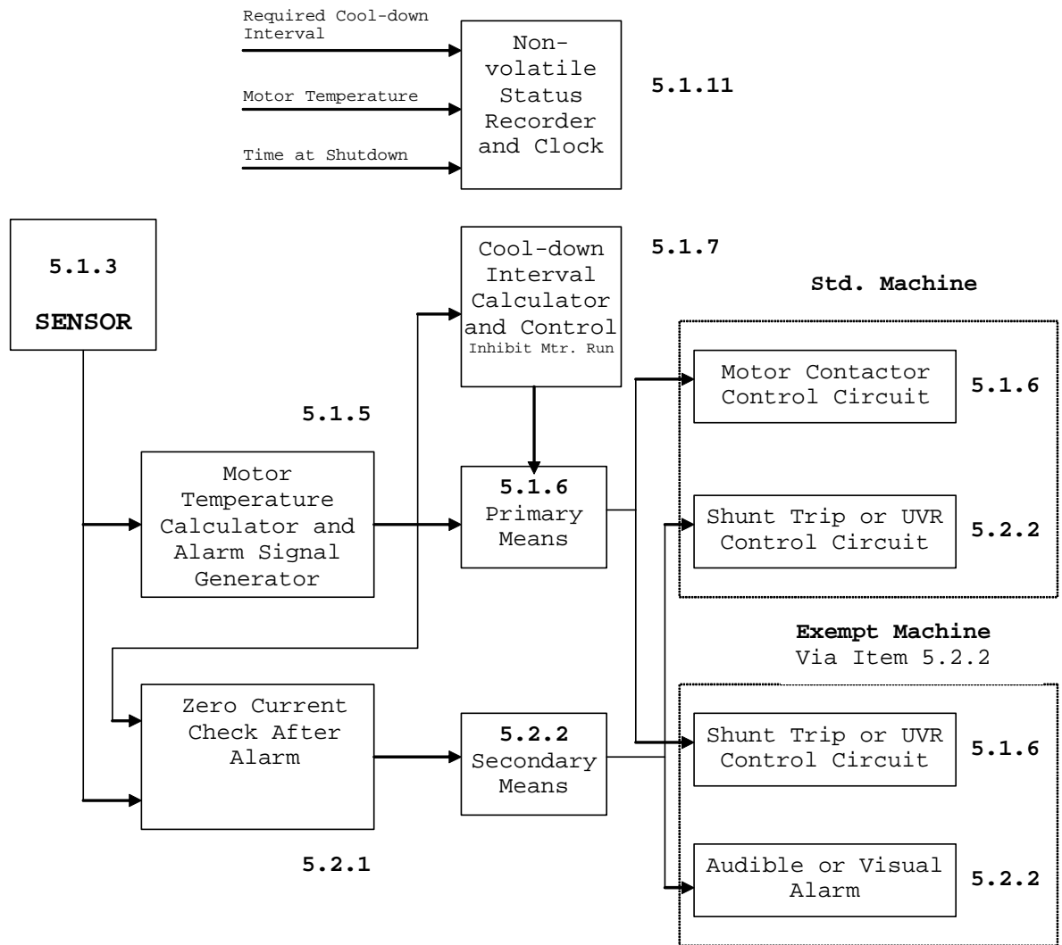
Microprocessor Based Motor Overload Protection System
